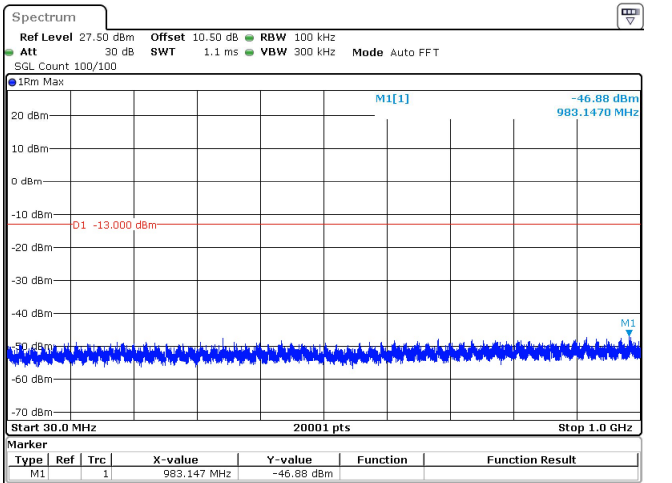
20MHz_15kHz_1745MHz_DFT-s-OFDM QPSK_RB1@105 -46.88 dBm
