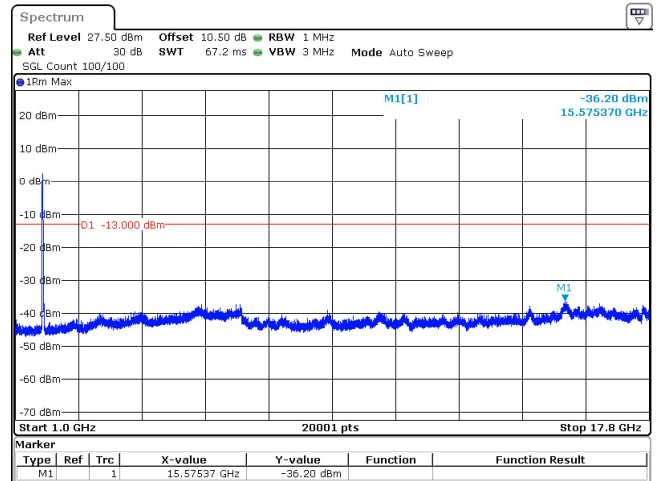
25MHz_15kHz_1722.5MHz_DFT-s-OFDM QPSK_RB128@0 -36.20 dBm
