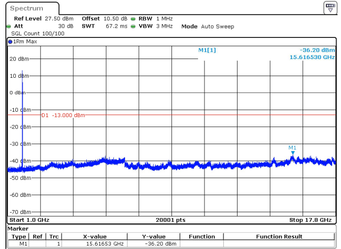
20MHz_15kHz_1745MHz_DFT-s-OFDM QPSK_RB1@105 -36.20 dBm
