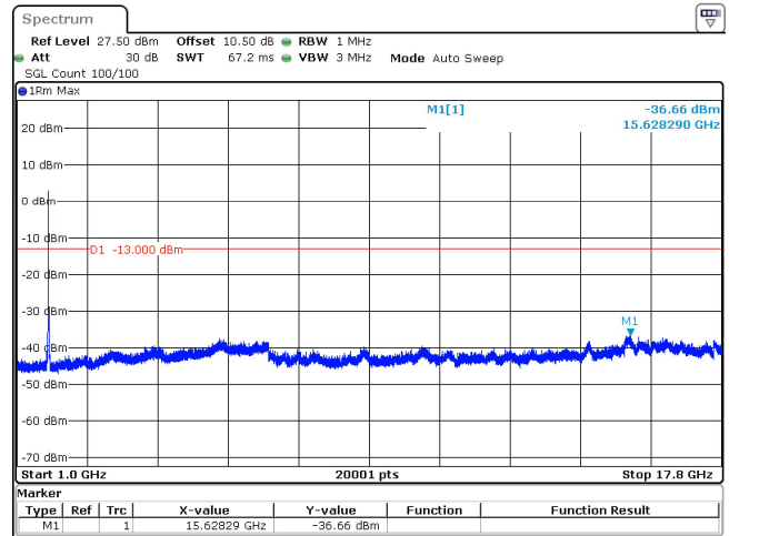
20MHz_15kHz_1745MHz_DFT-s-OFDM QPSK_RB100@0 -36.66 dBm
