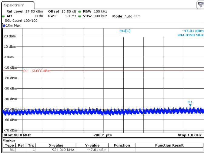
25MHz_15kHz_1722.5MHz_DFT-s-OFDM QPSK_RB1@0 -47.01 dBm
