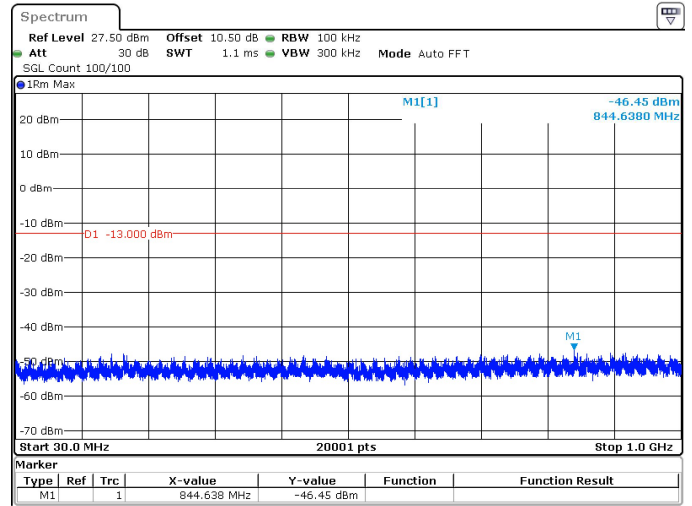
25MHz_15kHz_1722.5MHz_DFT-s-OFDM QPSK_RB1@132 -46.45 dBm
