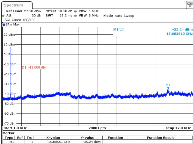
25MHz_15kHz_1722.5MHz_DFT-s-OFDM QPSK_RB1@132 -35.24 dBm
