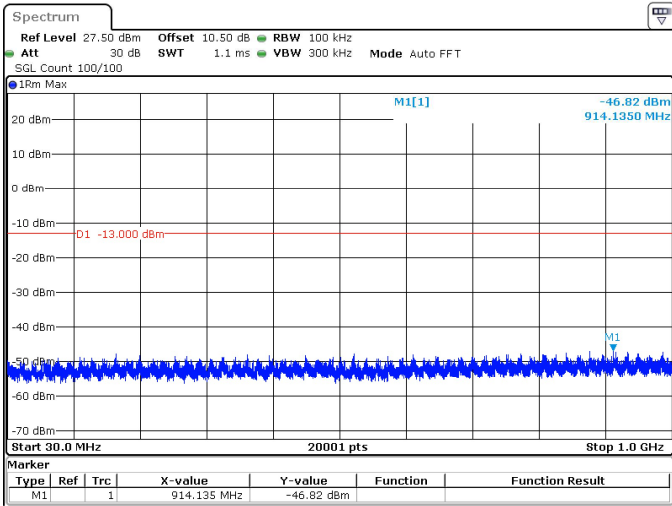
20MHz_15kHz_1745MHz_DFT-s-OFDM QPSK_RB100@0 -46.82 dBm
