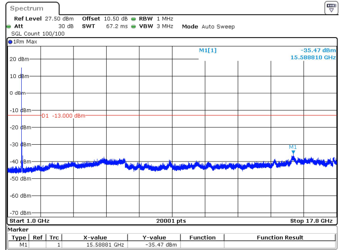
25MHz_15kHz_1722.5MHz_DFT-s-OFDM QPSK_RB1@0 -35.47 dBm
