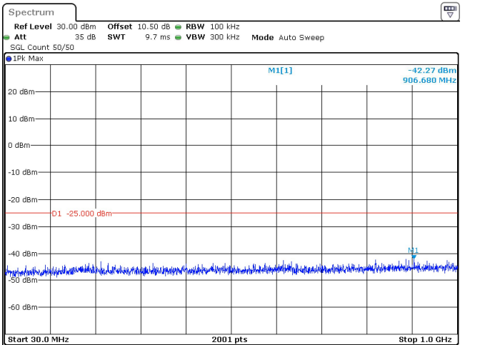
90MHz_30kHz_2592.99MHz_DFT-s-OFDM QPSK_RB1@244 -42.27 dBm
