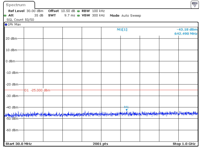
90MHz_30kHz_2592.99MHz_DFT-s-OFDM QPSK_RB1@0 -43.18 dBm
