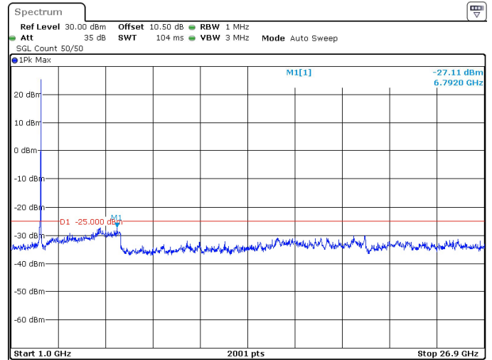
90MHz_30kHz_2592.99MHz_DFT-s-OFDM QPSK_RB1@244 -27.11 dBm
