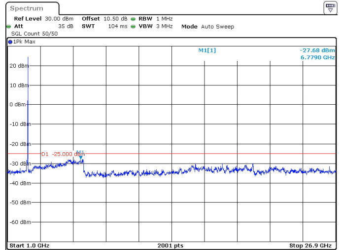
100MHz_30kHz_2546.01MHz_DFT-s-OFDM QPSK_RB1@272 -27.68 dBm
