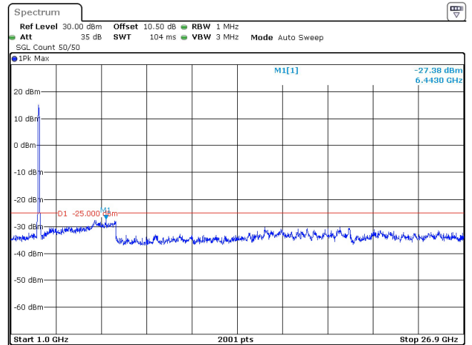
80MHz_30kHz_2592.99MHz_DFT-s-OFDM QPSK_RB216@0 -27.38 dBm
