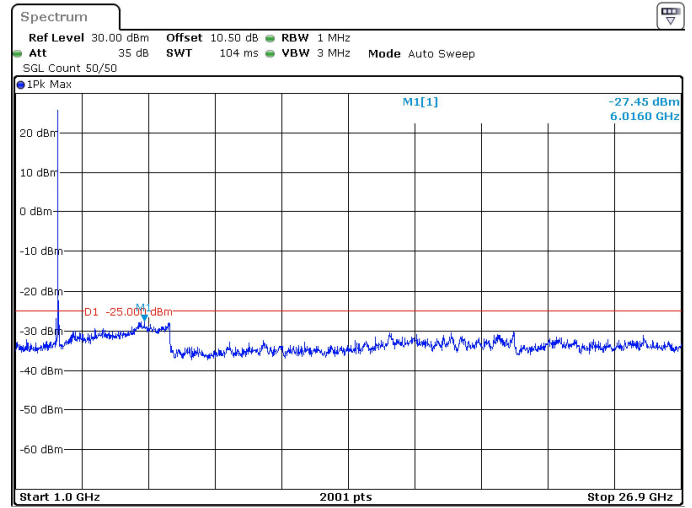
50MHz_30kHz_2664.99MHz_DFT-s-OFDM QPSK_RB1@0 -27.45 dBm
