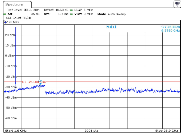
50MHz_30kHz_2664.99MHz_DFT-s-OFDM QPSK_RB1@132 -27.84 dBm
