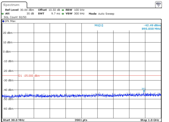
50MHz_30kHz_2592.99MHz_DFT-s-OFDM QPSK_RB1@132 -42.49 dBm
