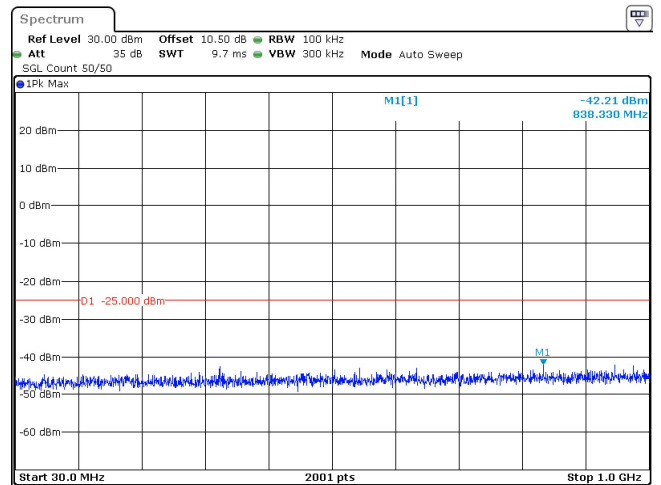
50MHz_30kHz_2592.99MHz_DFT-s-OFDM QPSK_RB128@0 -42.21 dBm
