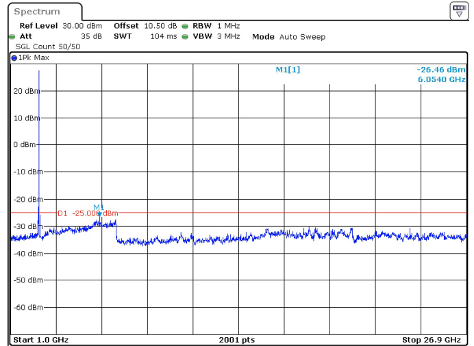
50MHz_30kHz_2592.99MHz_DFT-s-OFDM QPSK_RB1@132 -26.46 dBm
