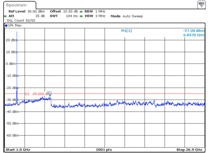
50MHz_30kHz_2592.99MHz_DFT-s-OFDM QPSK_RB1@0 -27.30 dBm
