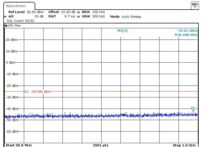
60MHz_30kHz_2526MHz_DFT-s-OFDM QPSK_RB162@0 -42.61 dBm
