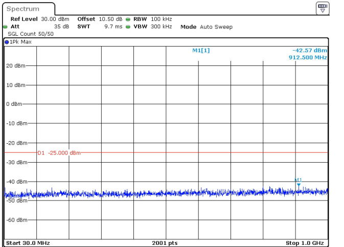
50MHz_30kHz_2664.99MHz_DFT-s-OFDM QPSK_RB1@132 -42.57 dBm
