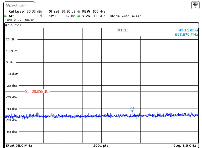
50MHz_30kHz_2664.99MHz_DFT-s-OFDM QPSK_RB128@0 -43.11 dBm
