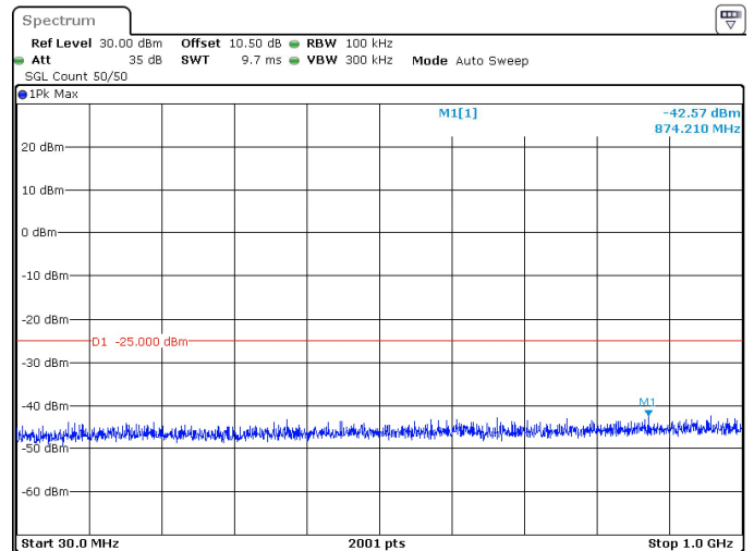
60MHz_30kHz_2526MHz_DFT-s-OFDM QPSK_RB1@161 -42.57 dBm
