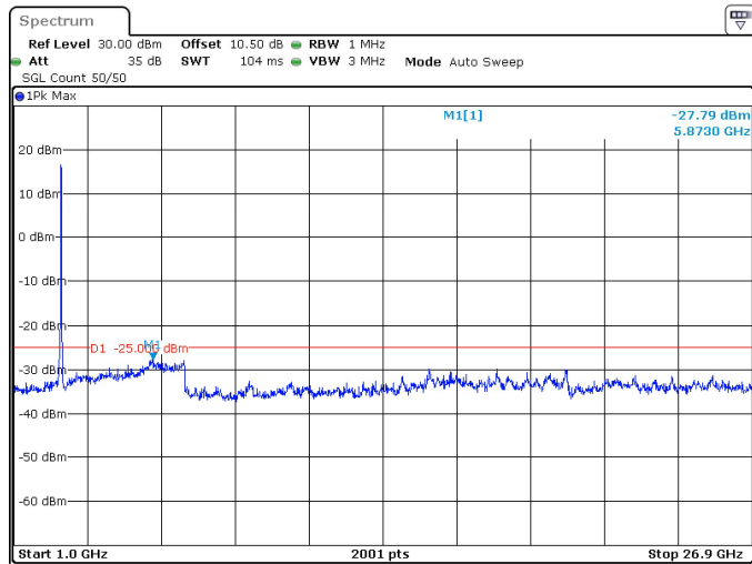
50MHz_30kHz_2664.99MHz_DFT-s-OFDM QPSK_RB128@0 -27.79 dBm
