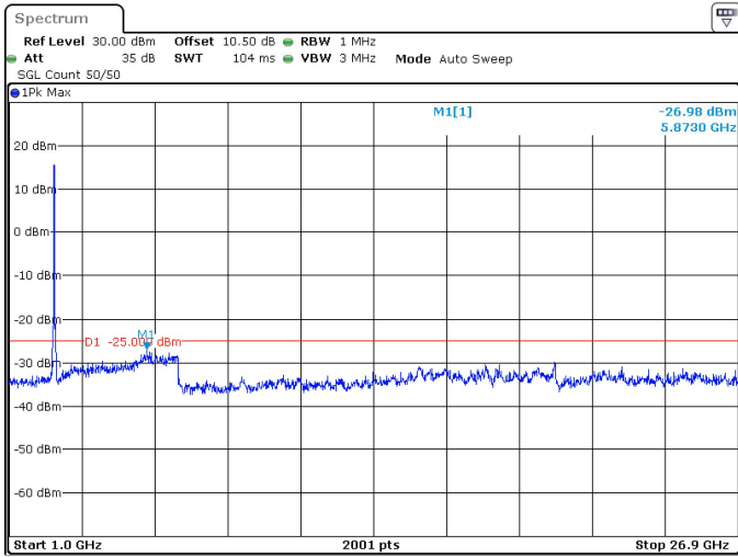
50MHz_30kHz_2592.99MHz_DFT-s-OFDM QPSK_RB128@0 -26.98 dBm
