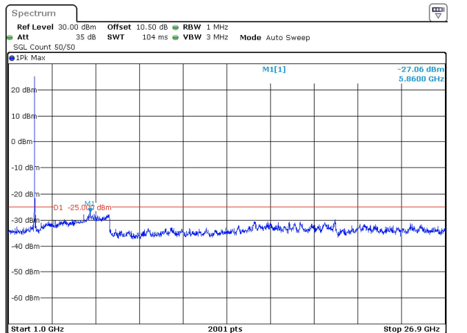
60MHz_30kHz_2526MHz_DFT-s-OFDM QPSK_RB1@161 -27.06 dBm
