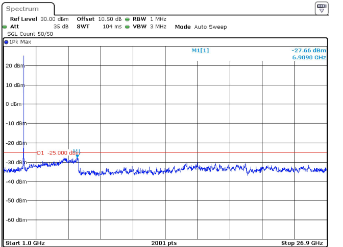
40MHz_30kHz_2592.99MHz_DFT-s-OFDM QPSK_RB1@105 -27.66 dBm
