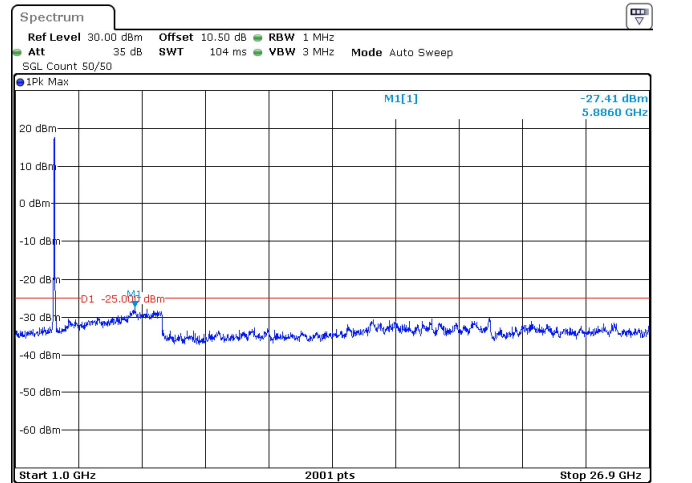
40MHz_30kHz_2592.99MHz_DFT-s-OFDM QPSK_RB100@0 -27.41 dBm
