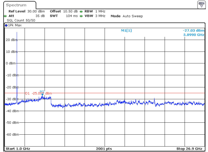
40MHz_30kHz_2592.99MHz_DFT-s-OFDM QPSK_RB1@0 -27.03 dBm
