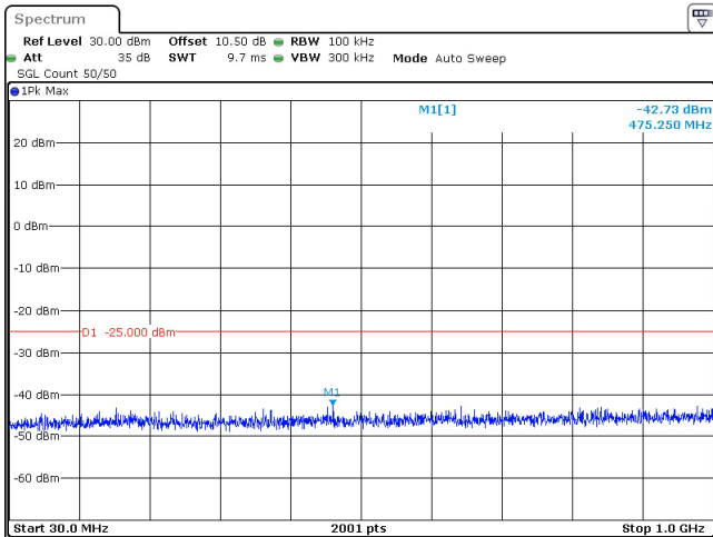
50MHz_30kHz_2521.02MHz_DFT-s-OFDM QPSK_RB1@132 -42.73 dBm
