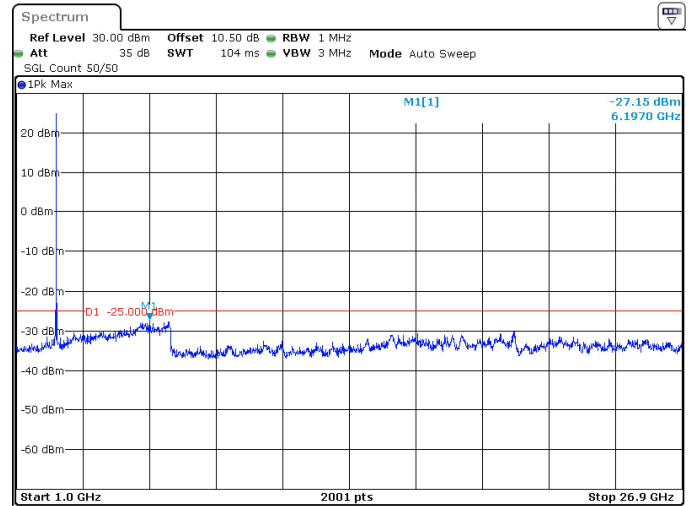
50MHz_30kHz_2521.02MHz_DFT-s-OFDM QPSK_RB1@132 -27.15 dBm
