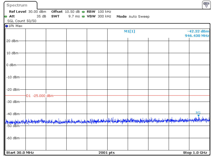
50MHz_30kHz_2521.02MHz_DFT-s-OFDM QPSK_RB1@0 -42.32 dBm
