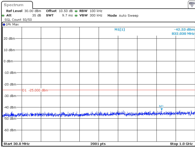
40MHz_30kHz_2592.99MHz_DFT-s-OFDM QPSK_RB100@0 -42.53 dBm
