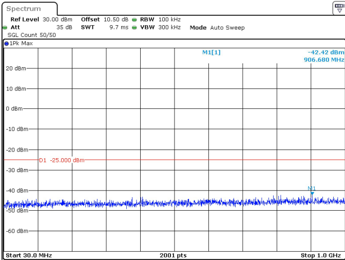
40MHz_30kHz_2592.99MHz_DFT-s-OFDM QPSK_RB1@0 -42.42 dBm
