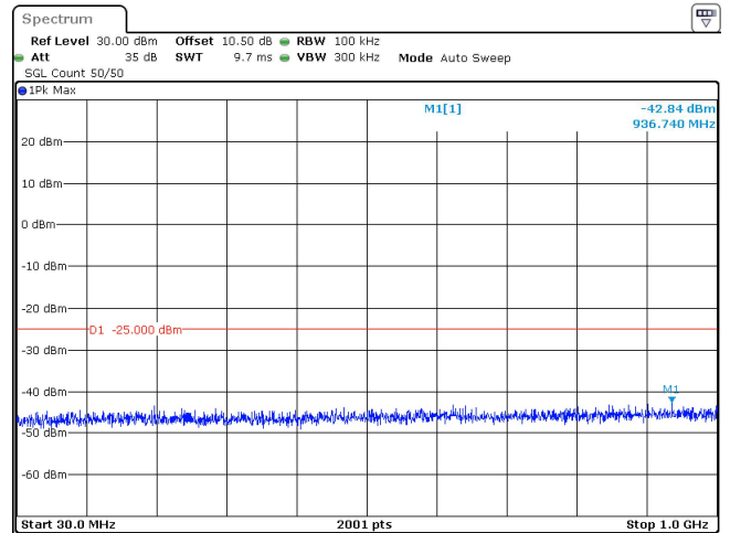
40MHz_30kHz_2670MHz_DFT-s-OFDM QPSK_RB100@0 -42.84 dBm
