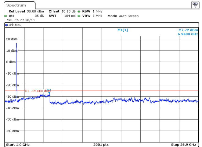
50MHz_30kHz_2521.02MHz_DFT-s-OFDM QPSK_RB128@0 -27.72 dBm
