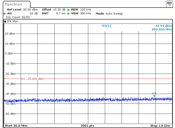
40MHz_30kHz_2592.99MHz_DFT-s-OFDM QPSK_RB1@105 -42.94 dBm
