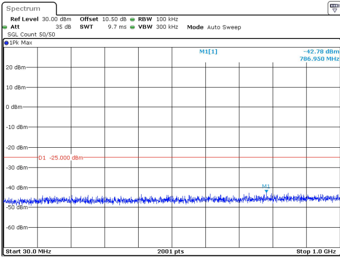
40MHz_30kHz_2516.01MHz_DFT-s-OFDM QPSK_RB100@0 -42.78 dBm
