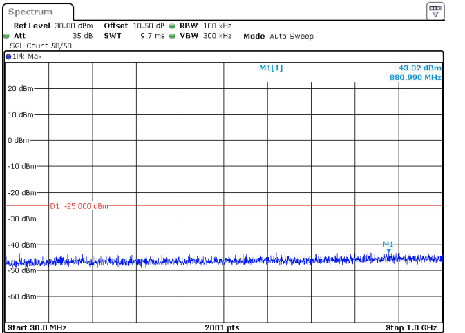
40MHz_30kHz_2516.01MHz_DFT-s-OFDM QPSK_RB1@105 -43.32 dBm
