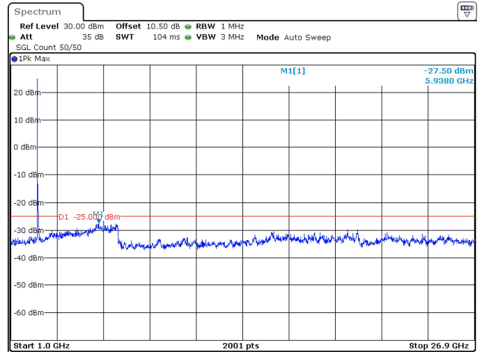
40MHz_30kHz_2516.01MHz_DFT-s-OFDM QPSK_RB1@0 -27.50 dBm
