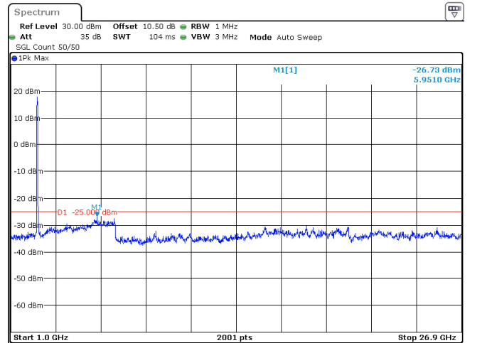
40MHz_30kHz_2516.01MHz_DFT-s-OFDM QPSK_RB100@0 -26.73 dBm
