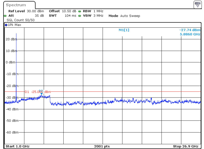
40MHz_30kHz_2516.01MHz_DFT-s-OFDM QPSK_RB1@105 -27.74 dBm
