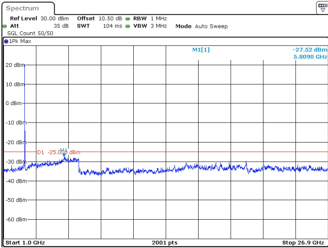
15MHz_30kHz_2682.48MHz_DFT-s-OFDM QPSK_RB36@0 -27.52 dBm
