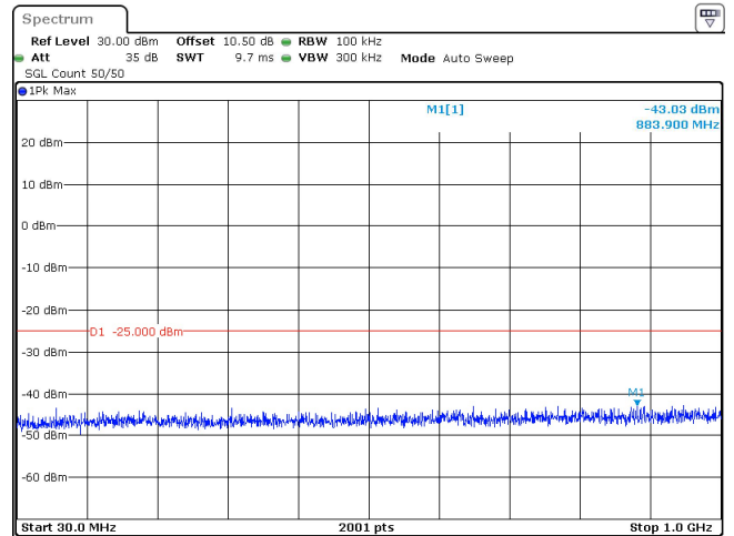
15MHz_30kHz_2592.99MHz_DFT-s-OFDM QPSK_RB36@0 -43.03 dBm
