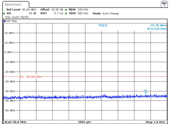
15MHz_30kHz_2682.48MHz_DFT-s-OFDM QPSK_RB36@0 -42.76 dBm
