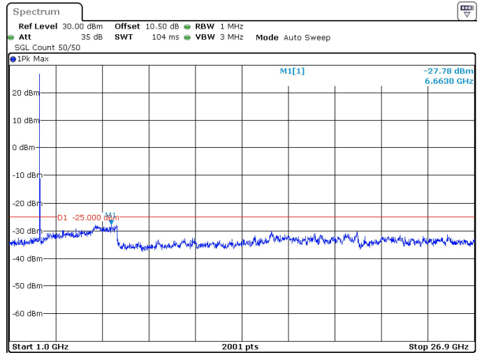
15MHz_30kHz_2682.48MHz_DFT-s-OFDM QPSK_RB1@37 -27.78 dBm
