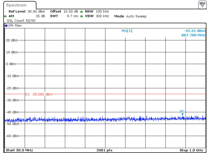
15MHz_30kHz_2592.99MHz_DFT-s-OFDM QPSK_RB1@37 -42.51 dBm
