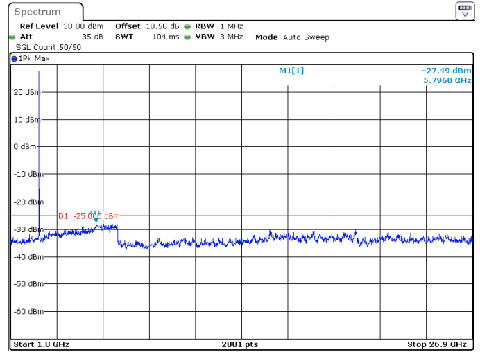
15MHz_30kHz_2592.99MHz_DFT-s-OFDM QPSK_RB1@0 -27.49 dBm
