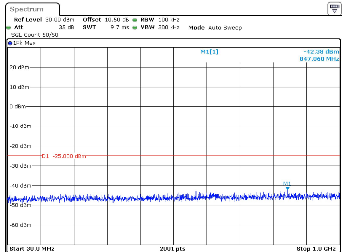
15MHz_30kHz_2503.5MHz_DFT-s-OFDM QPSK_RB1@37 -42.38 dBm
