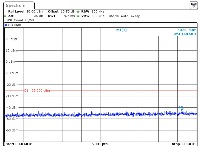
10MHz_30kHz_2592.99MHz_DFT-s-OFDM QPSK_RB1@23 -43.23 dBm
