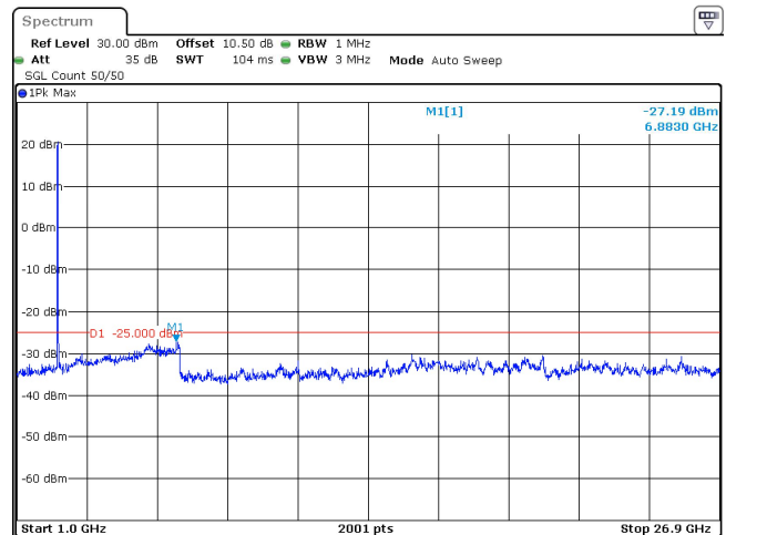
15MHz_30kHz_2503.5MHz_DFT-s-OFDM QPSK_RB36@0 -27.19 dBm
