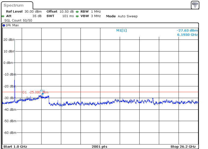
15MHz_30kHz_2595MHz_DFT-s-OFDM QPSK_RB36@0 -27.63 dBm
