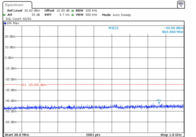
15MHz_30kHz_2612.5MHz_DFT-s-OFDM QPSK_RB36@0 -43.05 dBm
