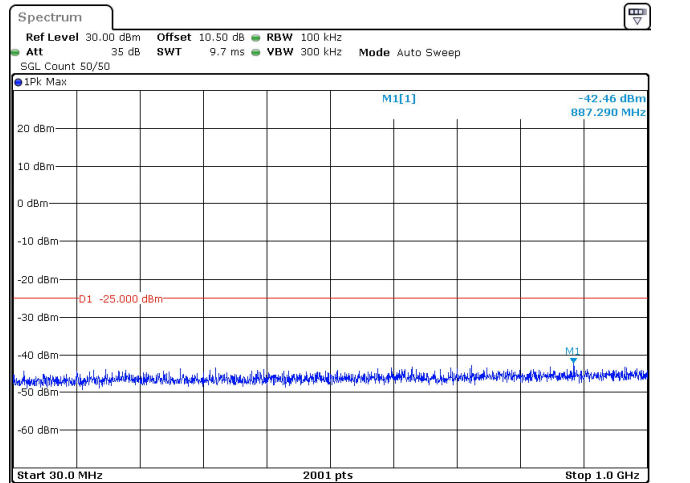
15MHz_30kHz_2595MHz_DFT-s-OFDM QPSK_RB36@0 -42.46 dBm
