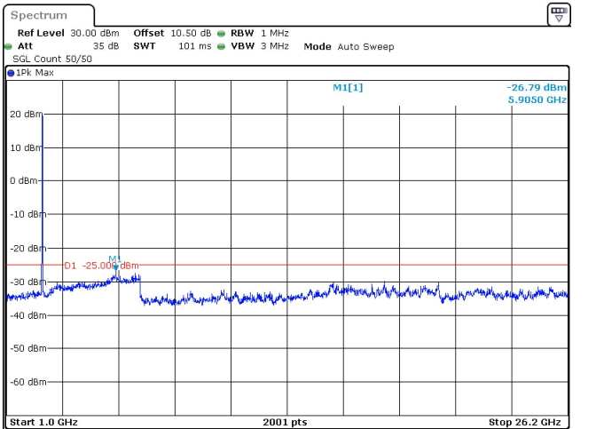
15MHz_30kHz_2612.5MHz_DFT-s-OFDM QPSK_RB36@0 -26.79 dBm
