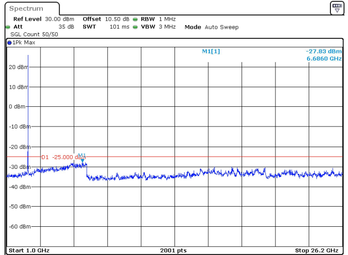
15MHz_30kHz_2595MHz_DFT-s-OFDM QPSK_RB1@37 -27.83 dBm
