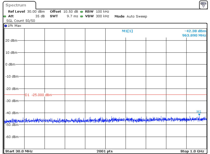
15MHz_30kHz_2612.5MHz_DFT-s-OFDM QPSK_RB1@37 -42.38 dBm
