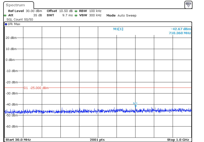
15MHz_30kHz_2577.5MHz_DFT-s-OFDM QPSK_RB36@0 -42.67 dBm
