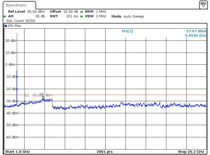
15MHz_30kHz_2595MHz_DFT-s-OFDM QPSK_RB1@0 -27.67 dBm
