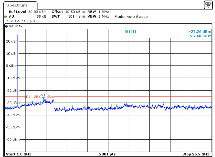
15MHz_30kHz_2577.5MHz_DFT-s-OFDM QPSK_RB1@37 -27.26 dBm
