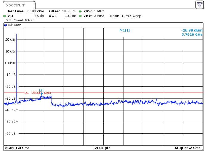
15MHz_30kHz_2612.5MHz_DFT-s-OFDM QPSK_RB1@0 -26.99 dBm
