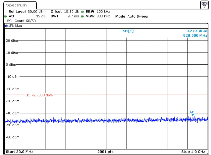
15MHz_30kHz_2577.5MHz_DFT-s-OFDM QPSK_RB1@0 -42.61 dBm
