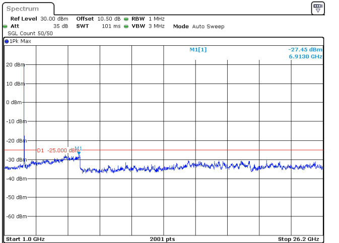
15MHz_30kHz_2577.5MHz_DFT-s-OFDM QPSK_RB36@0 -27.45 dBm
