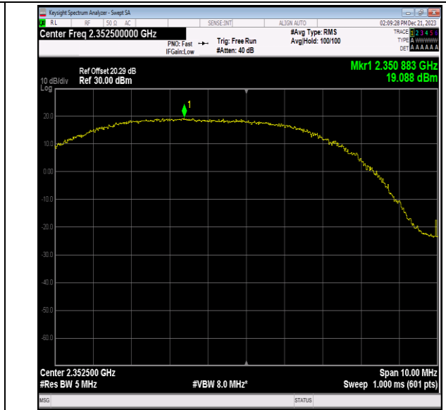
40(2350-2360)-5MHz-16QAM-39175-12RB#0-PASS
