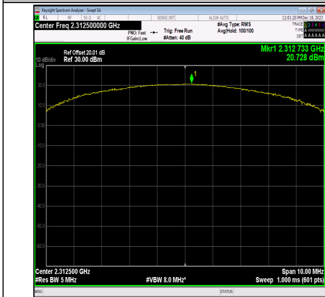
40(2305-2315)-5MHz-64QAM-38775-50RB#0-PASS
