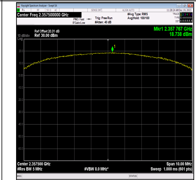
40(2350-2360)-5MHz-16QAM-39225-25RB#12-PASS
