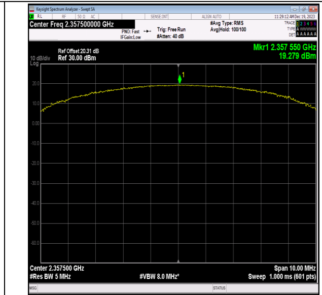
40(2350-2360)-5MHz-16QAM-39225-50RB#0-PASS
