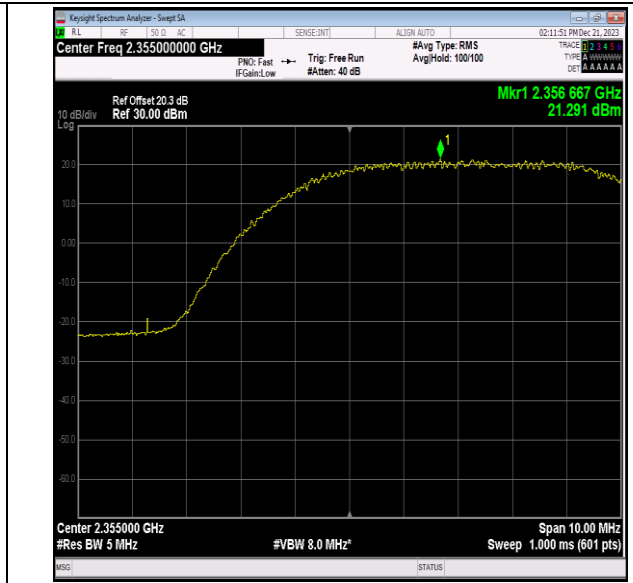
40(2350-2360)-5MHz-QPSK-39200-1RB#24-PASS
