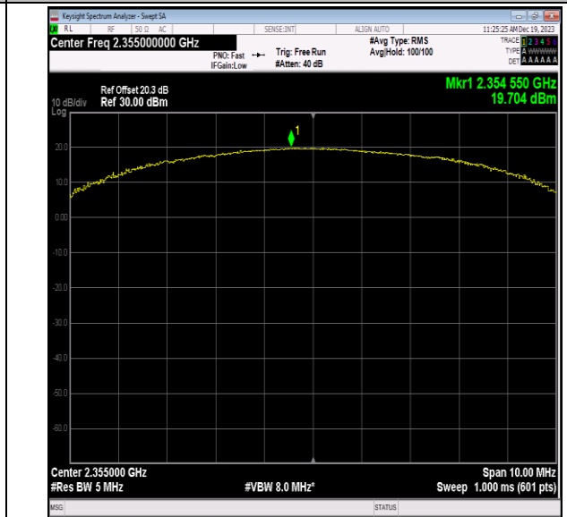
40(2350-2360)-5MHz-QPSK-39200-25RB#12-PASS
