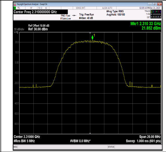
40(2305-2315)-10MHz-16QAM-38750-1RB#24-PASS
