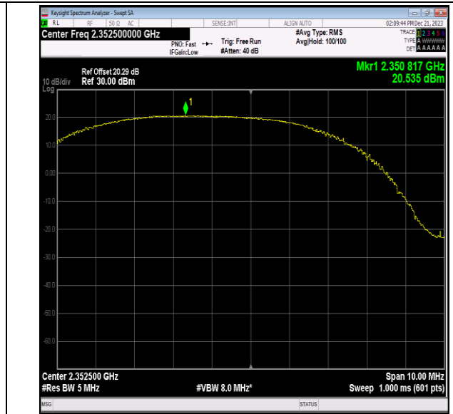
40(2350-2360)-5MHz-QPSK-39175-12RB#6-PASS
