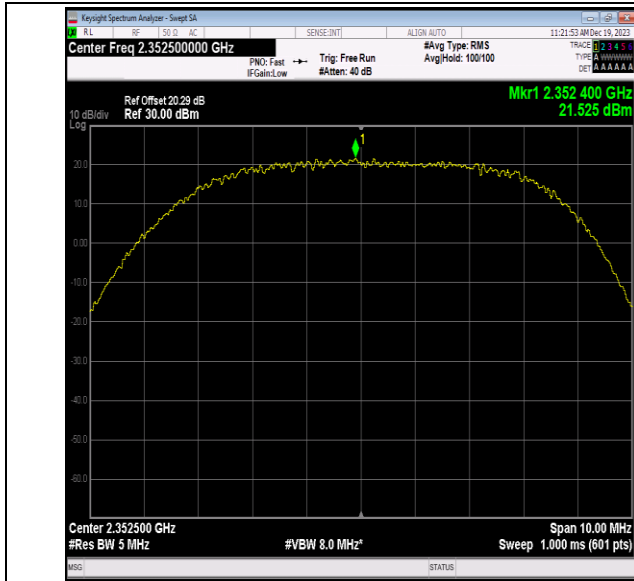
40(2350-2360)-5MHz-16QAM-39175-1RB#49-PASS
