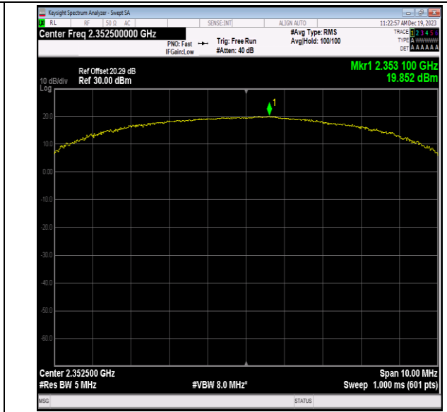
40(2350-2360)-5MHz-QPSK-39175-25RB#25-PASS
