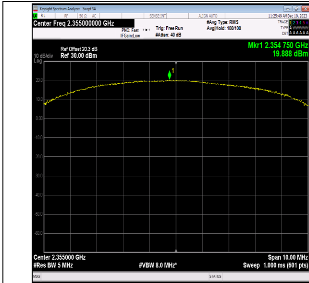
40(2350-2360)-5MHz-QPSK-39200-25RB#25-PASS
