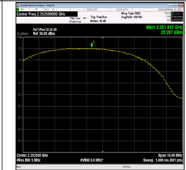
40(2350-2360)-5MHz-16QAM-39175-12RB#11-PASS
