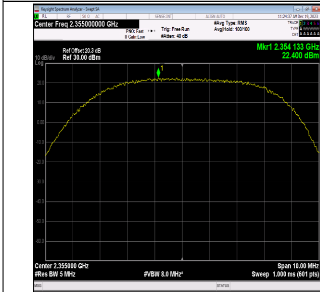
40(2350-2360)-5MHz-QPSK-39200-1RB#49-PASS
