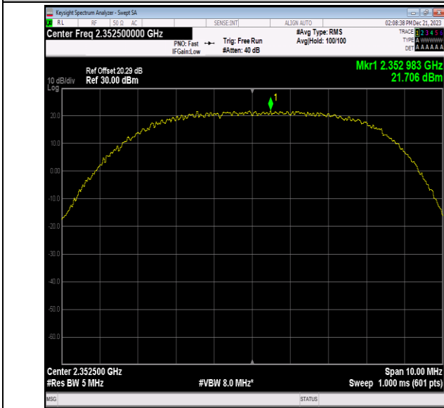
40(2350-2360)-5MHz-16QAM-39175-1RB#12-PASS
