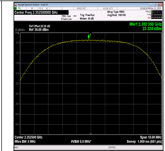
40(2350-2360)-5MHz-QPSK-39175-1RB#12-PASS
