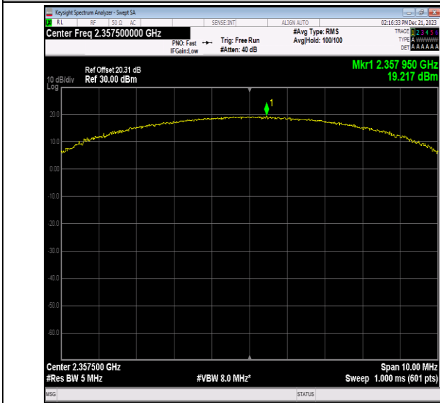
40(2350-2360)-5MHz-16QAM-39225-25RB#0-PASS
