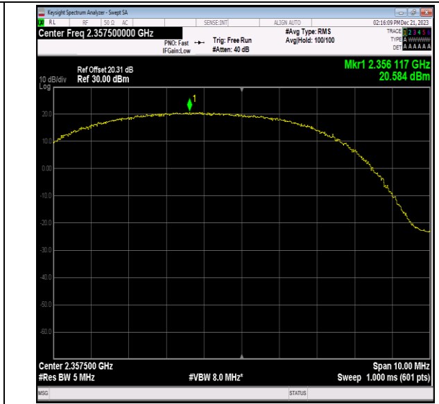
40(2350-2360)-5MHz-16QAM-39225-12RB#11-PASS
