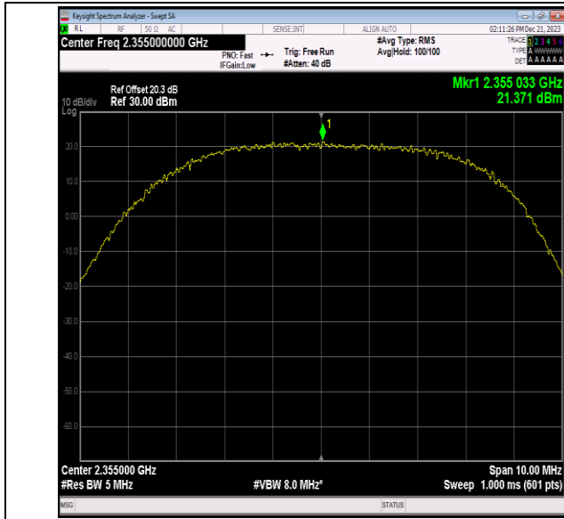
40(2350-2360)-5MHz-QPSK-39200-1RB#12-PASS
