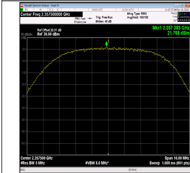
40(2350-2360)-5MHz-16QAM-39225-1RB#49-PASS
