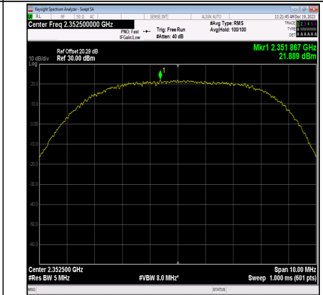
40(2350-2360)-5MHz-QPSK-39175-1RB#49-PASS
