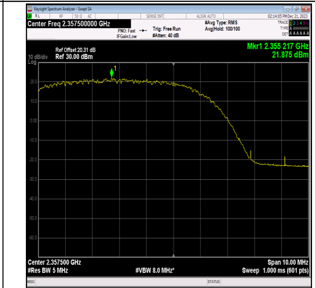
40(2350-2360)-5MHz-16QAM-39225-1RB#0-PASS
