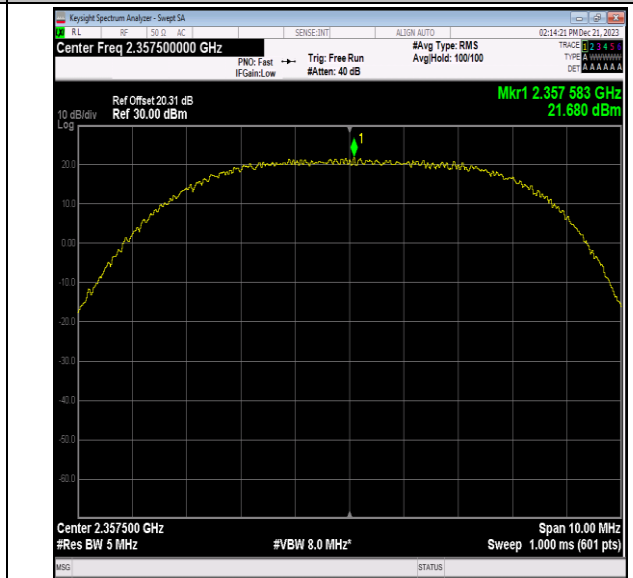
40(2350-2360)-5MHz-QPSK-39225-1RB#12-PASS
