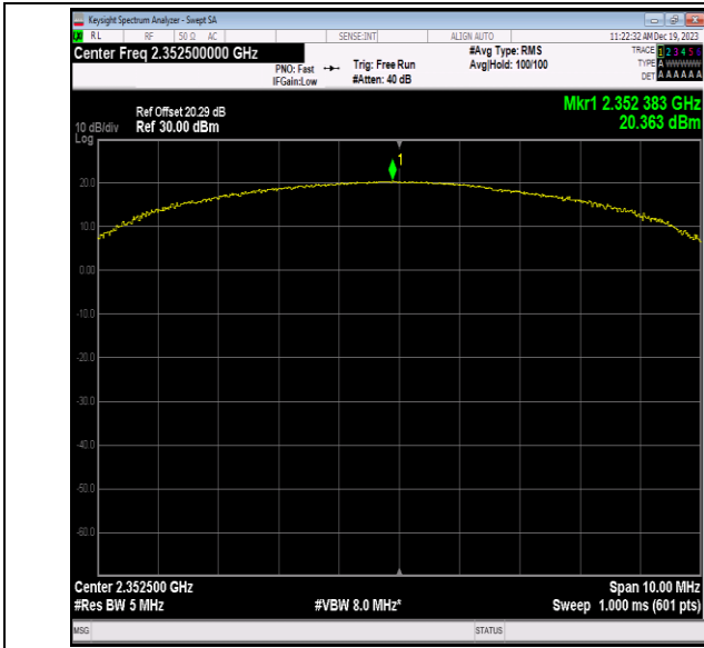
40(2350-2360)-5MHz-QPSK-39175-25RB#12-PASS
