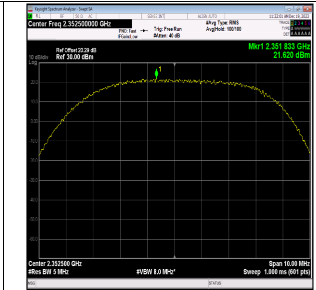
40(2350-2360)-5MHz-64QAM-39175-1RB#49-PASS
