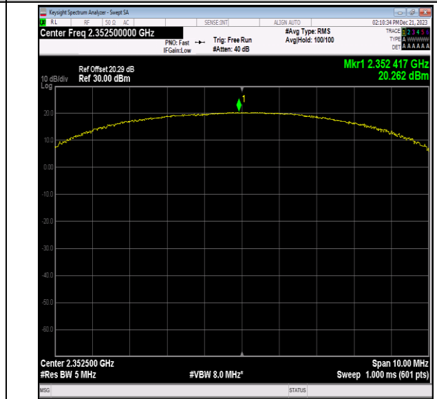
40(2350-2360)-5MHz-QPSK-39175-25RB#0-PASS
