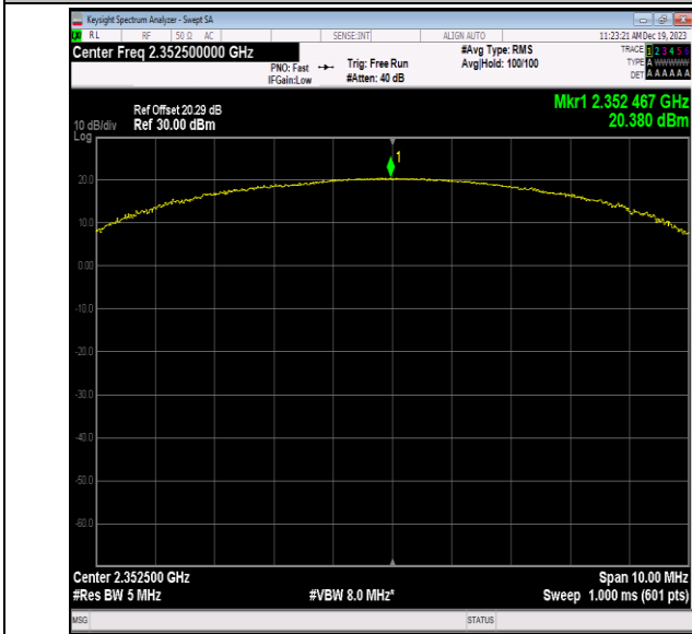
40(2350-2360)-5MHz-QPSK-39175-50RB#0-PASS
