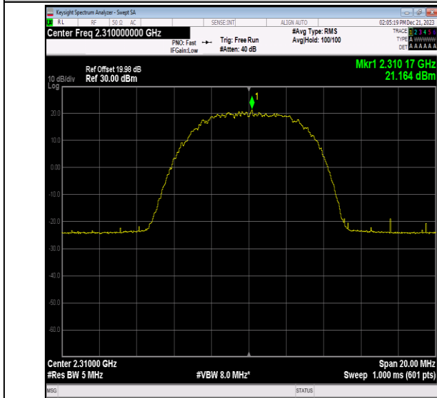
40(2305-2315)-10MHz-64QAM-38750-1RB#24-PASS
