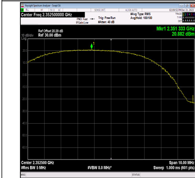
40(2350-2360)-5MHz-16QAM-39175-12RB#6-PASS
