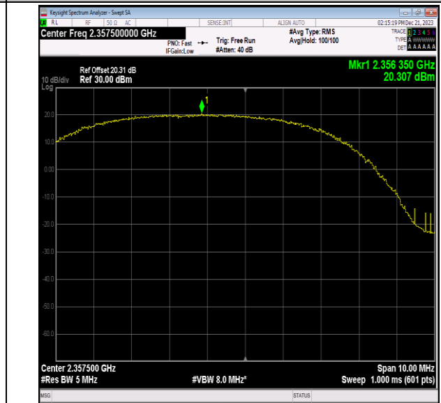
40(2350-2360)-5MHz-16QAM-39225-12RB#0-PASS
