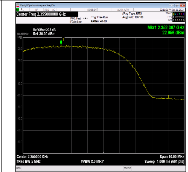
40(2350-2360)-5MHz-QPSK-39200-1RB#0-PASS
