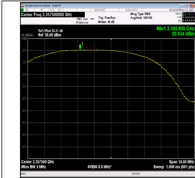
40(2350-2360)-5MHz-QPSK-39225-12RB#11-PASS
