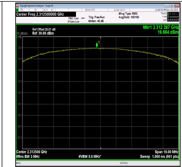
40(2305-2315)-5MHz-64QAM-38775-25RB#25-PASS
