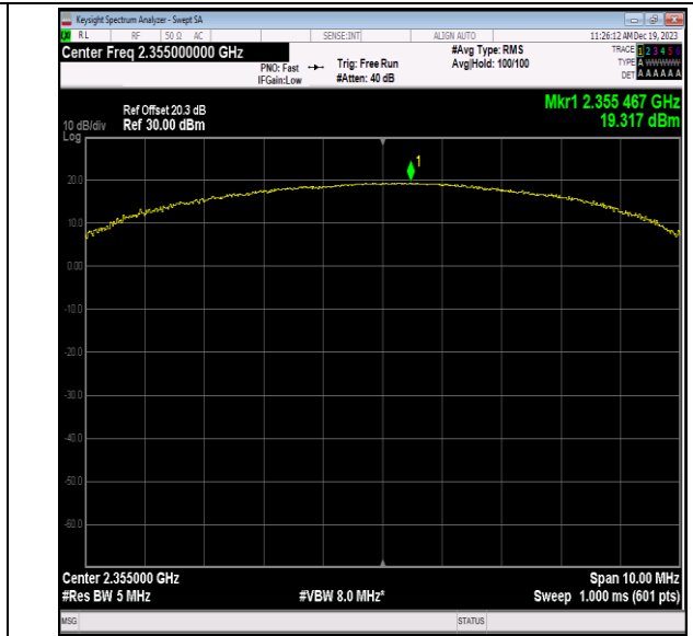
40(2350-2360)-5MHz-QPSK-39200-50RB#0-PASS
