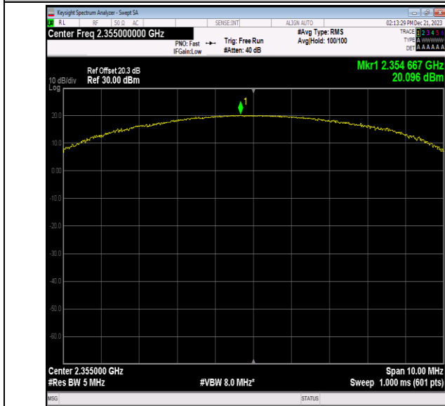
40(2350-2360)-5MHz-QPSK-39200-25RB#0-PASS
