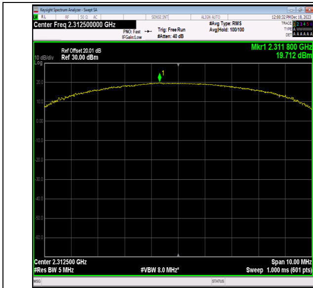
40(2305-2315)-5MHz-64QAM-38775-25RB#12-PASS
