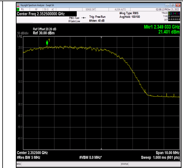
40(2350-2360)-5MHz-16QAM-39175-1RB#0-PASS
