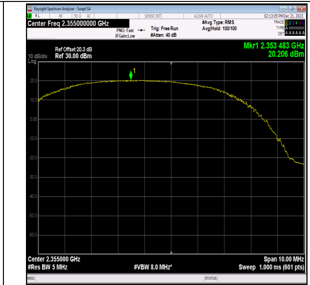
40(2350-2360)-5MHz-QPSK-39200-12RB#11-PASS
