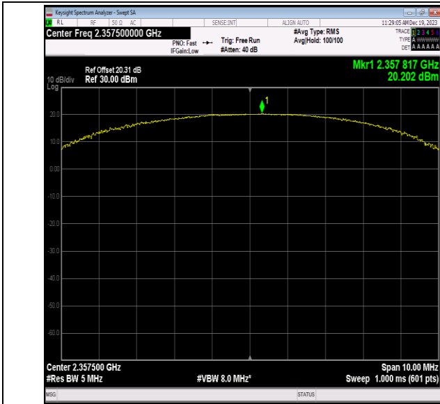
40(2350-2360)-5MHz-QPSK-39225-50RB#0-PASS
