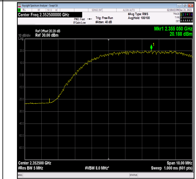
40(2350-2360)-5MHz-16QAM-39175-1RB#24-PASS
