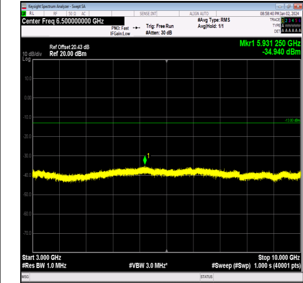
Band26_10MHz_16QAM_26740_1RB#0_3000~10000_30 00~10000
