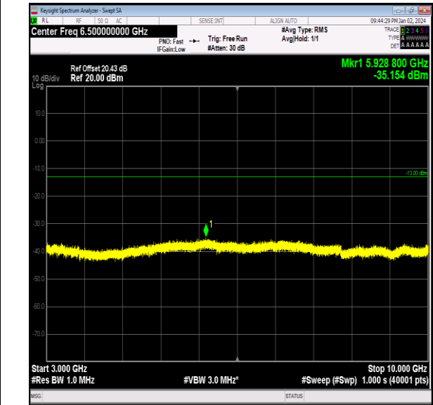
Band26_3MHz_16QAM_27025_1RB#0_3000~10000_300
