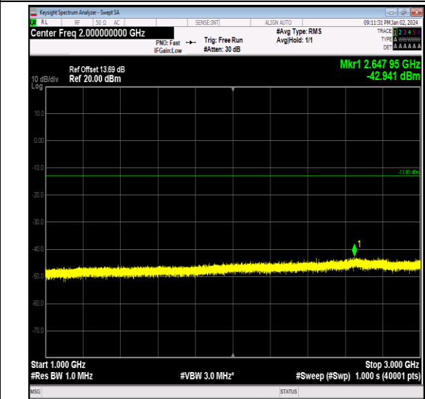
Band26_1.4MHz_QPSK_26797_1RB#0_1000~3000_1000 ~3000
