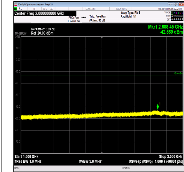
Band26_5MHz_16QAM_26715_1RB#0_1000~3000_1000 ~3000
