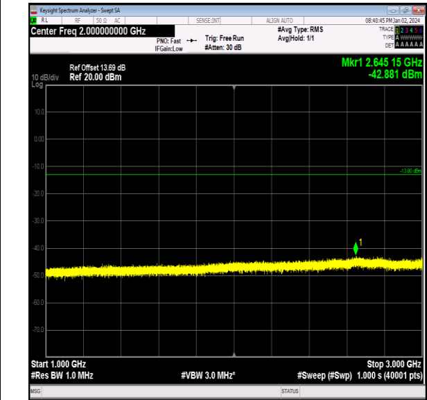
Band26_5MHz_16QAM_26740_1RB#0_1000~3000_1000 ~3000
