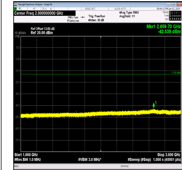
Band26_3MHz_16QAM_27025_1RB#0_1000~3000_1000
