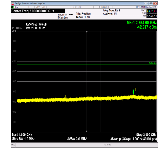
Band26_3MHz_QPSK_27025_1RB#0_1000~3000_1000~3000
