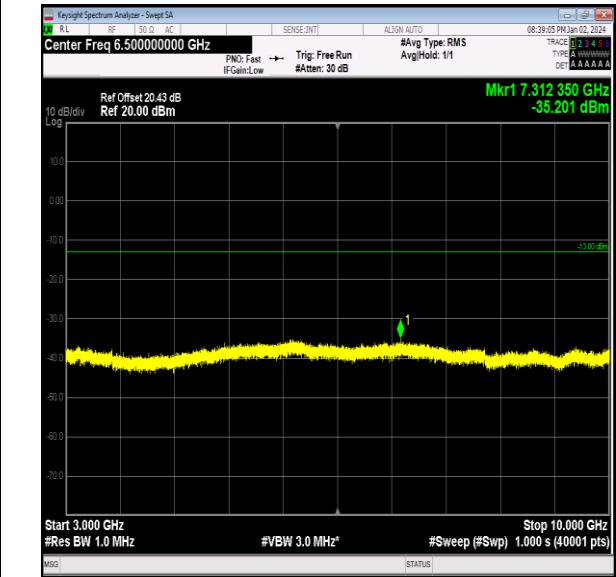
Band26_5MHz_16QAM_26715_1RB#0_3000~10000_3000 0~10000
