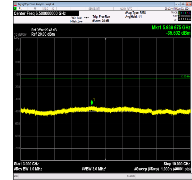
Band26_1.4MHz_16QAM_26797_1RB#0_3000~10000_30 00~10000
