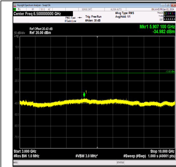
Band26_1.4MHz_16QAM_26915_1RB#0_3000~10000_30 00~10000
