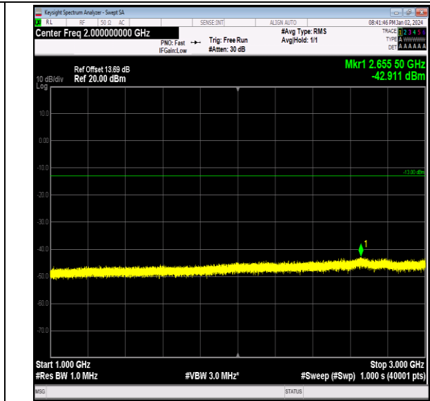
Band26_5MHz_QPSK_26765_1RB#0_1000~3000_1000~3000
