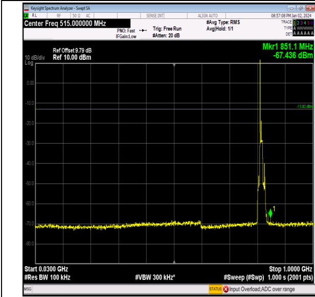
Band26_10MHz_QPSK_26740_1RB#0_30~1000_30~100 0
