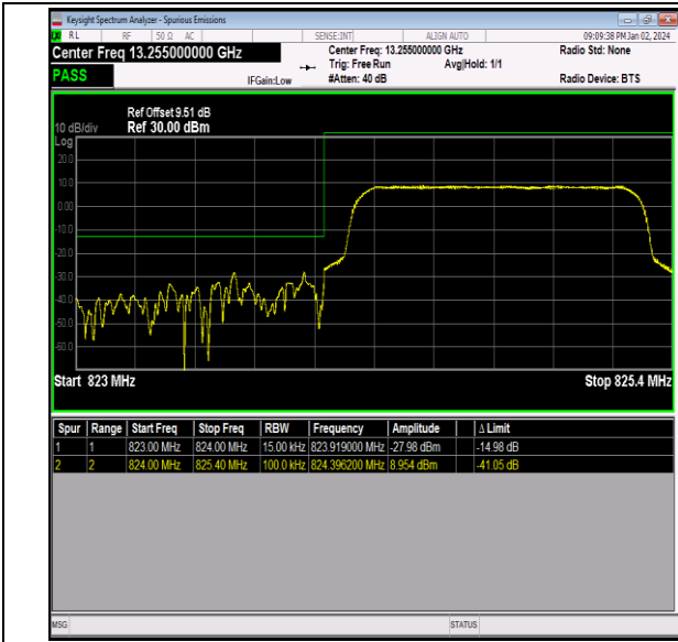
Band26_1.4MHz_16QAM_26797_6RB#0
