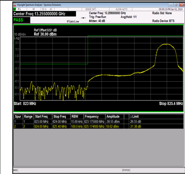
Band26_1.4MHz_16QAM_26797_1RB#5
