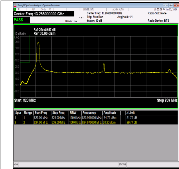
Band26_15MHz_QPSK_26865_1RB#0
