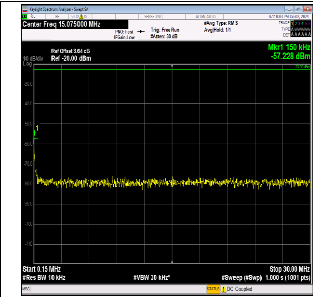
Band13_5MHz_QPSK_23205_1RB#0_0.15~30_0.15~30
