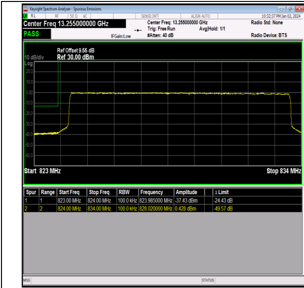
Band26_10MHz_16QAM_26840_50RB#0
