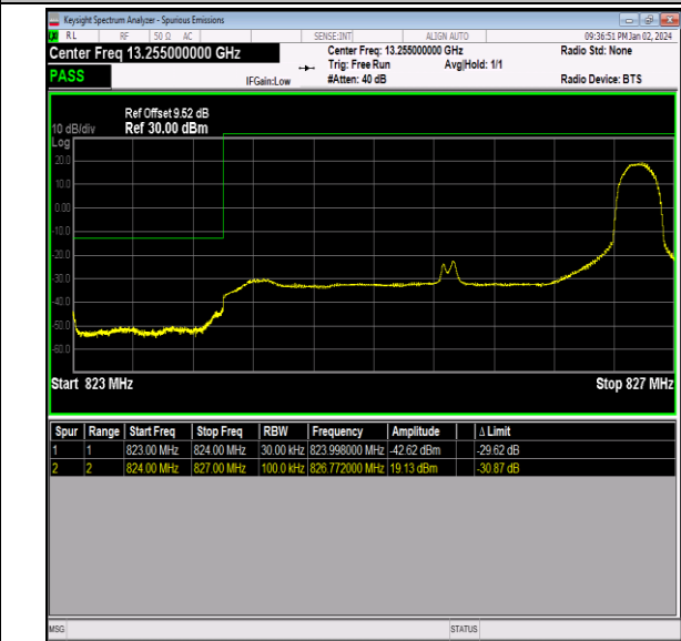
Band26_3MHz_16QAM_26805_1RB#14
