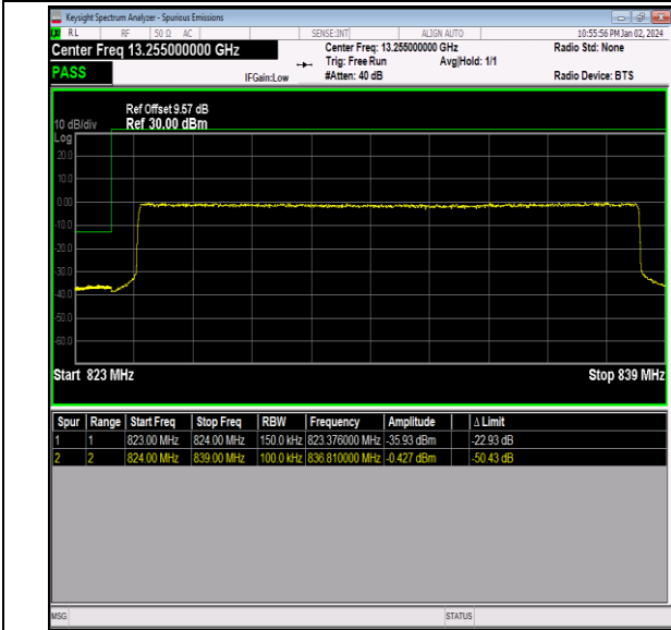
Band26_15MHz_QPSK_26865_75RB#0
