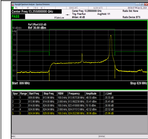
Band26_10MHz_16QAM_26740_1RB#49
