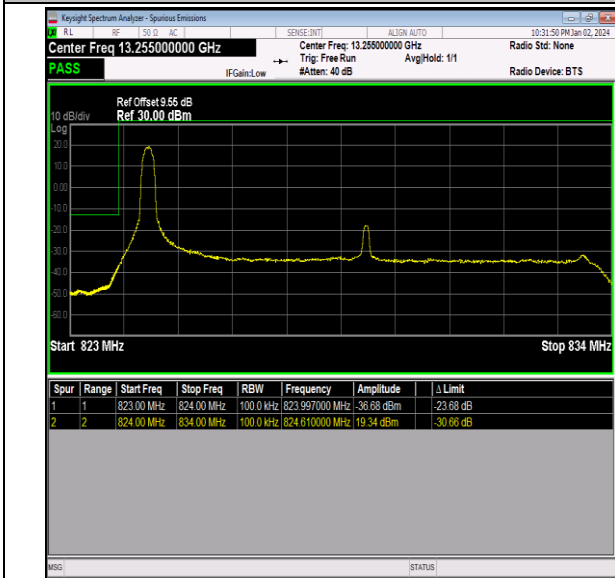
Band26_10MHz_16QAM_26840_1RB#0
