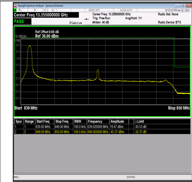
Band26_10MHz_16QAM_26990_1RB#0
