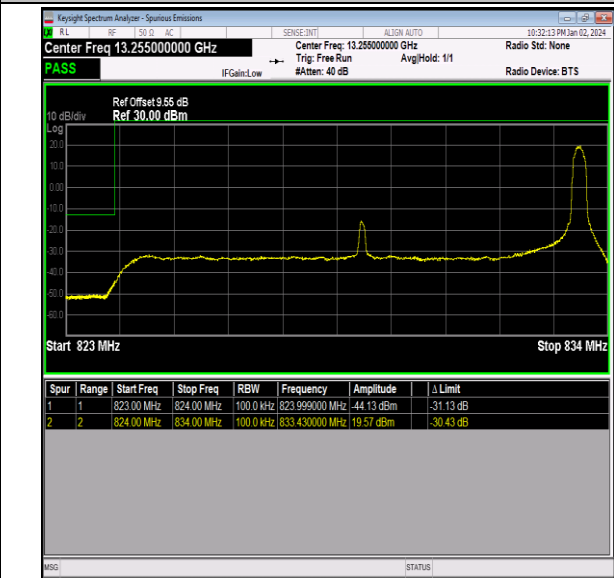
Band26_10MHz_16QAM_26840_1RB#49
