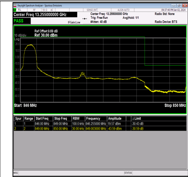
Band26_3MHz_16QAM_27025_1RB#0
