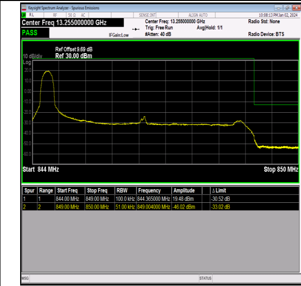
Band26_5MHz_16QAM_27015_1RB#0
