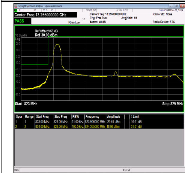
Band26_5MHz_16QAM_26815_1RB#0
