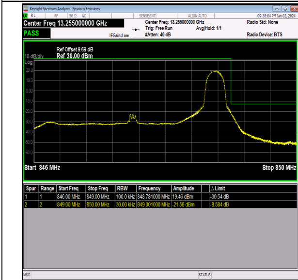
Band26_3MHz_16QAM_27025_1RB#14
