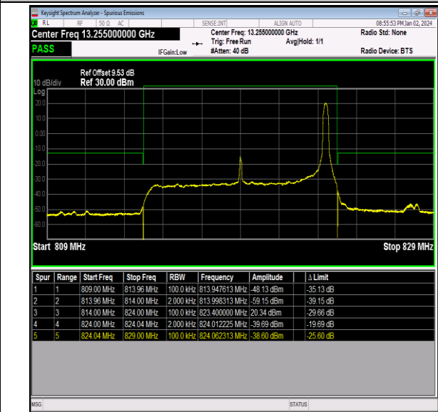
Band26_10MHz_QPSK_26740_1RB#49
