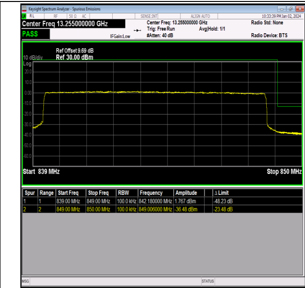
Band26_10MHz_QPSK_26990_50RB#0
