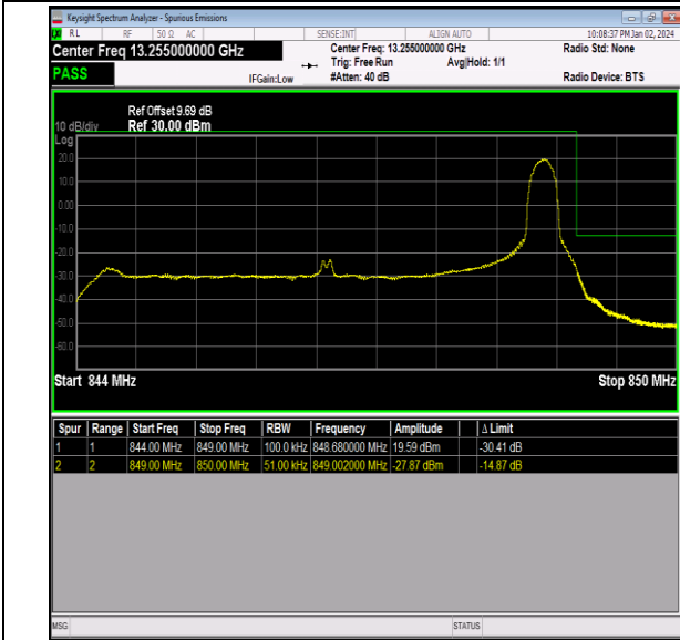
Band26_5MHz_16QAM_27015_1RB#24
