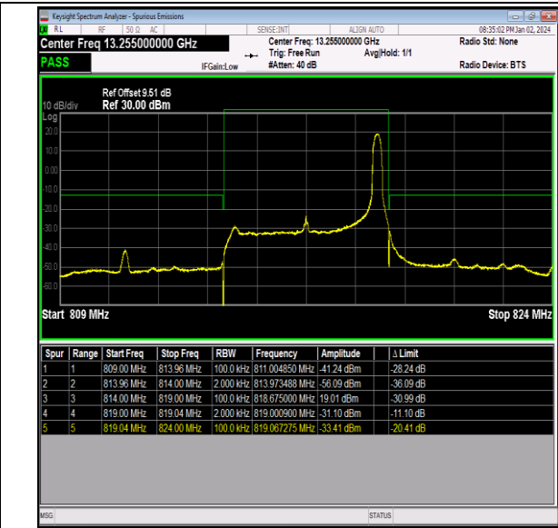
Band26_5MHz_16QAM_26715_1RB#24
