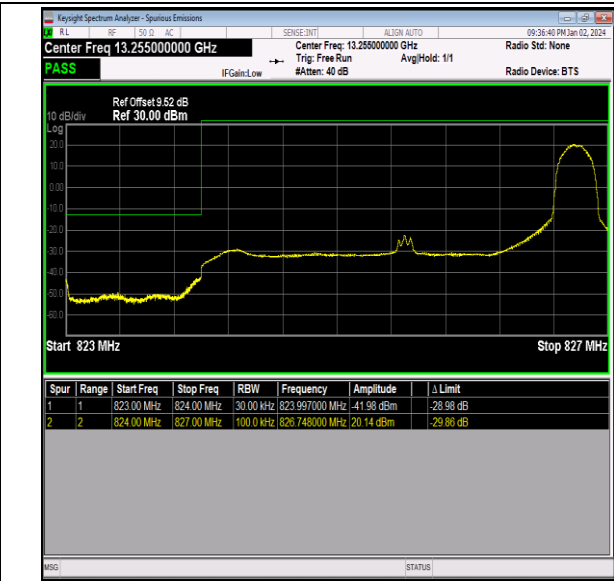
Band26_3MHz_QPSK_26805_1RB#14
