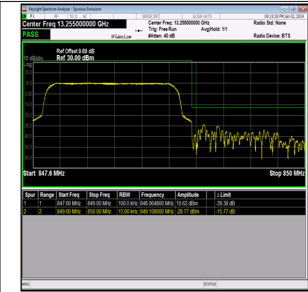
Band26_1.4MHz_QPSK_27033_6RB#0
