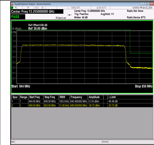
Band26_5MHz_16QAM_27015_25RB#0
