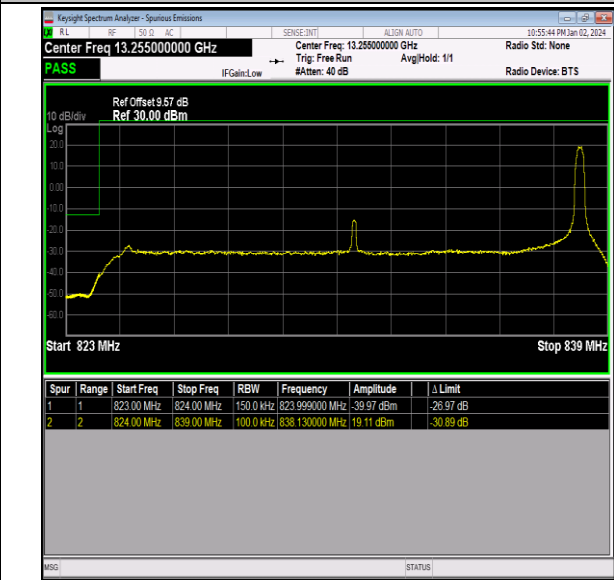
Band26_15MHz_16QAM_26865_1RB#74
