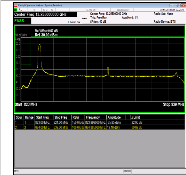
Band26_15MHz_16QAM_26865_1RB#0
