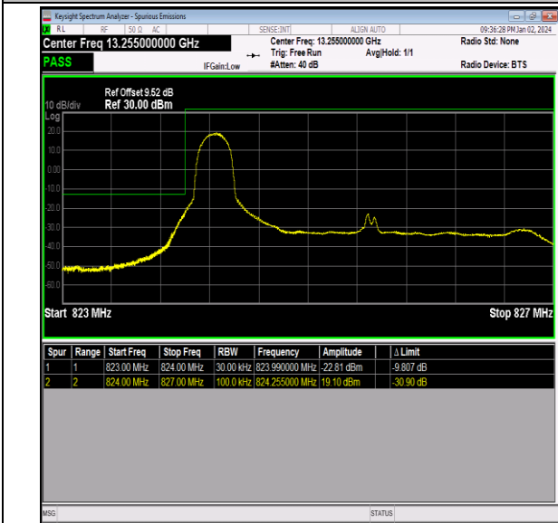
Band26_3MHz_16QAM_26805_1RB#0
