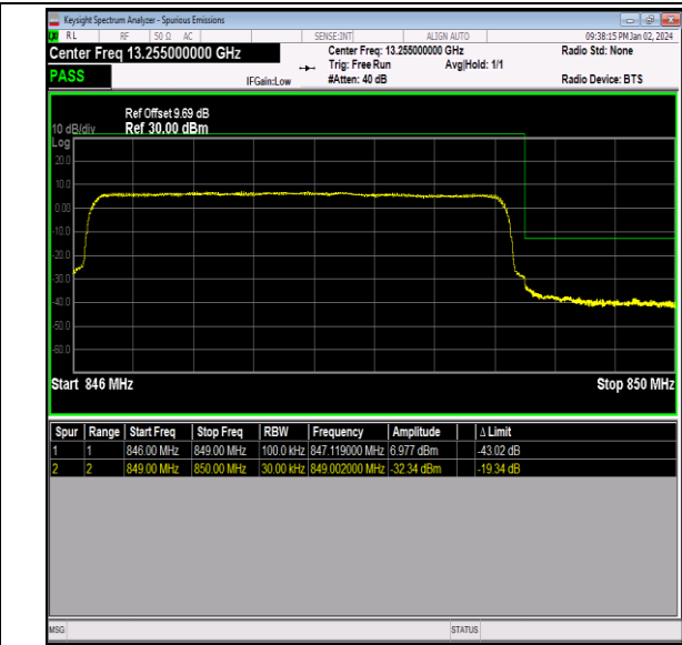
Band26_3MHz_QPSK_27025_15RB#0
