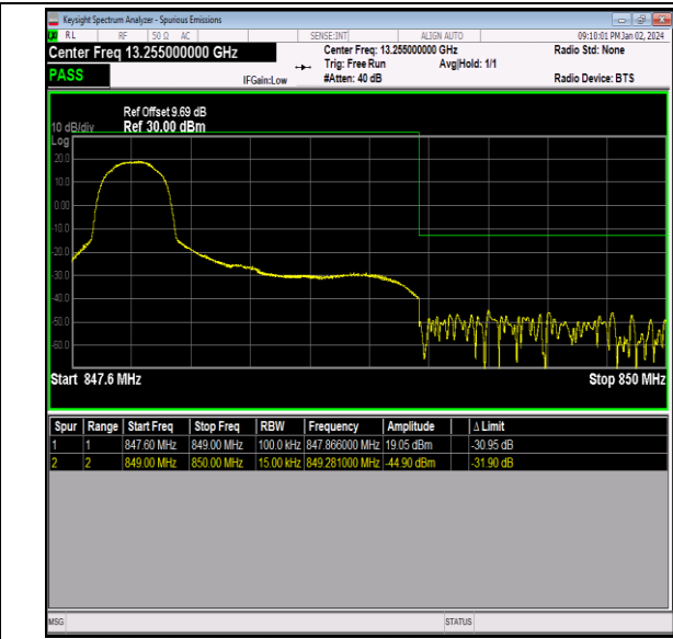
Band26_1.4MHz_16QAM_27033_1RB#0
