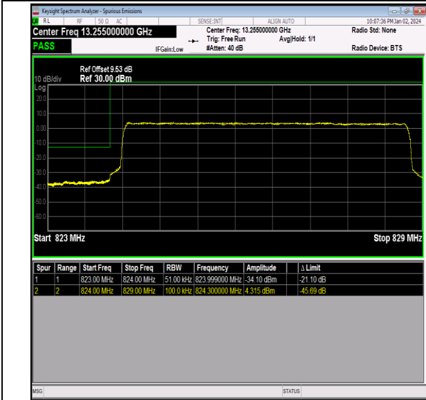
Band26_5MHz_QPSK_26815_25RB#0
