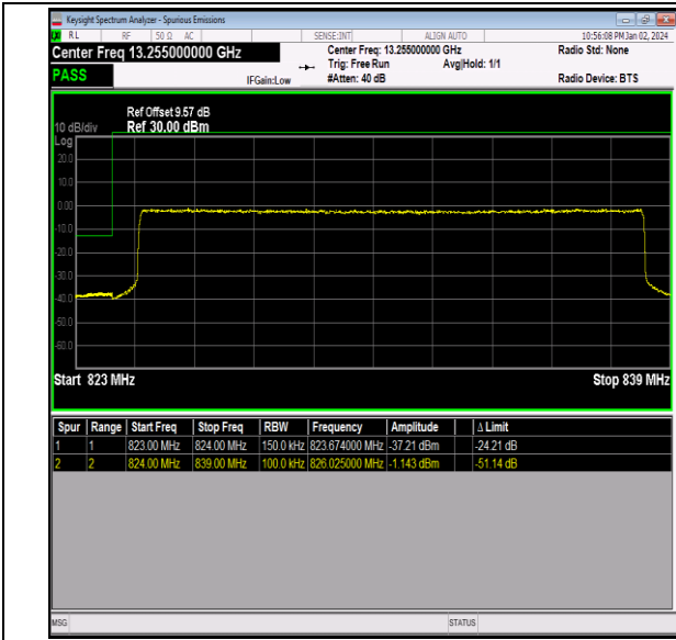
Band26_15MHz_16QAM_26865_75RB#0
