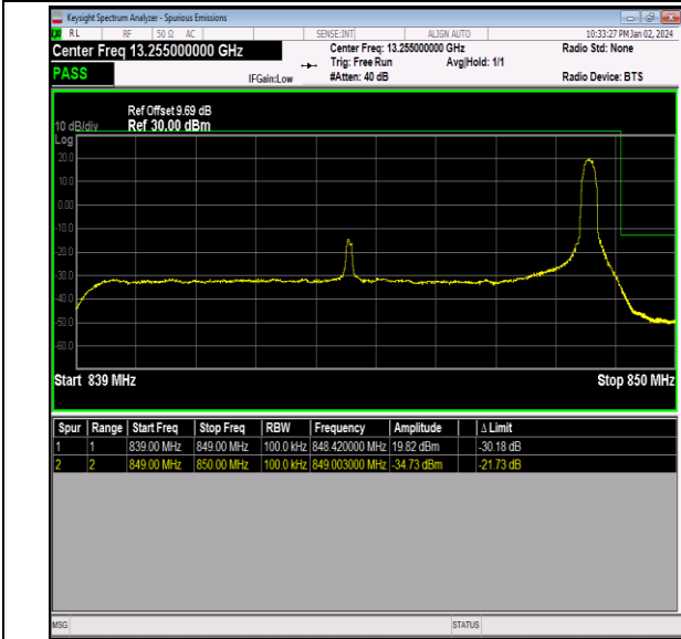
Band26_10MHz_16QAM_26990_1RB#49
