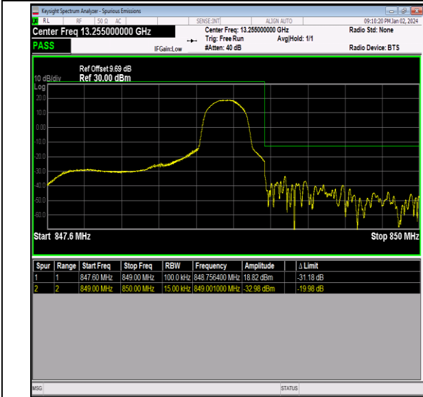
Band26_1.4MHz_16QAM_27033_1RB#5
