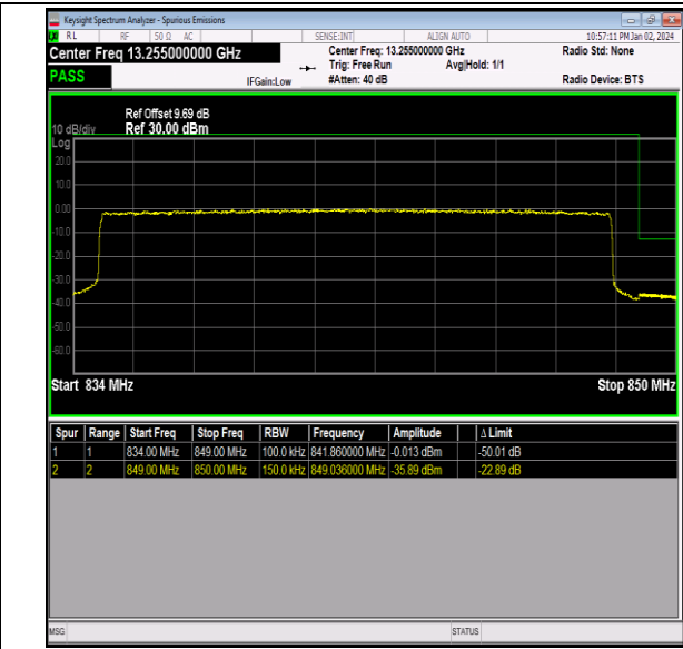
Band26_15MHz_QPSK_26965_75RB#0
