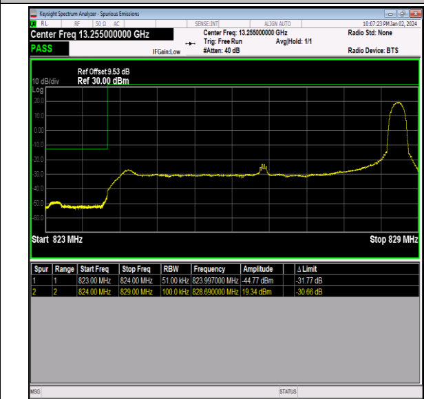
Band26_5MHz_16QAM_26815_1RB#24
