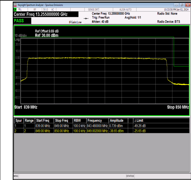
Band26_10MHz_16QAM_26990_50RB#0
