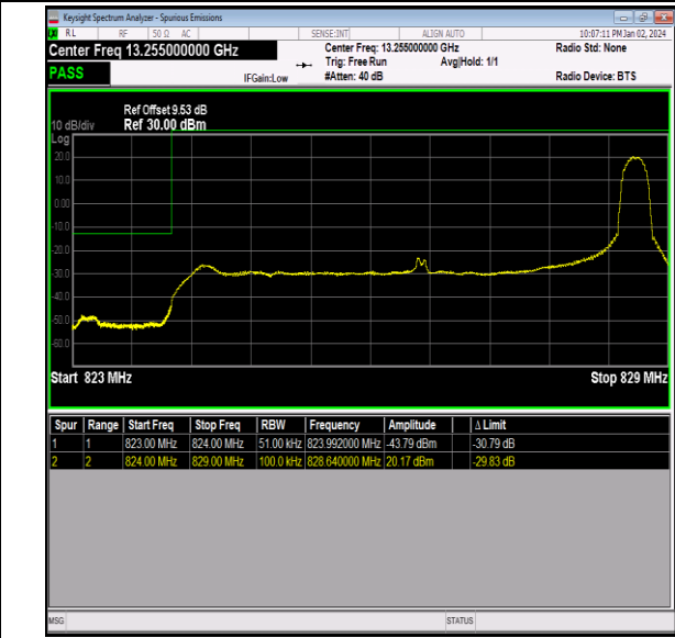
Band26_5MHz_QPSK_26815_1RB#24
