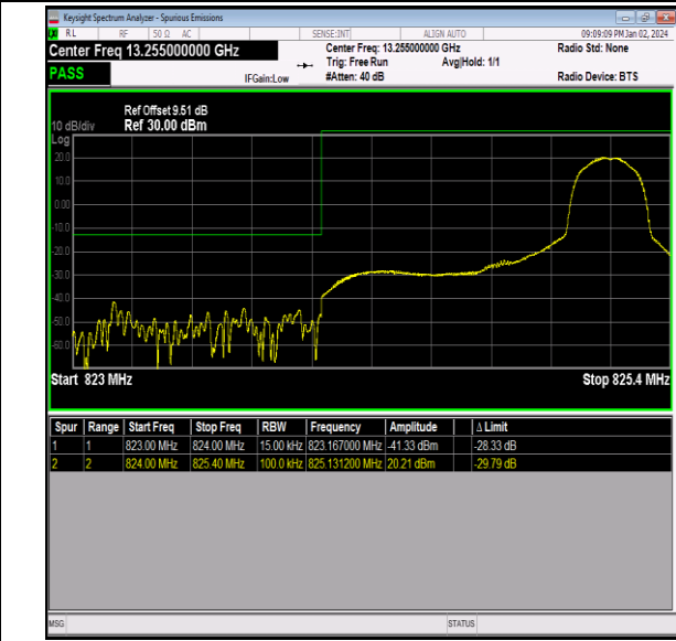
Band26_1.4MHz_QPSK_26797_1RB#5
