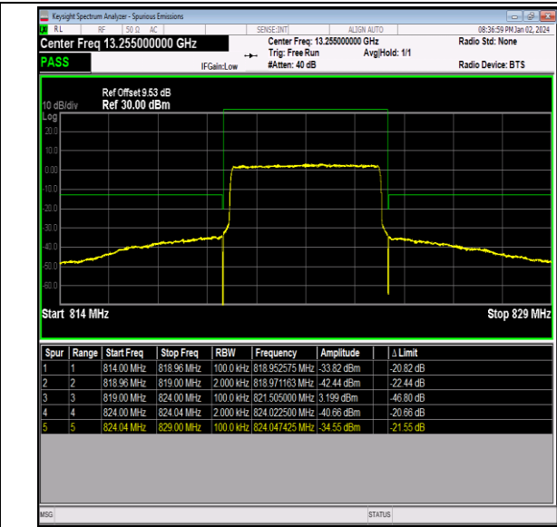
Band26_5MHz_16QAM_26765_25RB#0
