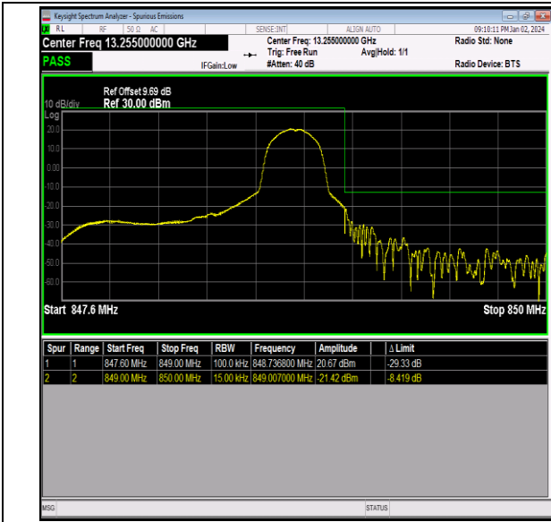
Band26_1.4MHz_QPSK_27033_1RB#5
