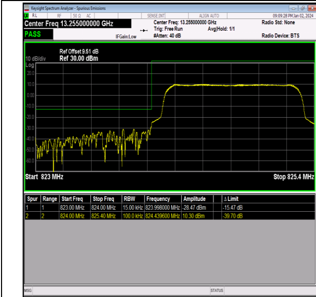
Band26_1.4MHz_QPSK_26797_6RB#0
