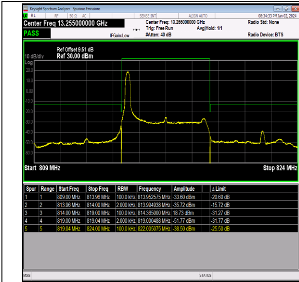
Band26_5MHz_16QAM_26715_1RB#0
