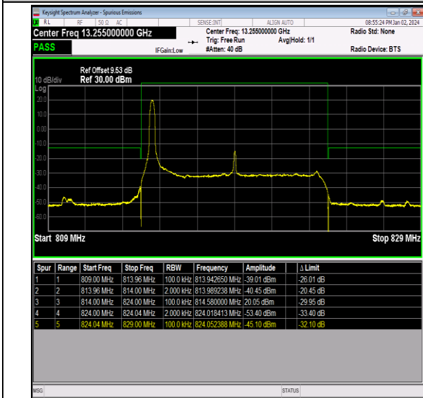
Band26_10MHz_QPSK_26740_1RB#0
