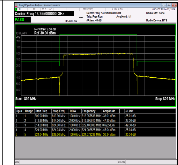
Band26_10MHz_16QAM_26740_50RB#0
