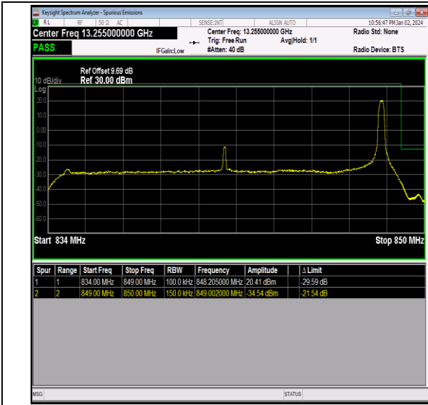
Band26_15MHz_QPSK_26965_1RB#74
