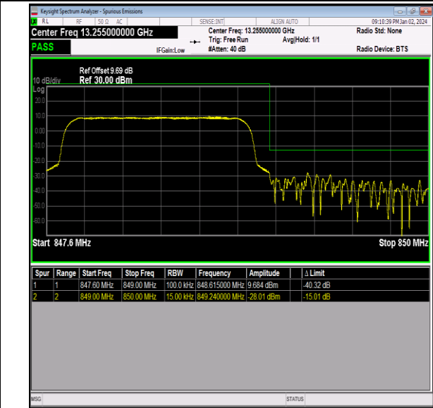
Band26_1.4MHz_16QAM_27033_6RB#0
