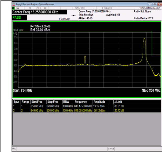
Band26_15MHz_16QAM_26965_1RB#74
