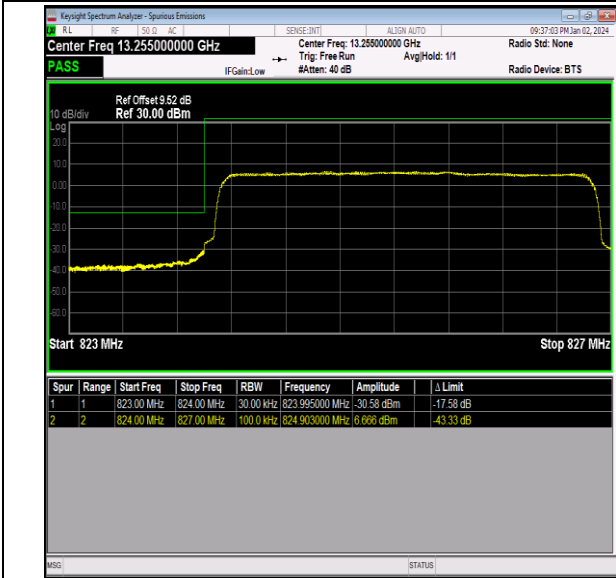
Band26_3MHz_QPSK_26805_15RB#0
