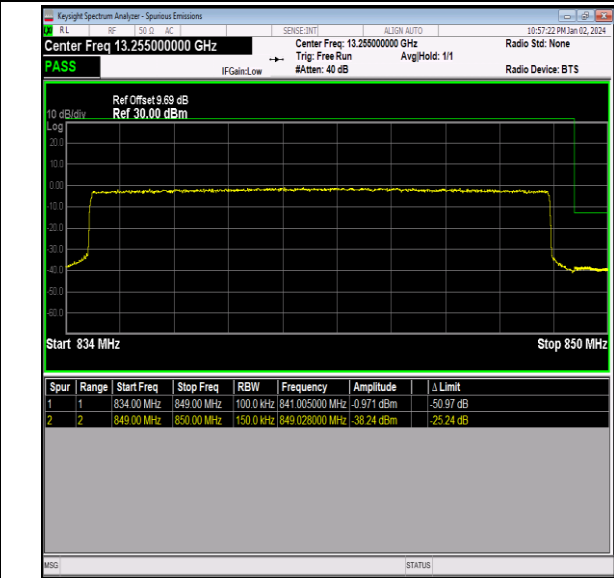
Band26_15MHz_16QAM_26965_75RB#0
