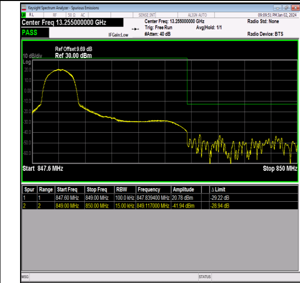
Band26_1.4MHz_QPSK_27033_1RB#0
