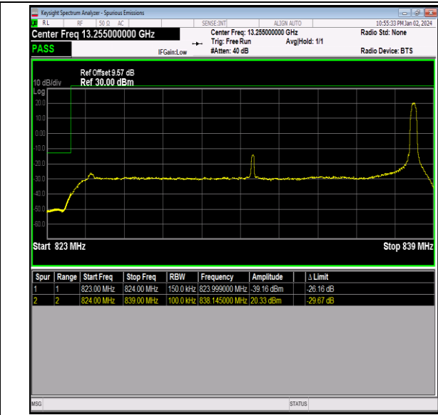
Band26_15MHz_QPSK_26865_1RB#74
