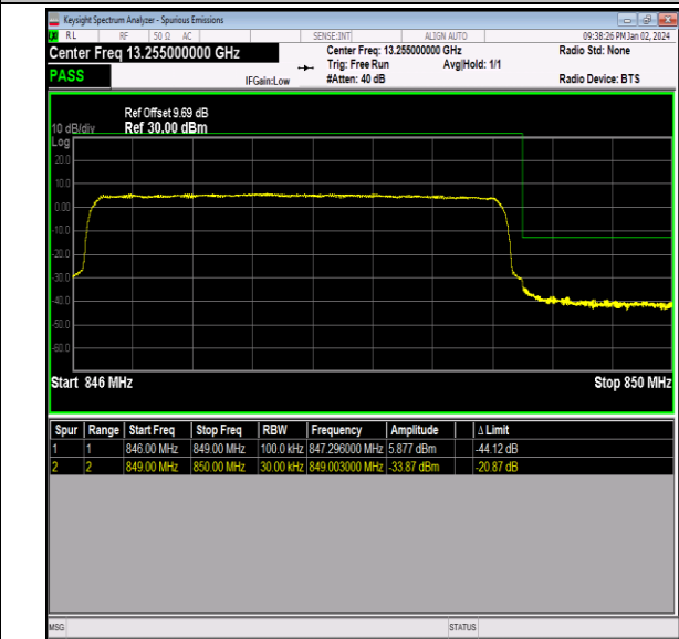
Band26_3MHz_16QAM_27025_15RB#0
