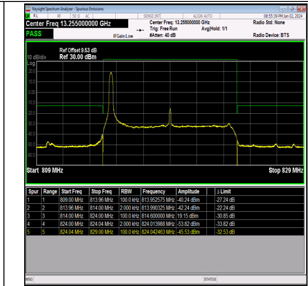
Band26_10MHz_16QAM_26740_1RB#0
