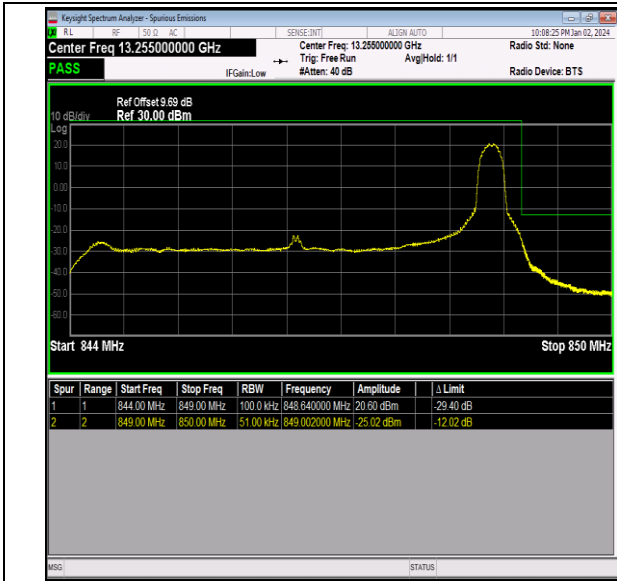
Band26_5MHz_QPSK_27015_1RB#24
