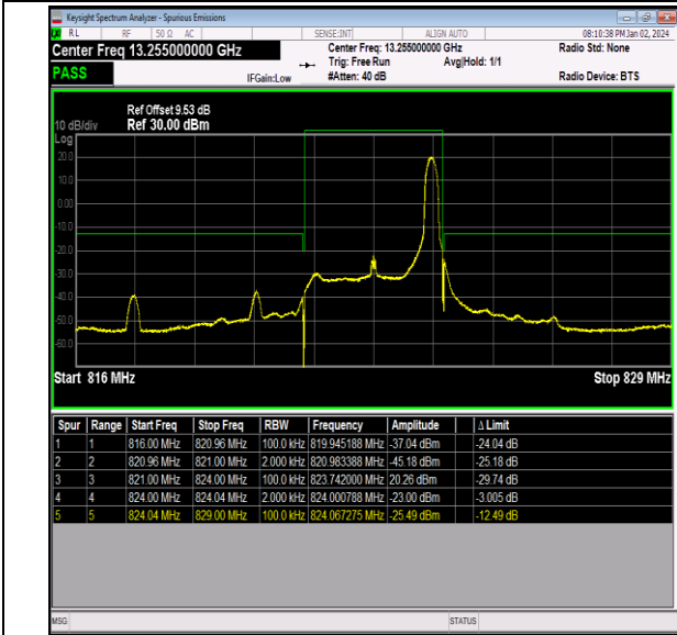
Band26_3MHz_QPSK_26775_1RB#14
