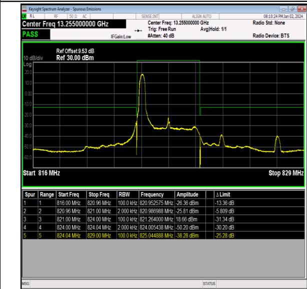
Band26_3MHz_16QAM_26775_1RB#0
