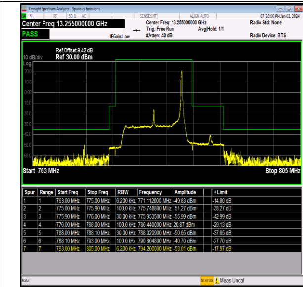
Band13_10MHz_QPSK_23230_1RB#49
