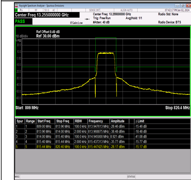
Band26_1.4MHz_16QAM_26697_6RB#0
