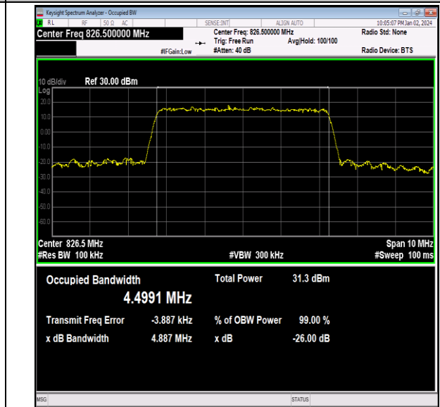
26(824-849)-5MHz-16QAM-26815-25RB#0-PASS
