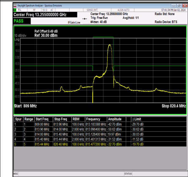
Band26_1.4MHz_QPSK_26697_1RB#5
