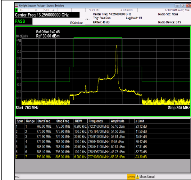
Band13_5MHz_16QAM_23255_1RB#24
