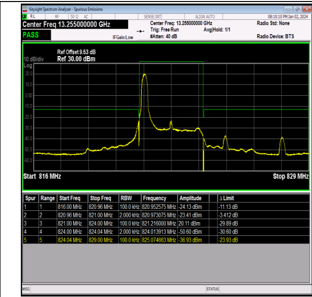
Band26_3MHz_QPSK_26775_1RB#0
