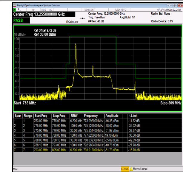
Band13_10MHz_16QAM_23230_1RB#0
