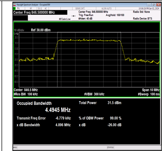
26(824-849)-5MHz-16QAM-27015-25RB#0-PASS
