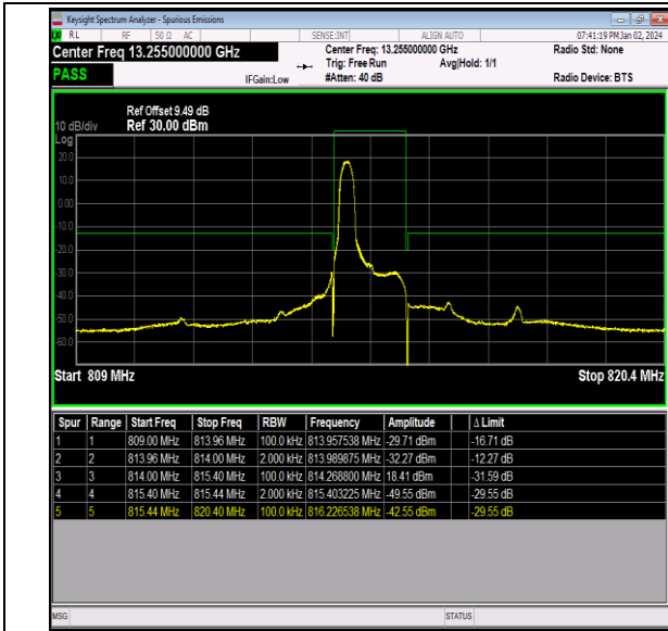
Band26_1.4MHz_16QAM_26697_1RB#0
