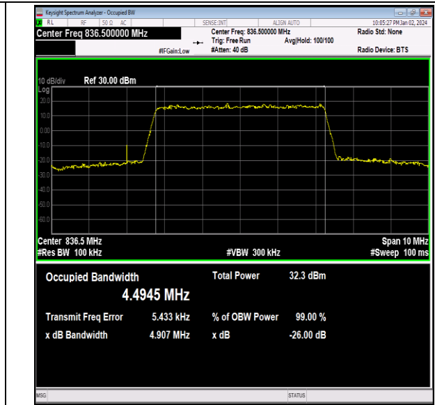
26(824-849)-5MHz-QPSK-26915-25RB#0-PASS
