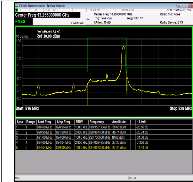
Band26_3MHz_16QAM_26775_1RB#14
