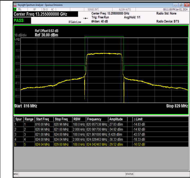
Band26_3MHz_QPSK_26775_15RB#0
