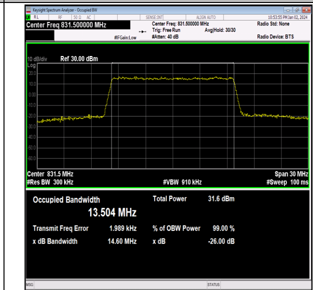
26(824-849)-15MHz-16QAM-26865-75RB#0-PASS
