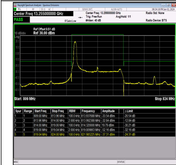
Band26_5MHz_QPSK_26715_1RB#0
