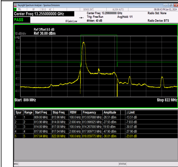
Band26_3MHz_QPSK_26705_1RB#0
