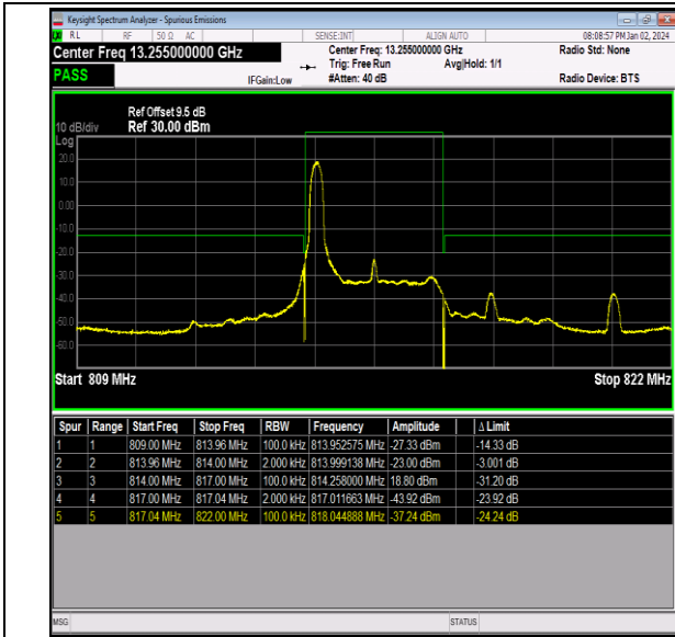
Band26_3MHz_16QAM_26705_1RB#0
