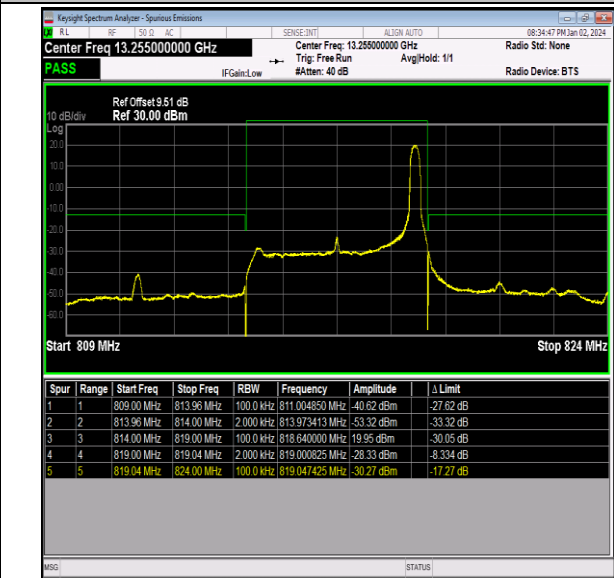
Band26_5MHz_QPSK_26715_1RB#24
