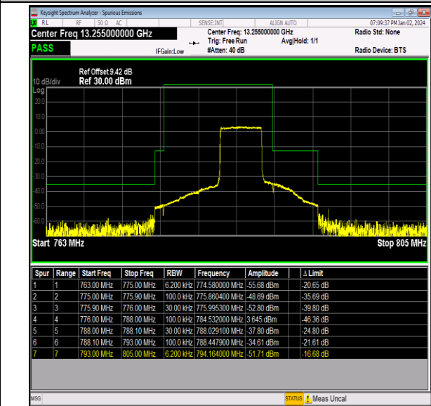
Band13_5MHz_16QAM_23255_25RB#0
