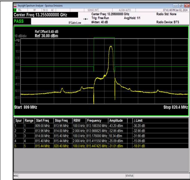
Band26_1.4MHz_16QAM_26697_1RB#5
