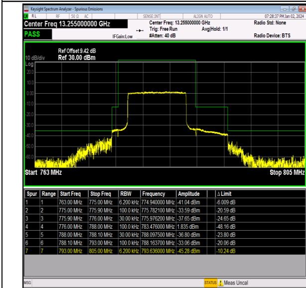
Band13_10MHz_QPSK_23230_50RB#0
