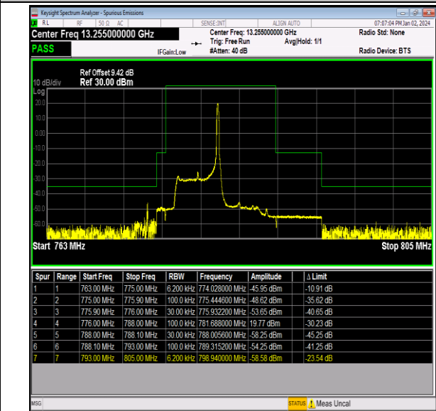
Band13_5MHz_16QAM_23205_1RB#24
