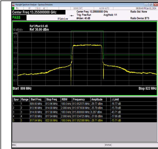
Band26_3MHz_QPSK_26705_15RB#0
