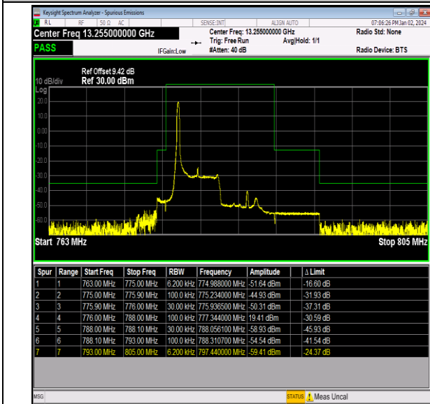
Band13_5MHz_16QAM_23205_1RB#0
