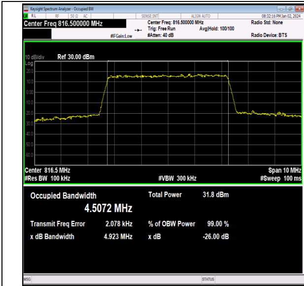
26(814-824)-5MHz-QPSK-26715-25RB#0-PASS
