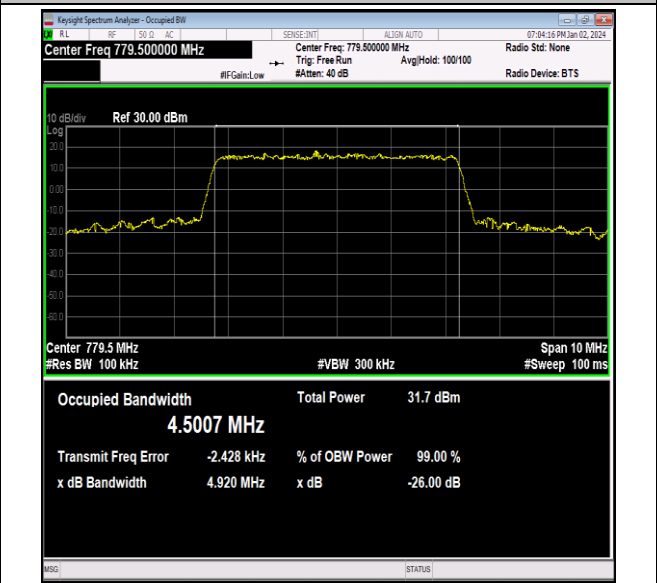
Band13-5MHz-16QAM-23205-25RB#0-PASS
