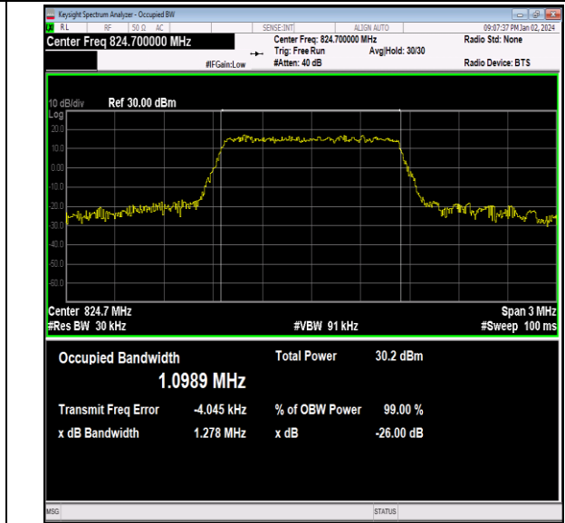
26(824-849)-1.4MHz-16QAM-26797-6RB#0-PASS
