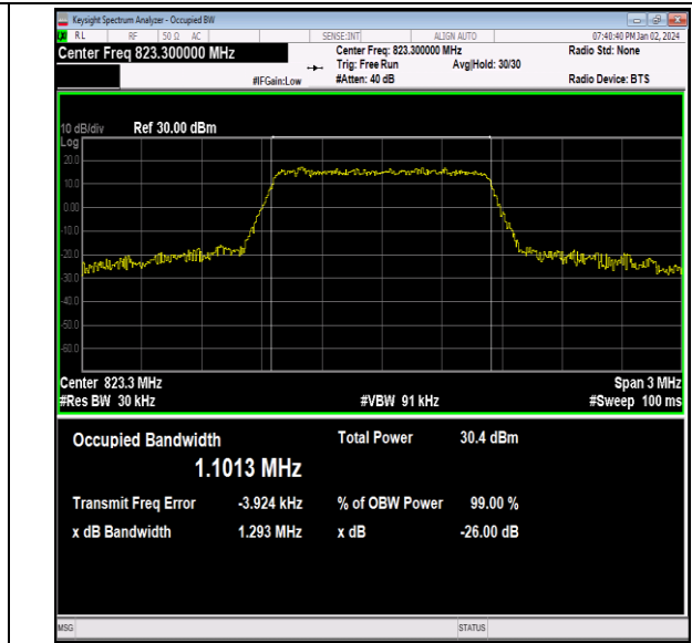
26(814-824)-1.4MHz-16QAM-26783-6RB#0-PASS
