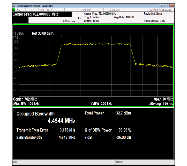
Band13-5MHz-QPSK-23230-25RB#0-PASS
