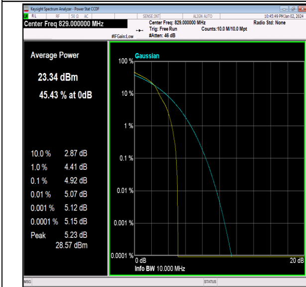
26(824-849)-10MHz-16QAM-26840-1RB#0-PASS
