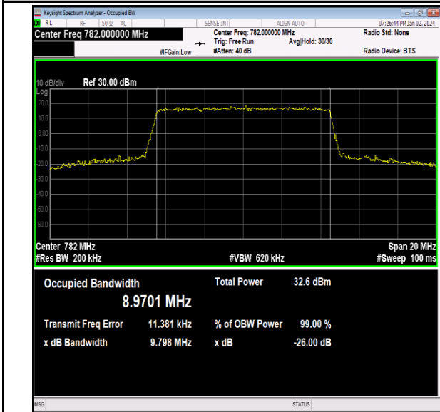
Band13-10MHz-QPSK-23230-50RB#0-PASS
