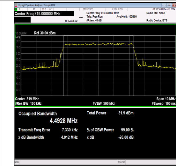
26(814-824)-5MHz-QPSK-26740-25RB#0-PASS
