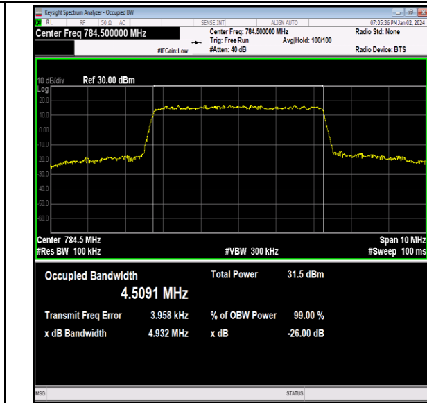
Band13-5MHz-16QAM-23255-25RB#0-PASS
