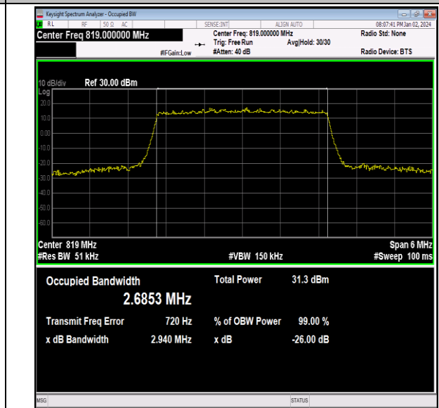
26(814-824)-3MHz-QPSK-26740-15RB#0-PASS
