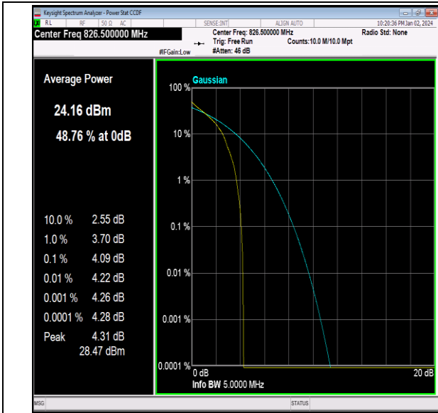
26(824-849)-5MHz-QPSK-26815-1RB#0-PASS
