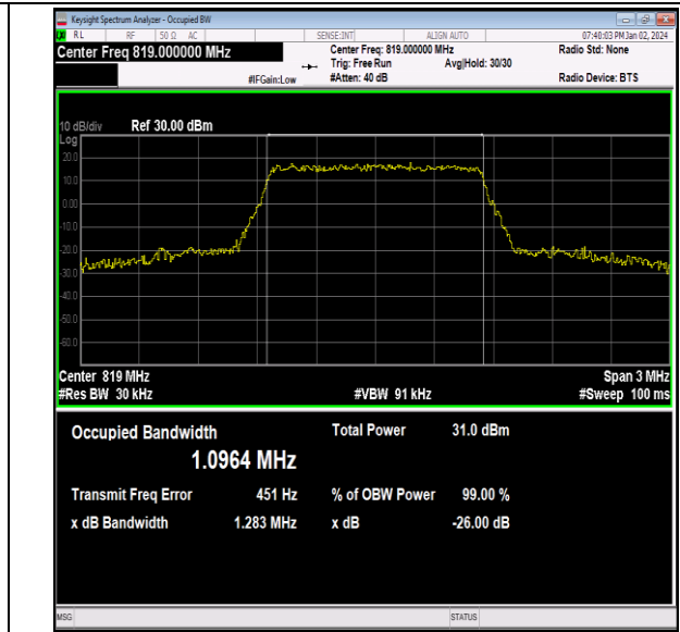
26(814-824)-1.4MHz-QPSK-26740-6RB#0-PASS
