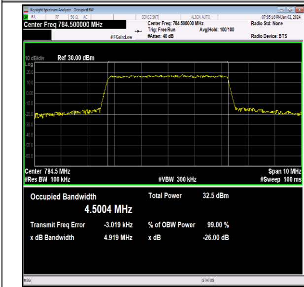
Band13-5MHz-QPSK-23255-25RB#0-PASS
