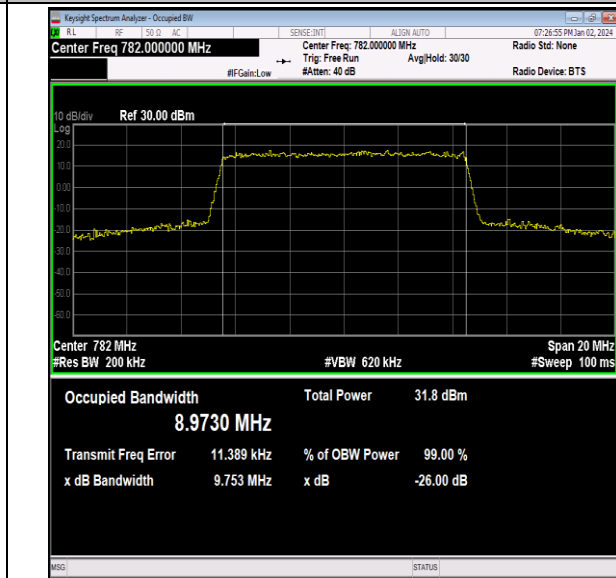
Band13-10MHz-16QAM-23230-50RB#0-PASS
