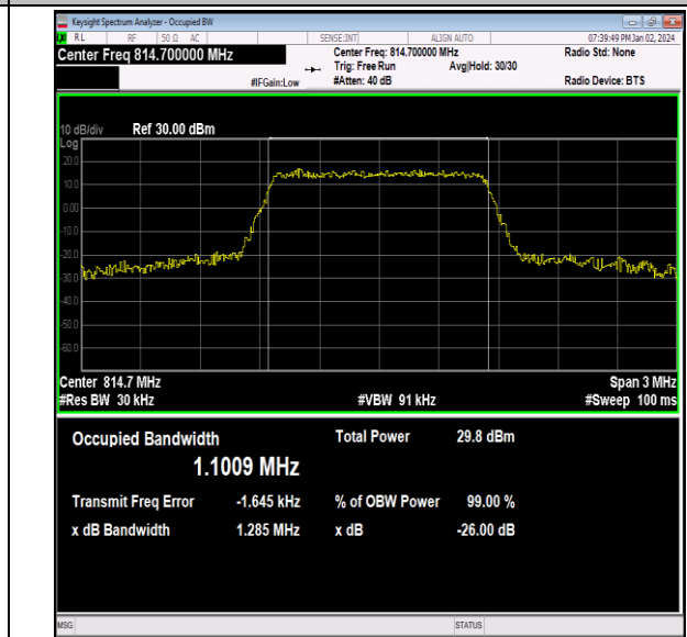
26(814-824)-1.4MHz-16QAM-26697-6RB#0-PASS
