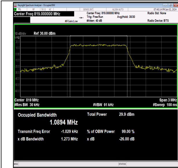
26(814-824)-1.4MHz-16QAM-26740-6RB#0-PASS
