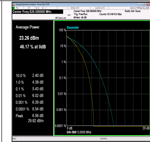
26(824-849)-5MHz-QPSK-26815-25RB#0-PASS
