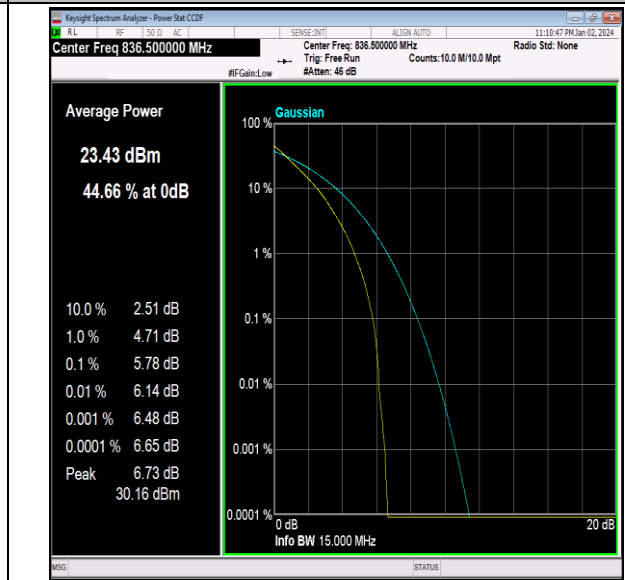
26(824-849)-15MHz-QPSK-26915-75RB#0-PASS
