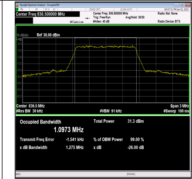
26(824-849)-1.4MHz-QPSK-26915-6RB#0-PASS
