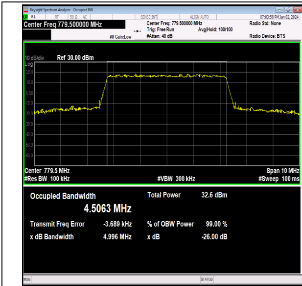
Band13-5MHz-QPSK-23205-25RB#0-PASS
