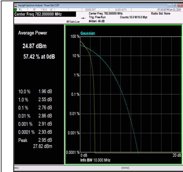
Band13-10MHz-QPSK-23230-1RB#0-PASS
