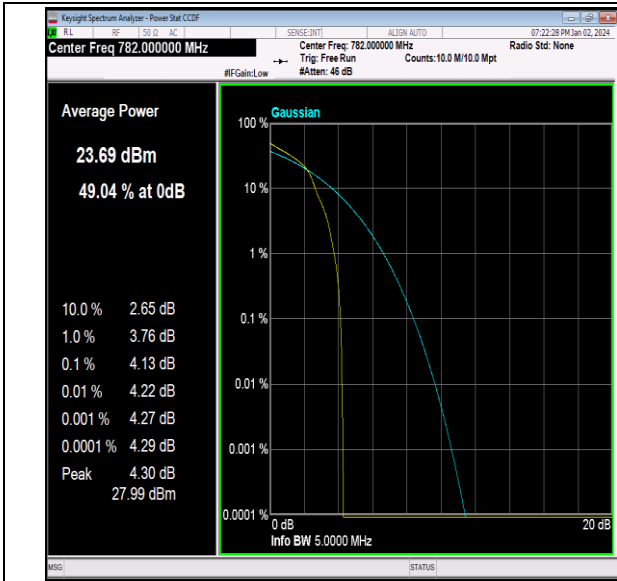
Band13-5MHz-16QAM-23230-1RB#0-PASS
