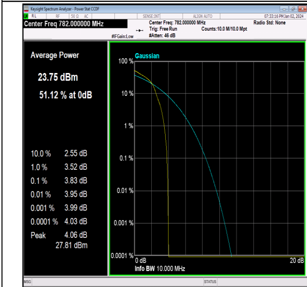
Band13-10MHz-16QAM-23230-1RB#0-PASS
