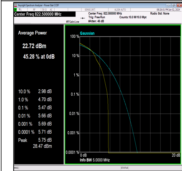
26(814-824)-3MHz-16QAM-26775-1RB#0-PASS
