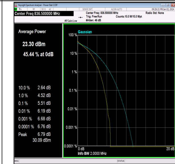
26(824-849)-1.4MHz-QPSK-26915-6RB#0-PASS
