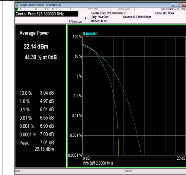
26(814-824)-1.4MHz-16QAM-26783-6RB#0-PASS
