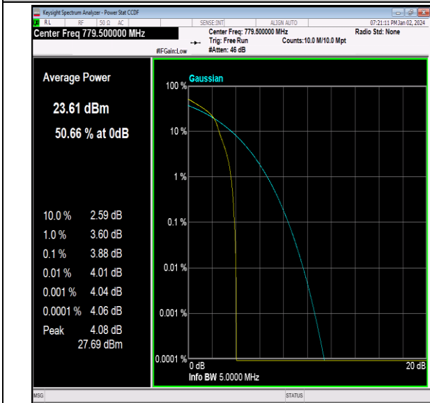
Band13-5MHz-16QAM-23205-1RB#0-PASS
