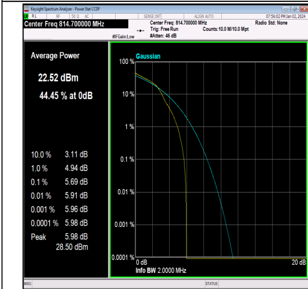
26(814-824)-1.4MHz-16QAM-26697-1RB#0-PASS
