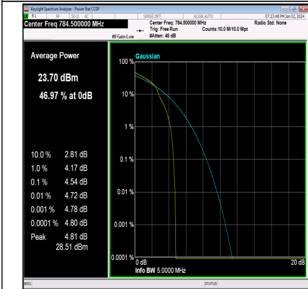
Band13-5MHz-16QAM-23255-1RB#0-PASS
