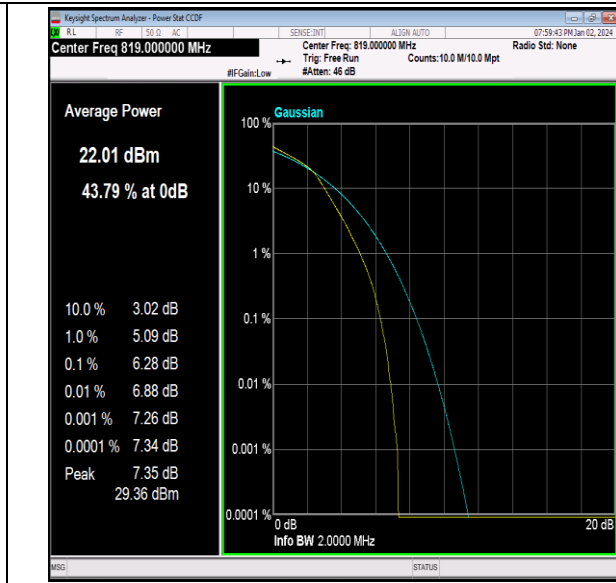
26(814-824)-1.4MHz-16QAM-26740-6RB#0-PASS
