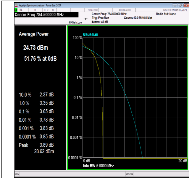
Band13-5MHz-QPSK-23255-1RB#0-PASS
