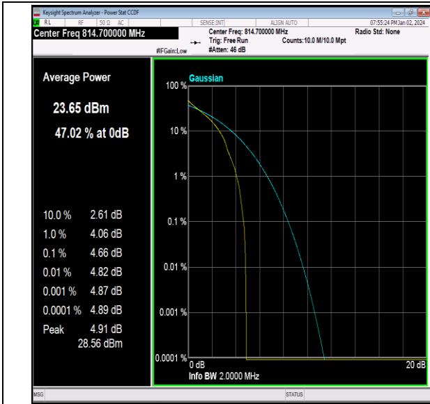
26(814-824)-1.4MHz-QPSK-26697-1RB#0-PASS
