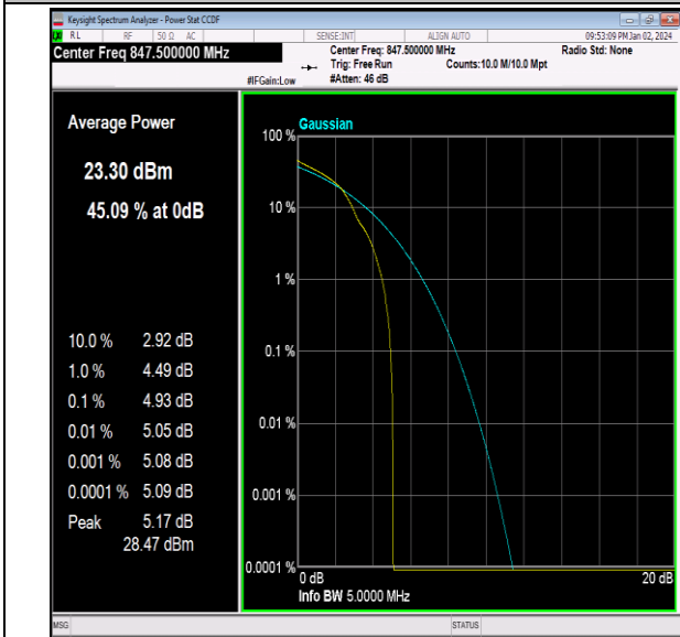
26(824-849)-3MHz-16QAM-27025-1RB#0-PASS
