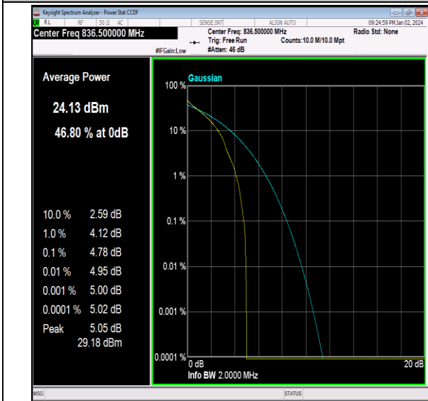
26(824-849)-1.4MHz-QPSK-26915-1RB#0-PASS
