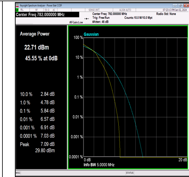
Band13-5MHz-16QAM-23230-25RB#0-PASS
