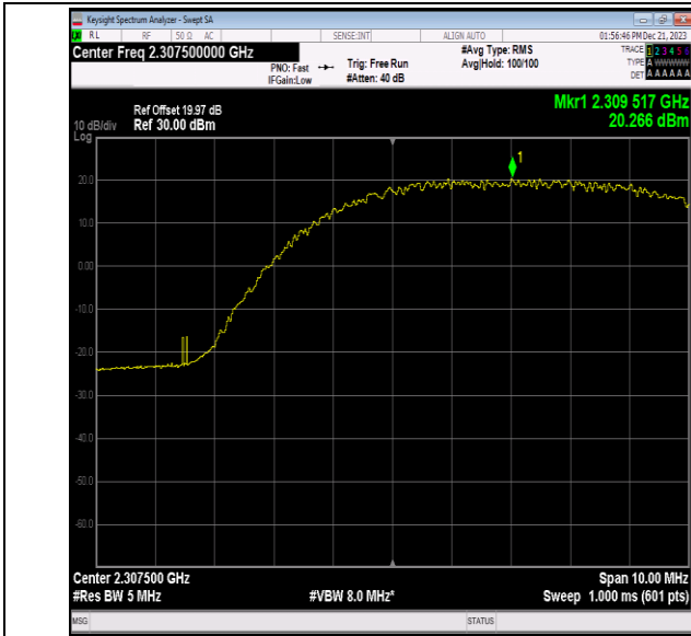
40(2305-2315)-5MHz-64QAM-38725-1RB#24-PASS
