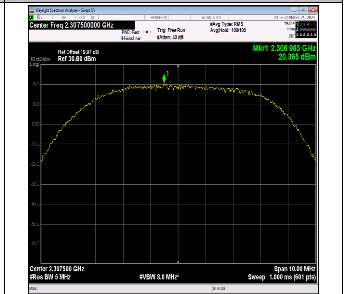
40(2305-2315)-5MHz-64QAM-38725-1RB#12-PASS
