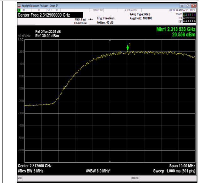
40(2305-2315)-5MHz-16QAM-38775-1RB#24-PASS
