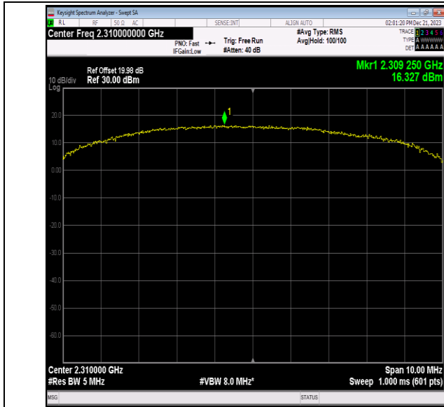
40(2305-2315)-5MHz-64QAM-38750-25RB#0-PASS
