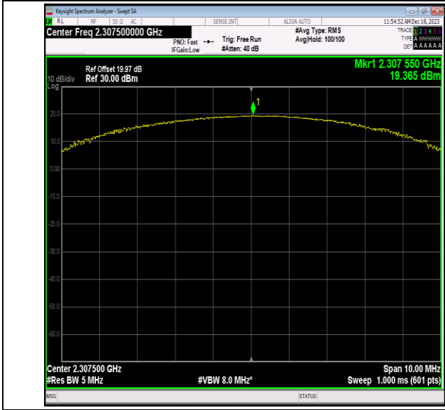
40(2305-2315)-5MHz-64QAM-38725-25RB#12-PASS
