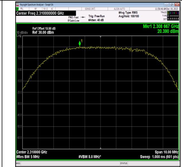
40(2305-2315)-5MHz-16QAM-38750-1RB#49-PASS
