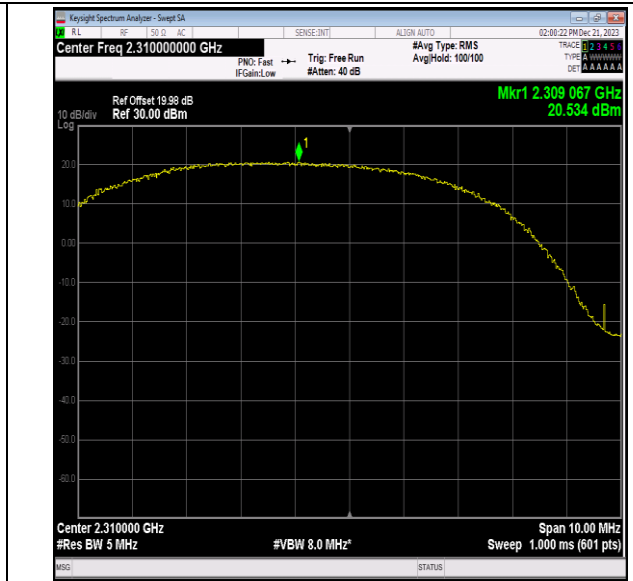
40(2305-2315)-5MHz-16QAM-38750-12RB#6-PASS
