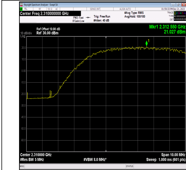
40(2305-2315)-5MHz-16QAM-38750-1RB#24-PASS
