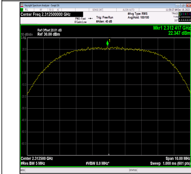
40(2305-2315)-5MHz-16QAM-38775-1RB#49-PASS
