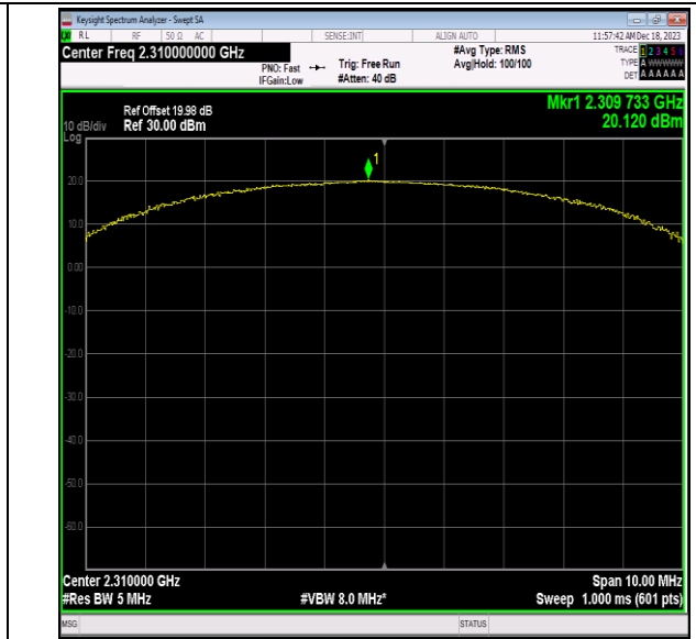
40(2305-2315)-5MHz-64QAM-38750-25RB#12-PASS
