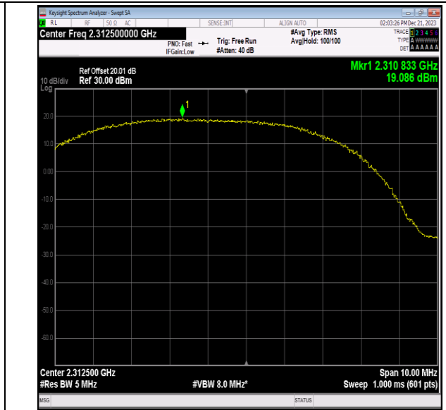
40(2305-2315)-5MHz-64QAM-38775-12RB#6-PASS
