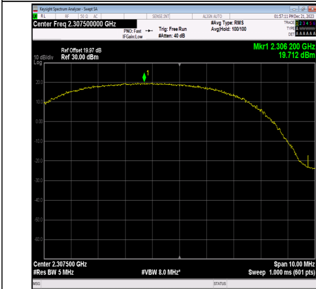
40(2305-2315)-5MHz-64QAM-38725-12RB#0-PASS
