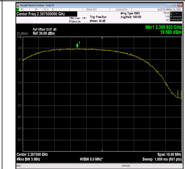
40(2305-2315)-5MHz-16QAM-38725-12RB#11-PASS
