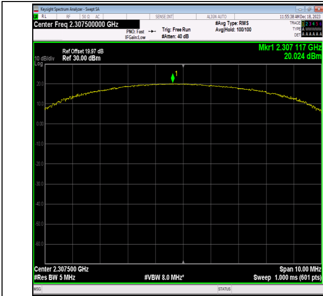
40(2305-2315)-5MHz-64QAM-38725-50RB#0-PASS
