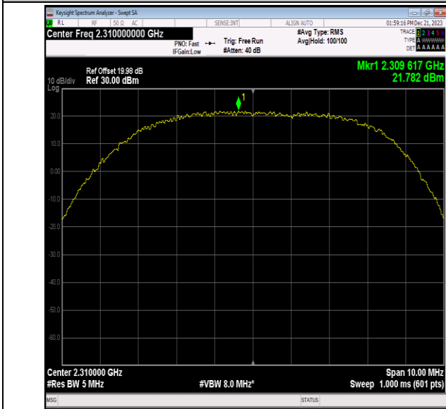
40(2305-2315)-5MHz-64QAM-38750-1RB#12-PASS
