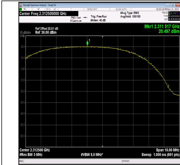
40(2305-2315)-5MHz-16QAM-38775-12RB#6-PASS
