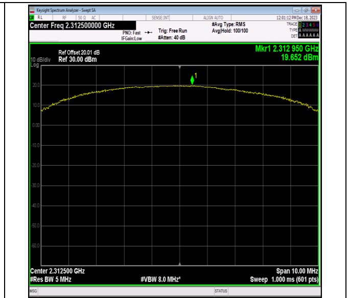
40(2305-2315)-5MHz-16QAM-38775-50RB#0-PASS
