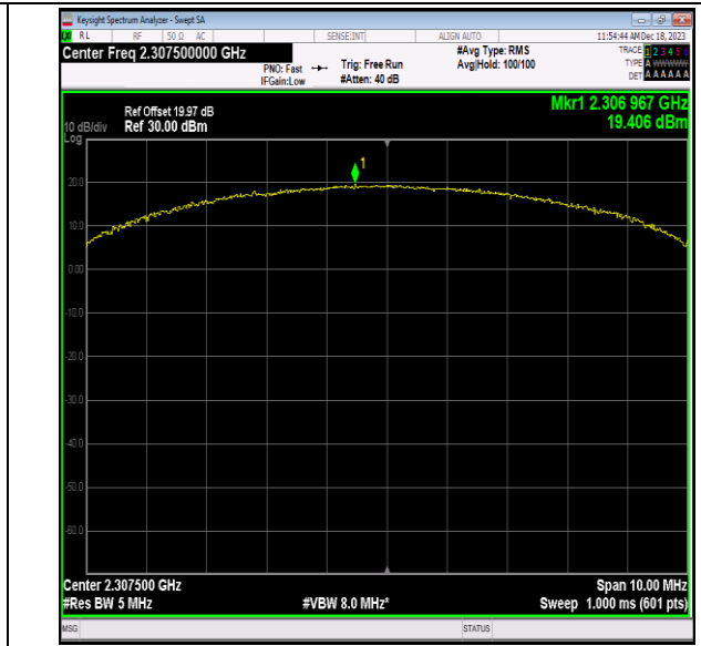
40(2305-2315)-5MHz-16QAM-38725-25RB#12-PASS
