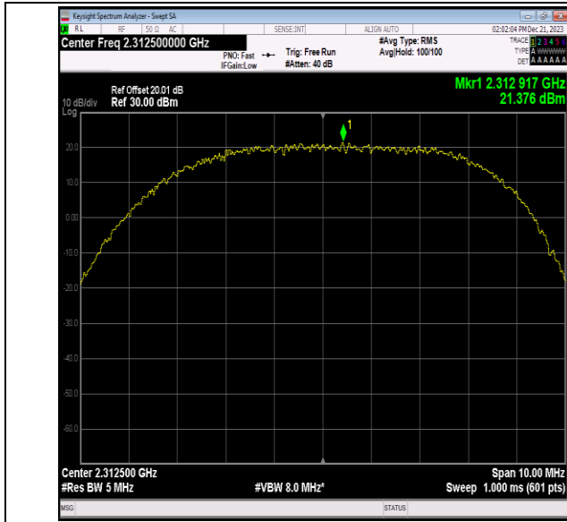
40(2305-2315)-5MHz-16QAM-38775-1RB#12-PASS
