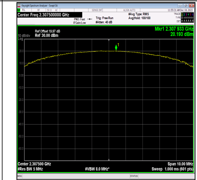
40(2305-2315)-5MHz-16QAM-38725-50RB#0-PASS
