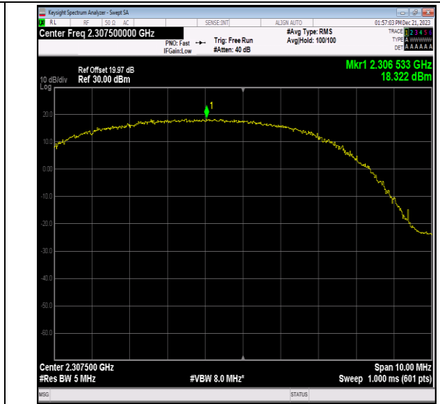
40(2305-2315)-5MHz-16QAM-38725-12RB#0-PASS
