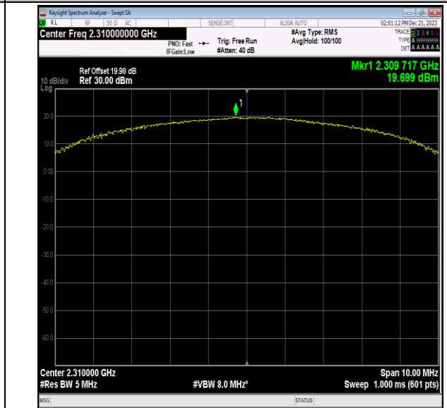
40(2305-2315)-5MHz-16QAM-38750-25RB#0-PASS
