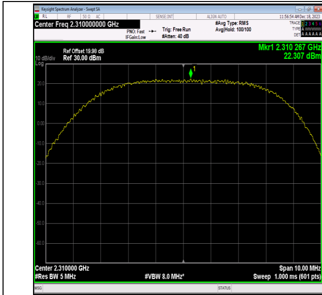
40(2305-2315)-5MHz-64QAM-38750-1RB#49-PASS
