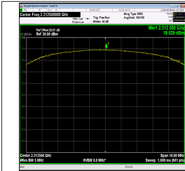
40(2305-2315)-5MHz-16QAM-38775-25RB#25-PASS
