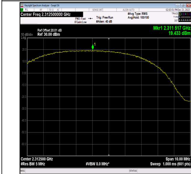
40(2305-2315)-5MHz-64QAM-38775-12RB#11-PASS
