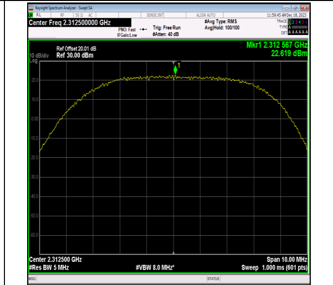
40(2305-2315)-5MHz-64QAM-38775-1RB#49-PASS
