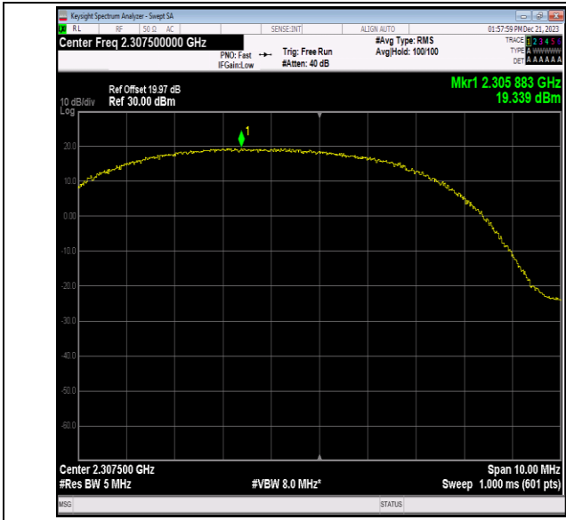
40(2305-2315)-5MHz-64QAM-38725-12RB#11-PASS
