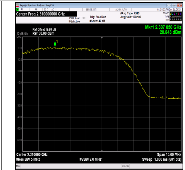
40(2305-2315)-5MHz-64QAM-38750-1RB#0-PASS
