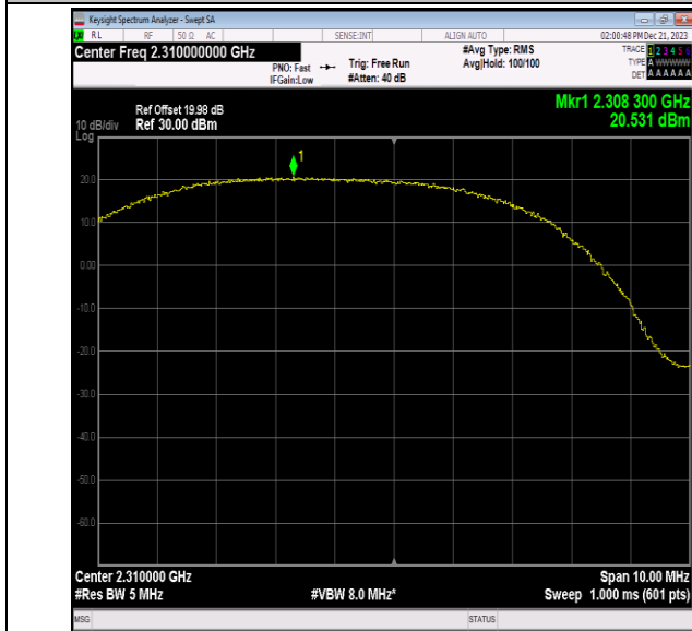
40(2305-2315)-5MHz-16QAM-38750-12RB#11-PASS
