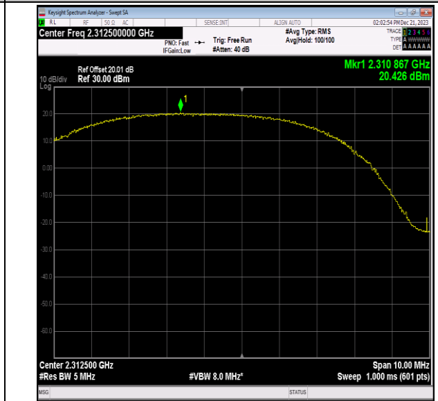
40(2305-2315)-5MHz-16QAM-38775-12RB#0-PASS
