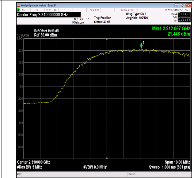
40(2305-2315)-5MHz-64QAM-38750-1RB#24-PASS
