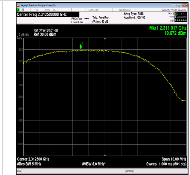
40(2305-2315)-5MHz-16QAM-38775-12RB#11-PASS
