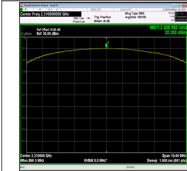
40(2305-2315)-5MHz-64QAM-38750-25RB#25-PASS
