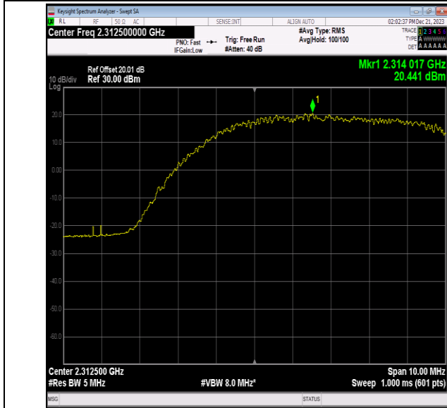
40(2305-2315)-5MHz-64QAM-38775-1RB#24-PASS
