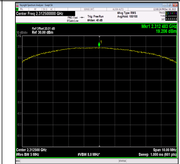
40(2305-2315)-5MHz-16QAM-38775-25RB#12-PASS
