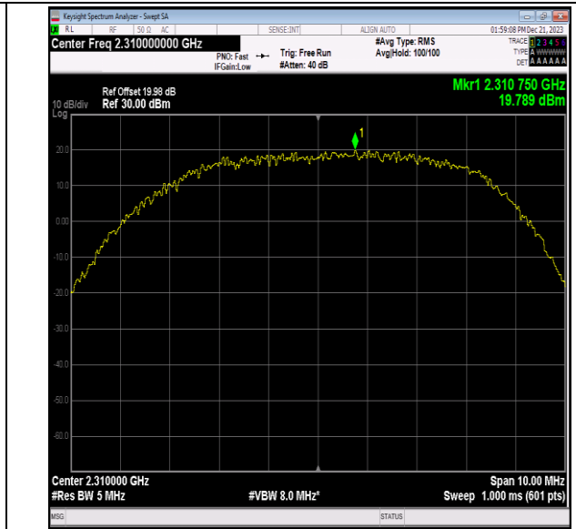
40(2305-2315)-5MHz-16QAM-38750-1RB#12-PASS
