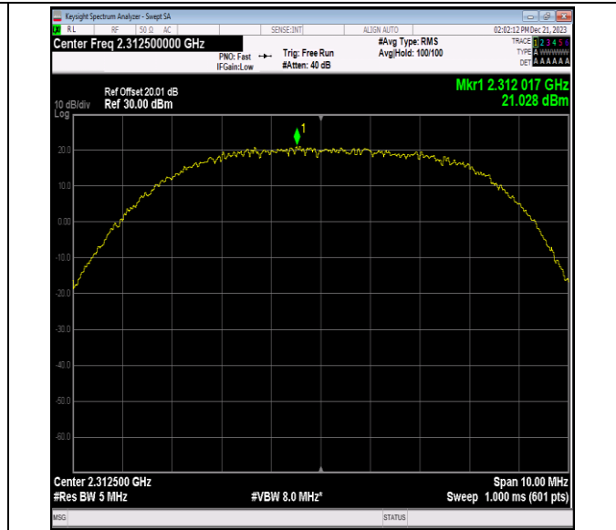
40(2305-2315)-5MHz-64QAM-38775-1RB#12-PASS
