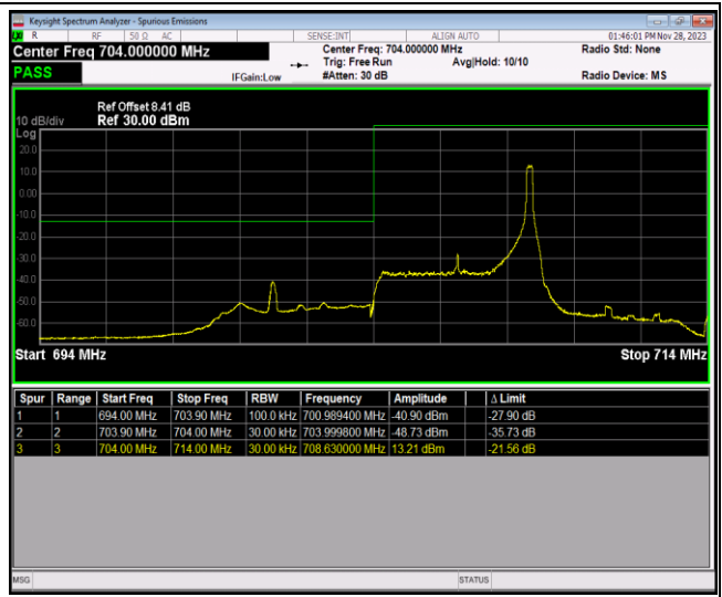
Band17-5MHz-64QAM-23825-1RB#0
