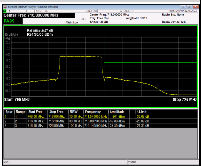
Band17-10MHz-QPSK-23780-1RB#49
