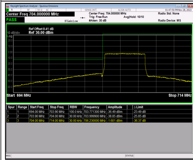
Band17-5MHz-64QAM-23825-1RB#24
