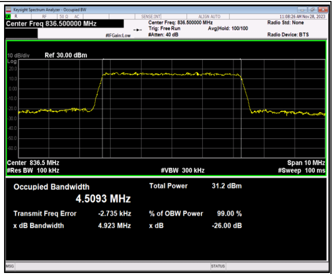
Band5-5MHz-16QAM-20425-25RB#0
