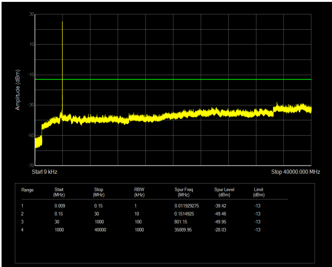
n77(3700-3980) SCS=30kHz DFT_QPSK BW=100MHz Channel=650000 RB=270@0
