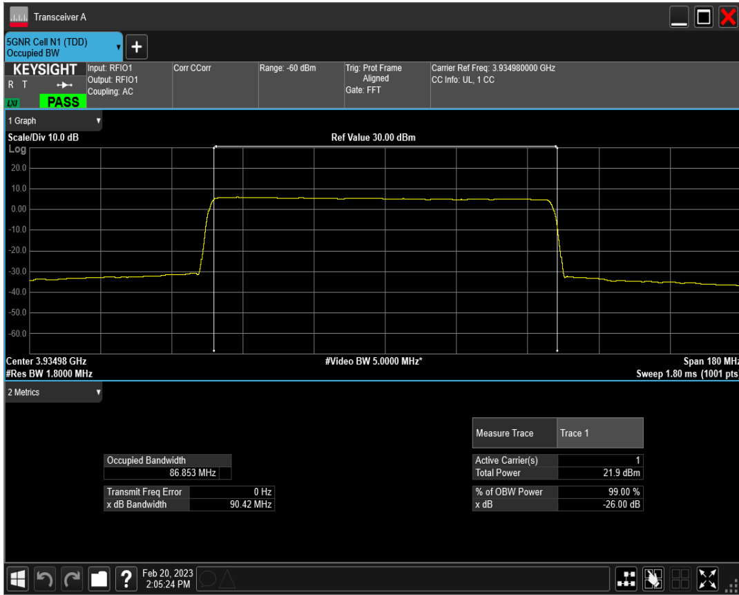
n77(3700-3980) SCS=30kHz CP_QPSK BW=90MHz Channel=662332 RB=245@0
