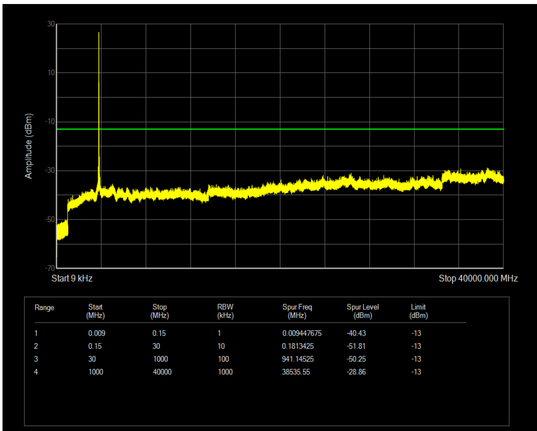
n77(3700-3980) SCS=30kHz DFT_QPSK BW=100MHz Channel=656000 RB=1@272
