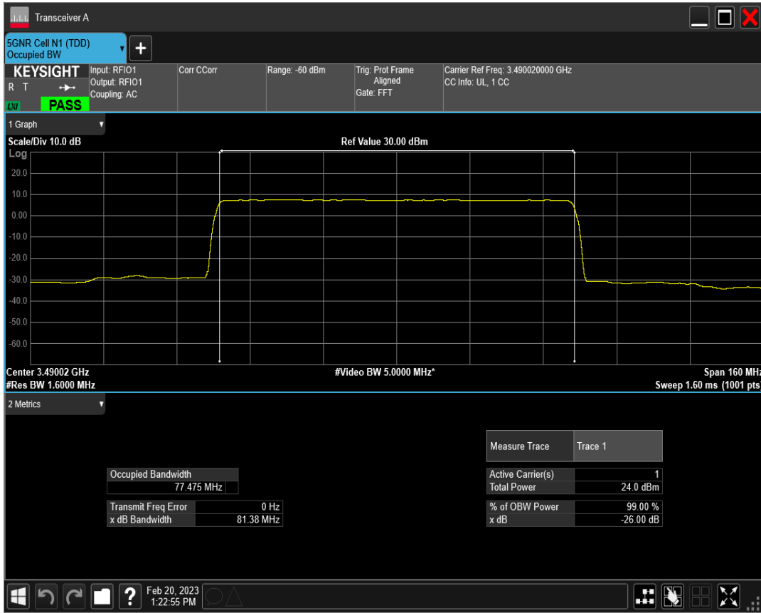
n77(3450-3550) SCS=30kHz CP_QPSK BW=80MHz Channel=632668 RB=217@0
