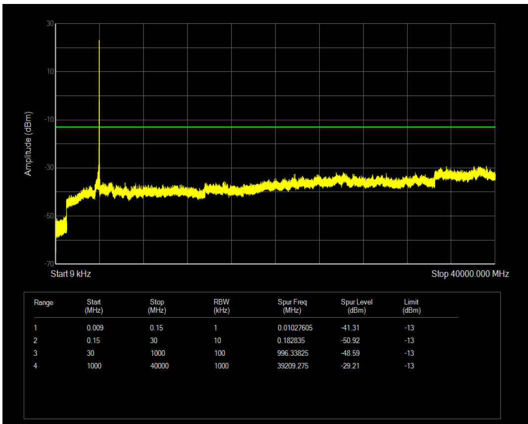
n77(3700-3980) SCS=15kHz DFT_QPSK BW=50MHz Channel=663666 RB=1@269
