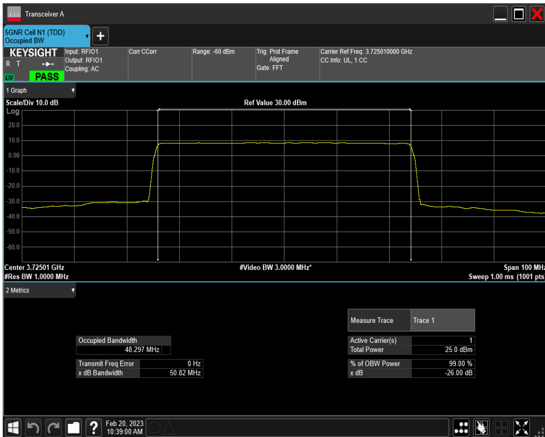
n77(3700-3980) SCS=15kHz DFT_QAM16 BW=50MHz Channel=648334 RB=270@0
