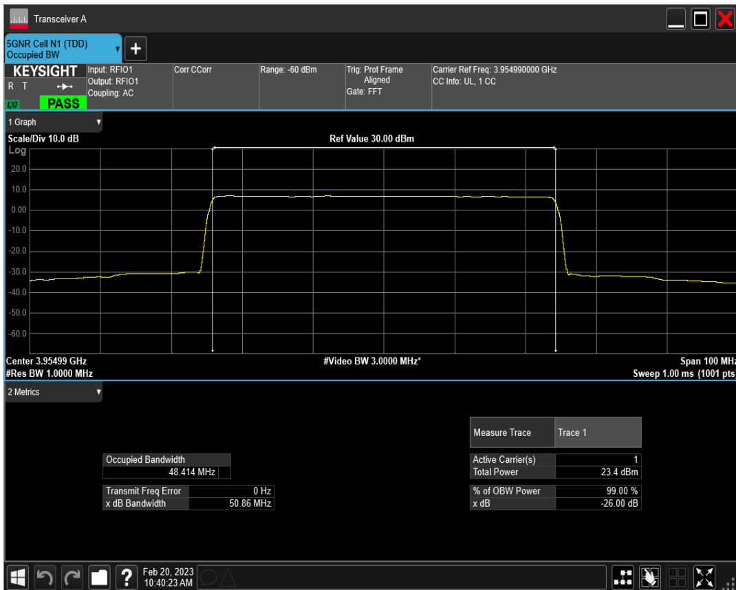
n77(3700-3980) SCS=15kHz DFT_QAM256 BW=50MHz Channel=663666 RB=270@0
