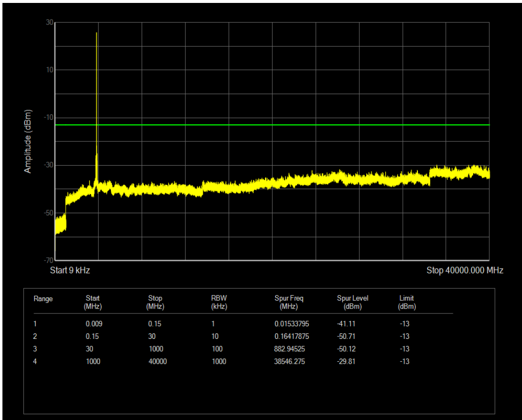
n77(3700-3980) SCS=15kHz DFT_QPSK BW=10MHz Channel=656000 RB=1@51
