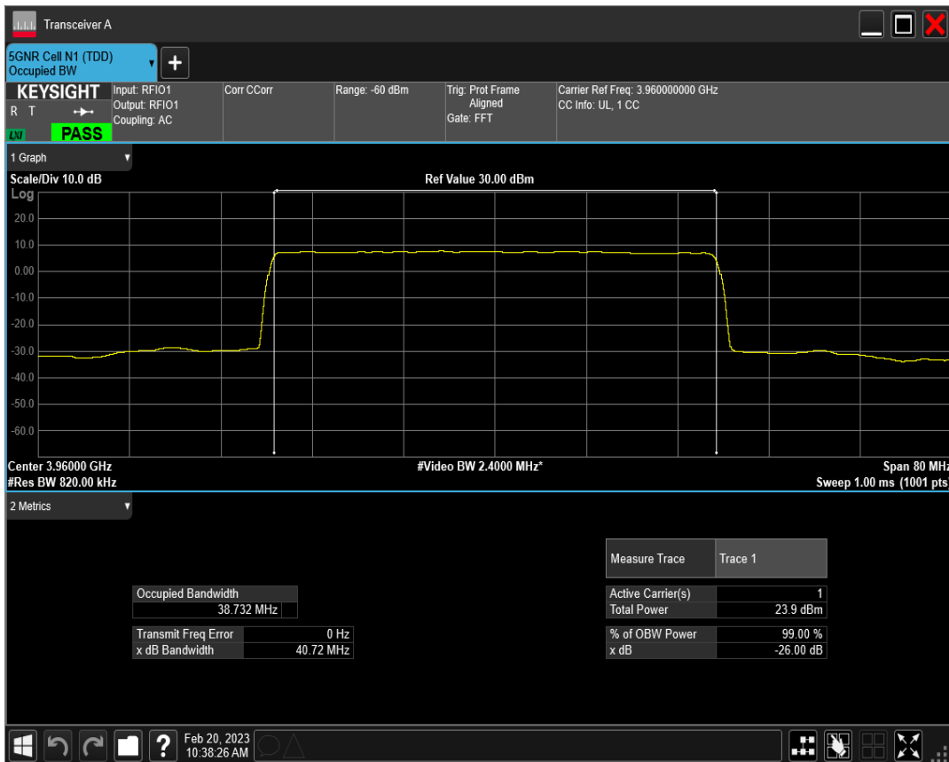
n77(3700-3980) SCS=15kHz DFT_QAM64 BW=40MHz Channel=664000 RB=216@0
