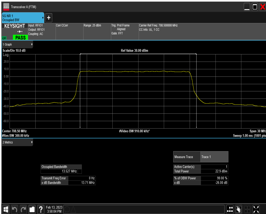
n12 SCS=30kHz DFT_QAM16 BW=15MHz Channel=141700 RB=36@0
