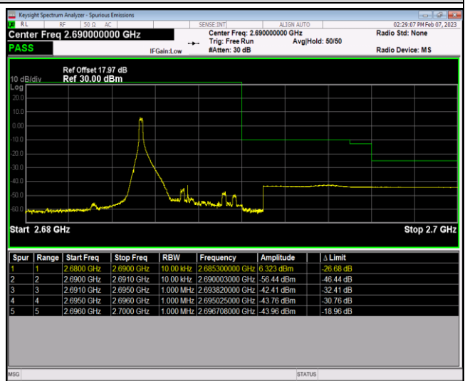
Band41-5MHz-64QAM-41565-25RB#0
