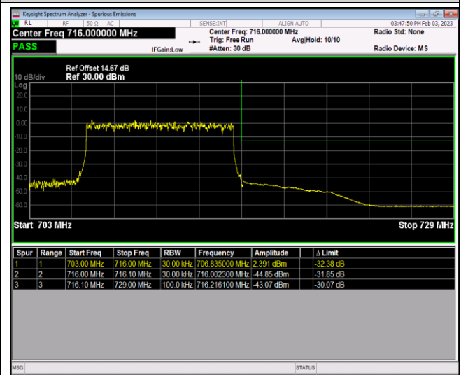
Band17-10MHz-16QAM-23780-1RB#49
