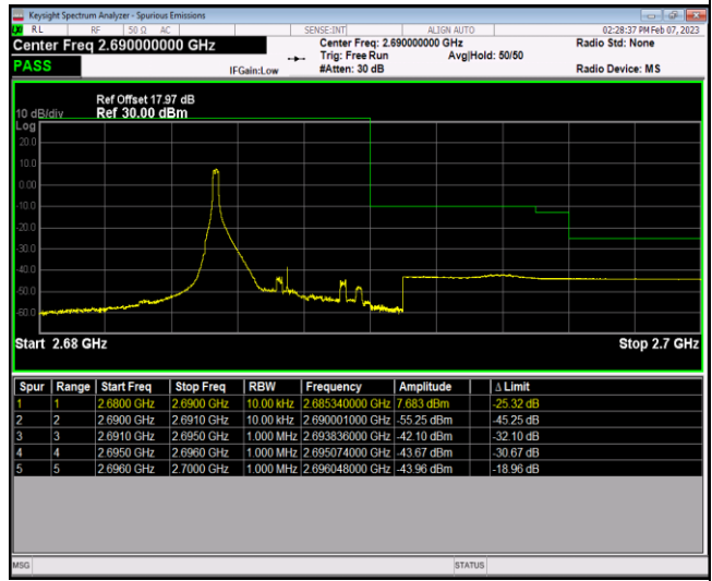
Band41-5MHz-16QAM-41565-25RB#0
