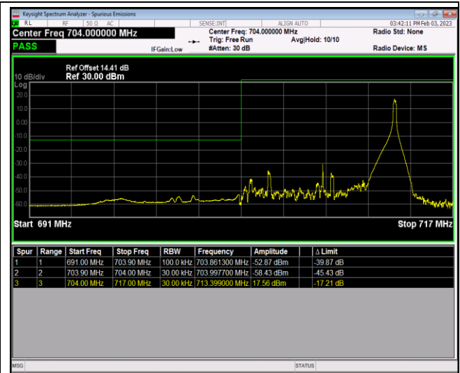
Band17-10MHz-QPSK-23800-1RB#0
