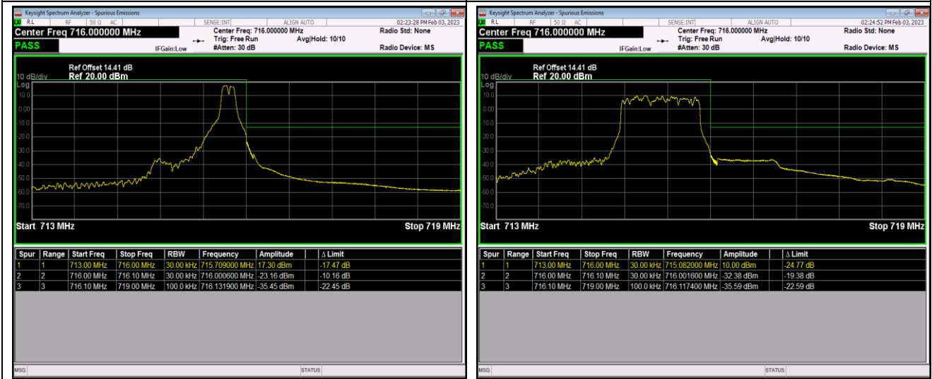
Band12-1.4MHz-16QAM-23017-1RB#0
