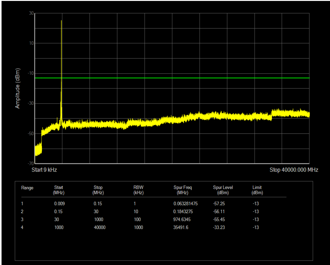
n77(3700-3980) SCS=30kHz DFT_QPSK BW=100MHz Channel=662000 RB=270@0
