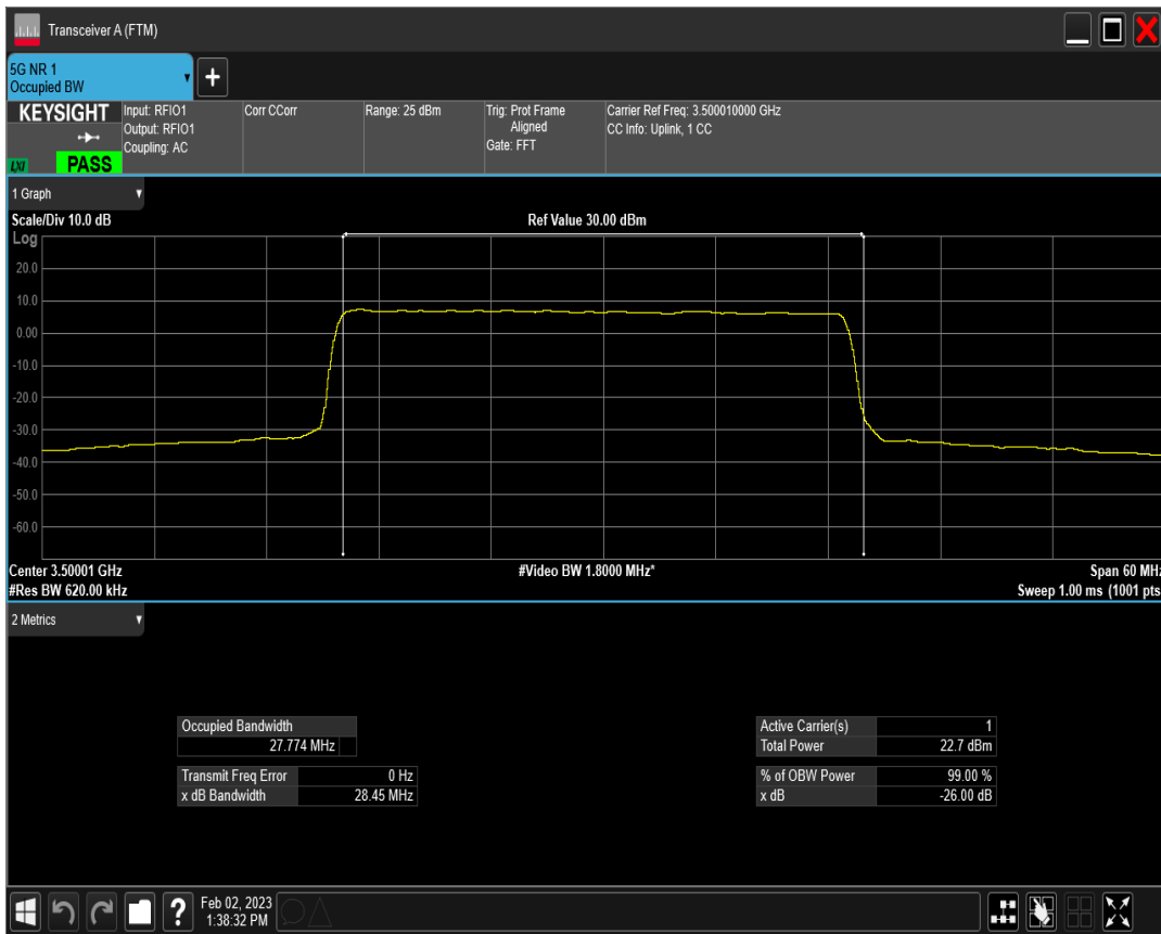
n77(3450-3550) SCS=30kHz CP_QPSK BW=30MHz Channel=633334 RB=78@0
