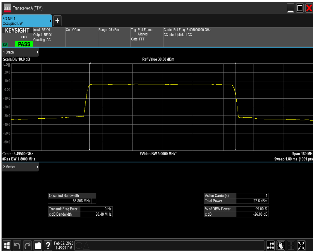
n77(3450-3550) SCS=30kHz CP_QPSK BW=90MHz Channel=633000 RB=245@0
