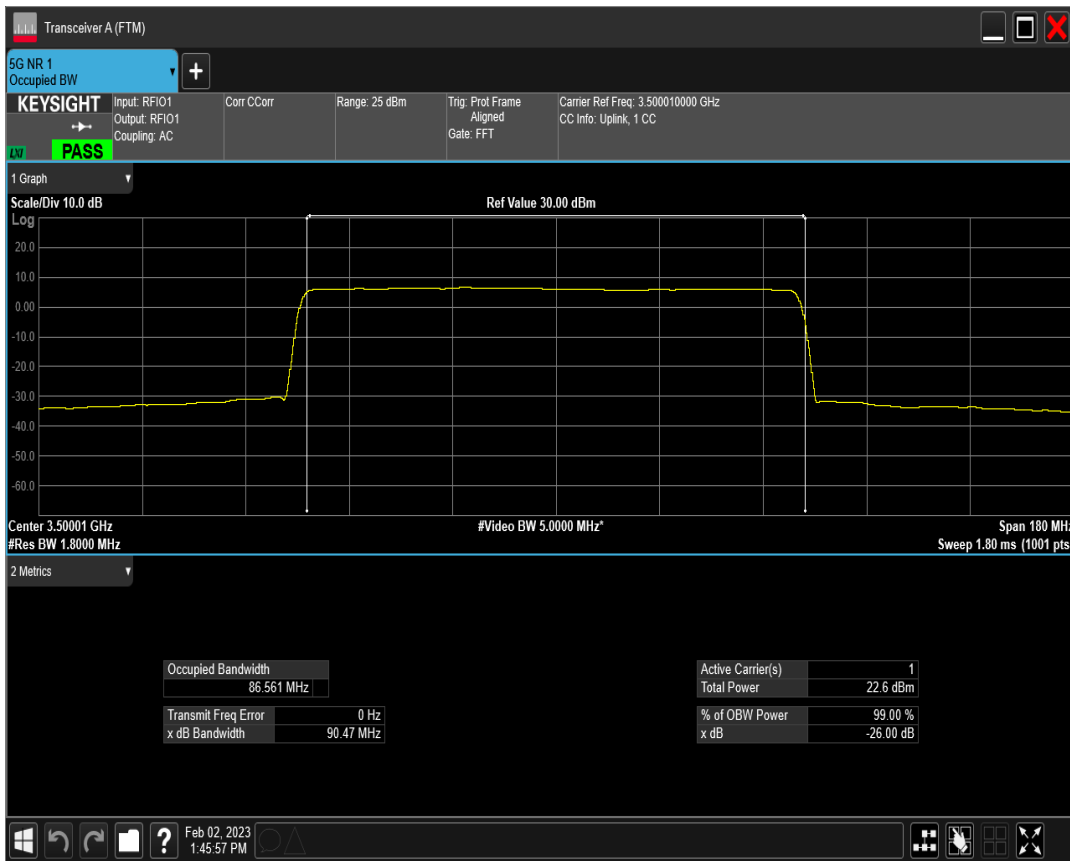
n77(3450-3550) SCS=30kHz CP_QPSK BW=90MHz Channel=633334 RB=245@0
