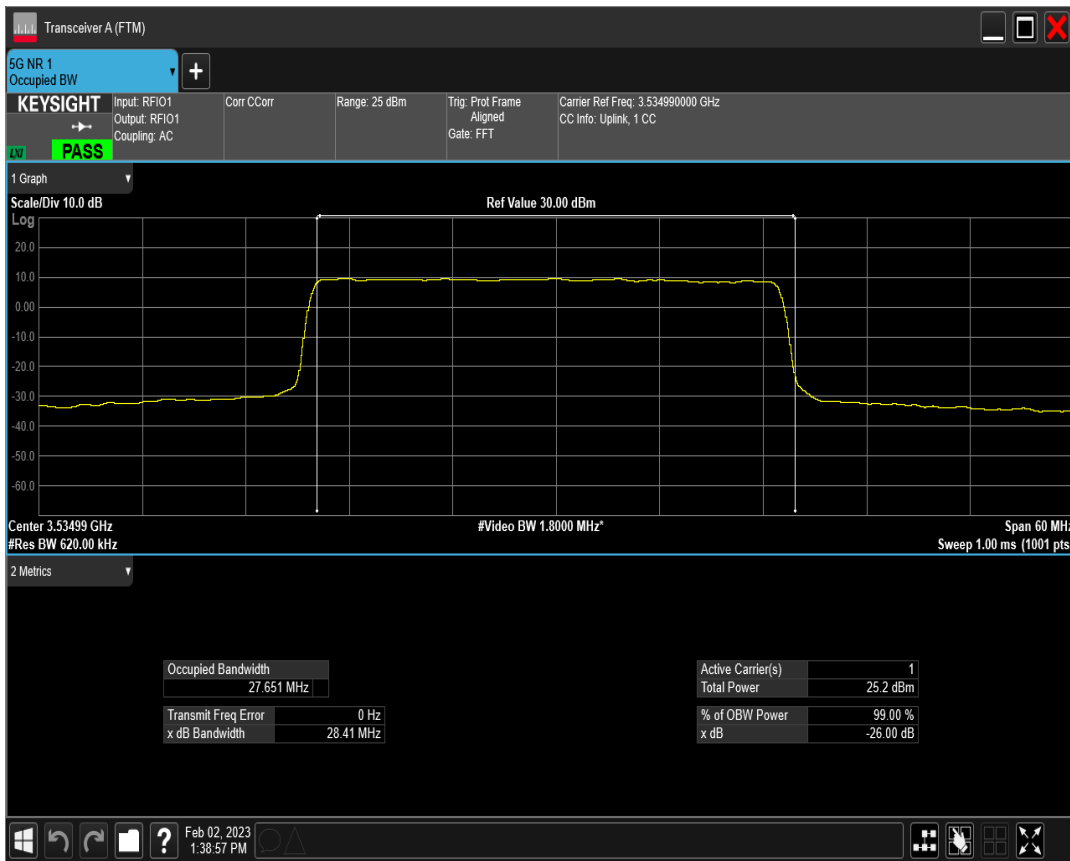
n77(3450-3550) SCS=30kHz DFT_QAM64 BW=30MHz Channel=635666 RB=75@0
