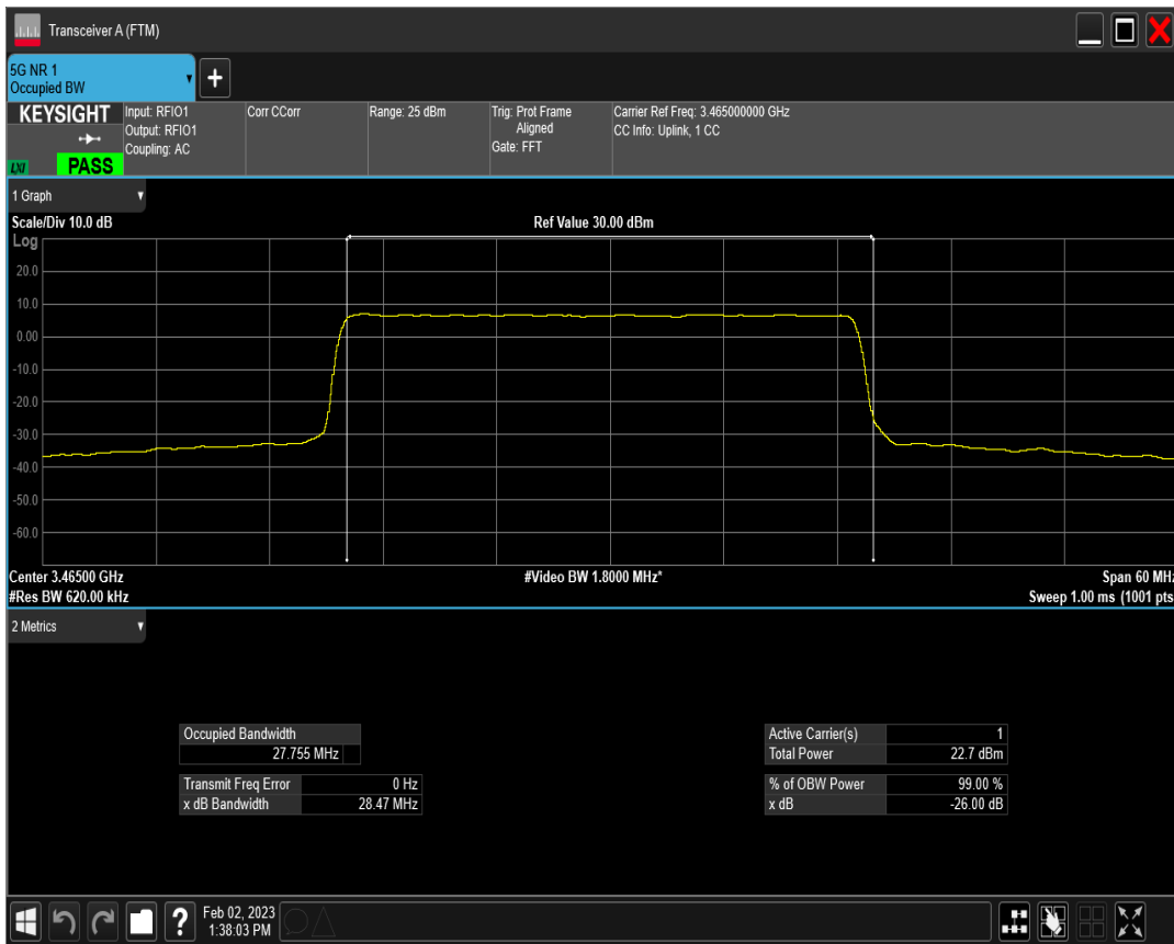
n77(3450-3550) SCS=30kHz CP_QPSK BW=30MHz Channel=631000 RB=78@0
