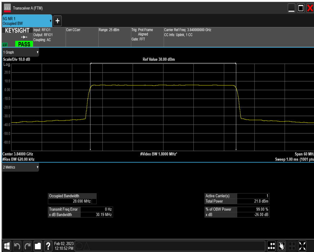
n77(3700-3980) SCS=15kHz CP_QPSK BW=30MHz Channel=656000 RB=160@0
