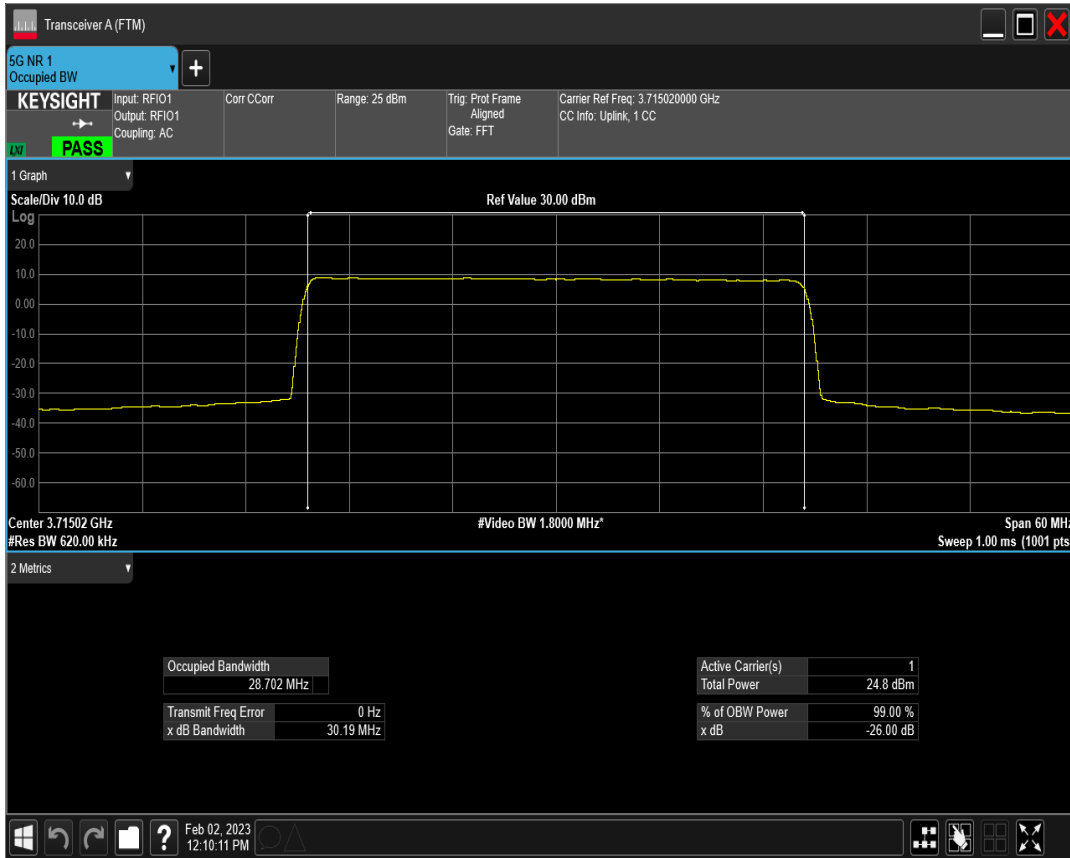
n77(3700-3980) SCS=15kHz DFT_QAM64 BW=30MHz Channel=647668 RB=160@0
