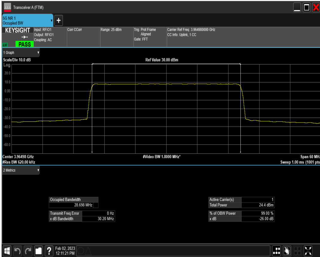
n77(3700-3980) SCS=15kHz DFT_QAM64 BW=30MHz Channel=664332 RB=160@0
