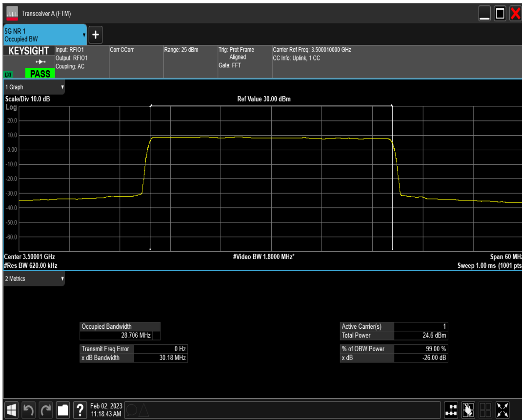
n77(3450-3550) SCS=15kHz DFT_QAM64 BW=30MHz Channel=633334 RB=160@0
