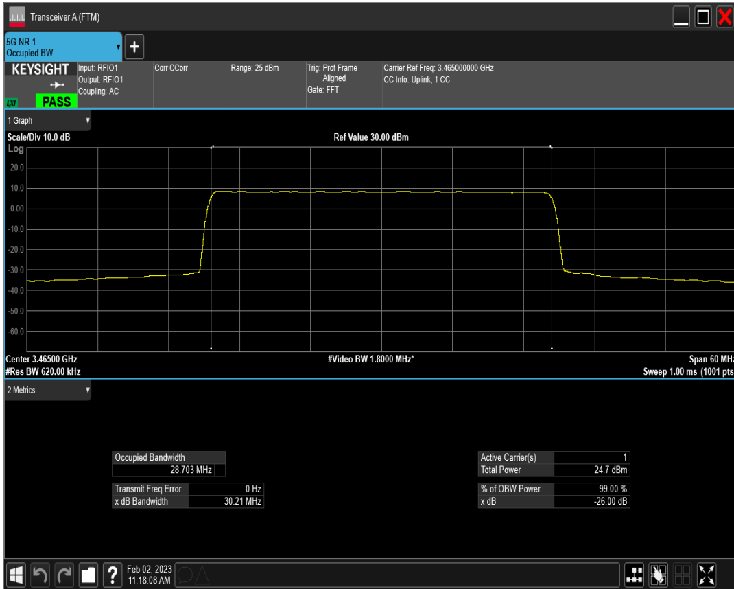
n77(3450-3550) SCS=15kHz DFT_QAM64 BW=30MHz Channel=631000 RB=160@0
