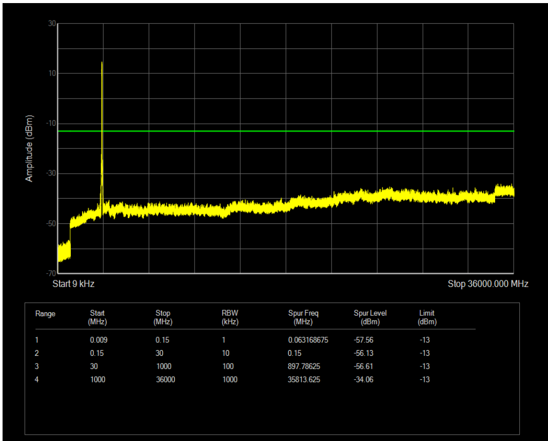
n77(3450-3550) SCS=15kHz DFT_QPSK BW=50MHz Channel=633334 RB=1 @0
