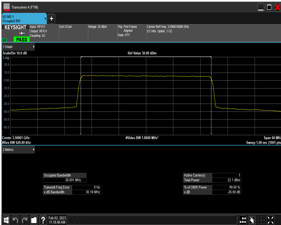
n77(3450-3550) SCS=15kHz CP_QPSK BW=30MHz Channel=633334 RB=160@0
