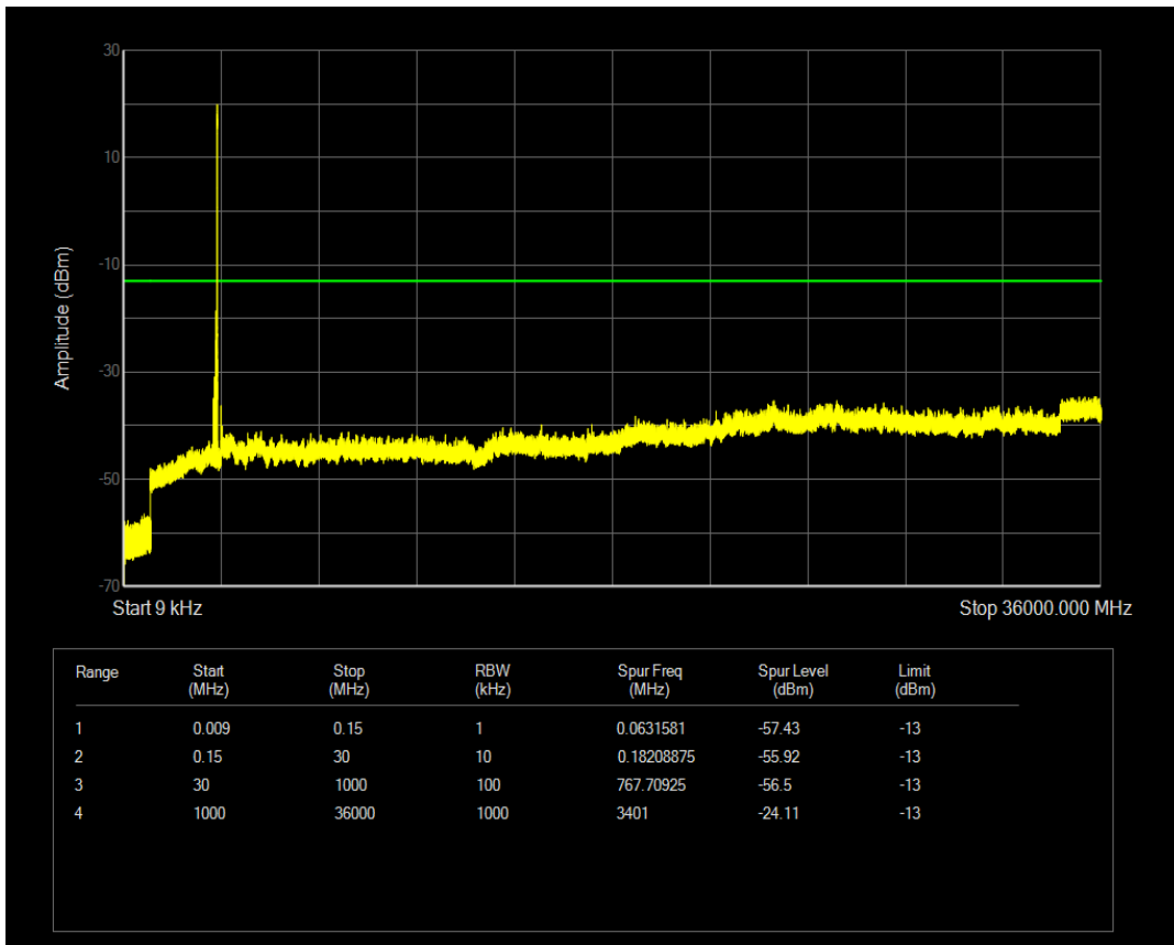
n77(3450-3550) SCS=15kHz DFT_QPSK BW=10MHz Channel=630334 RB=1@0
