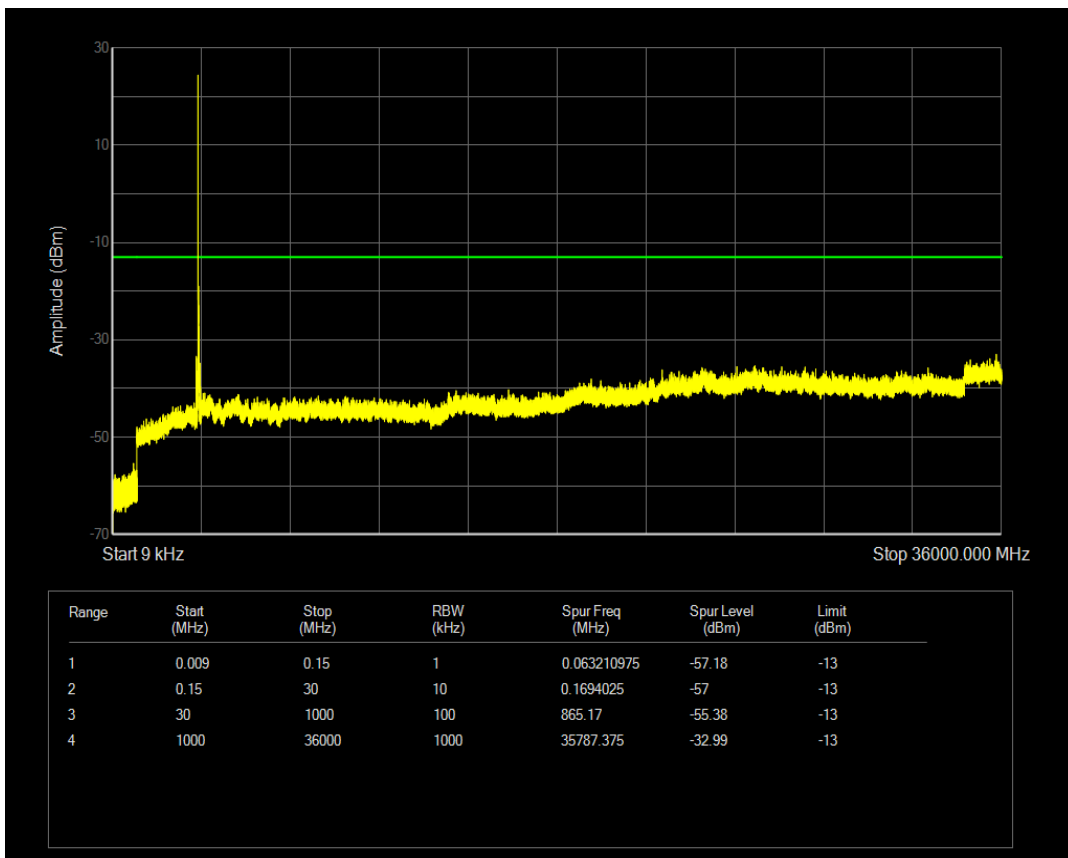
n77(3450-3550) SCS=15kHz DFT_QPSK BW=50MHz Channel=633334 RB=1 @269
