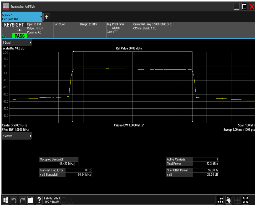
n77(3450-3550) SCS=15kHz CP_QPSK BW=50MHz Channel=633334 RB=270@0
