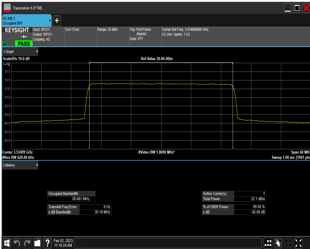
n77(3450-3550) SCS=15kHz CP_QPSK BW=30MHz Channel=635666 RB=160@0
