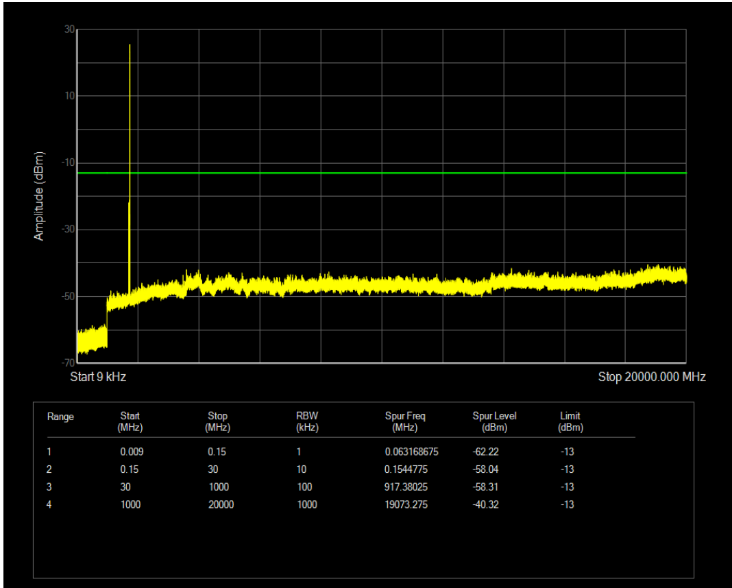
n66 SCS=15kHz DFT_QPSK BW=5MHz Channel=349000 RB=1@0
