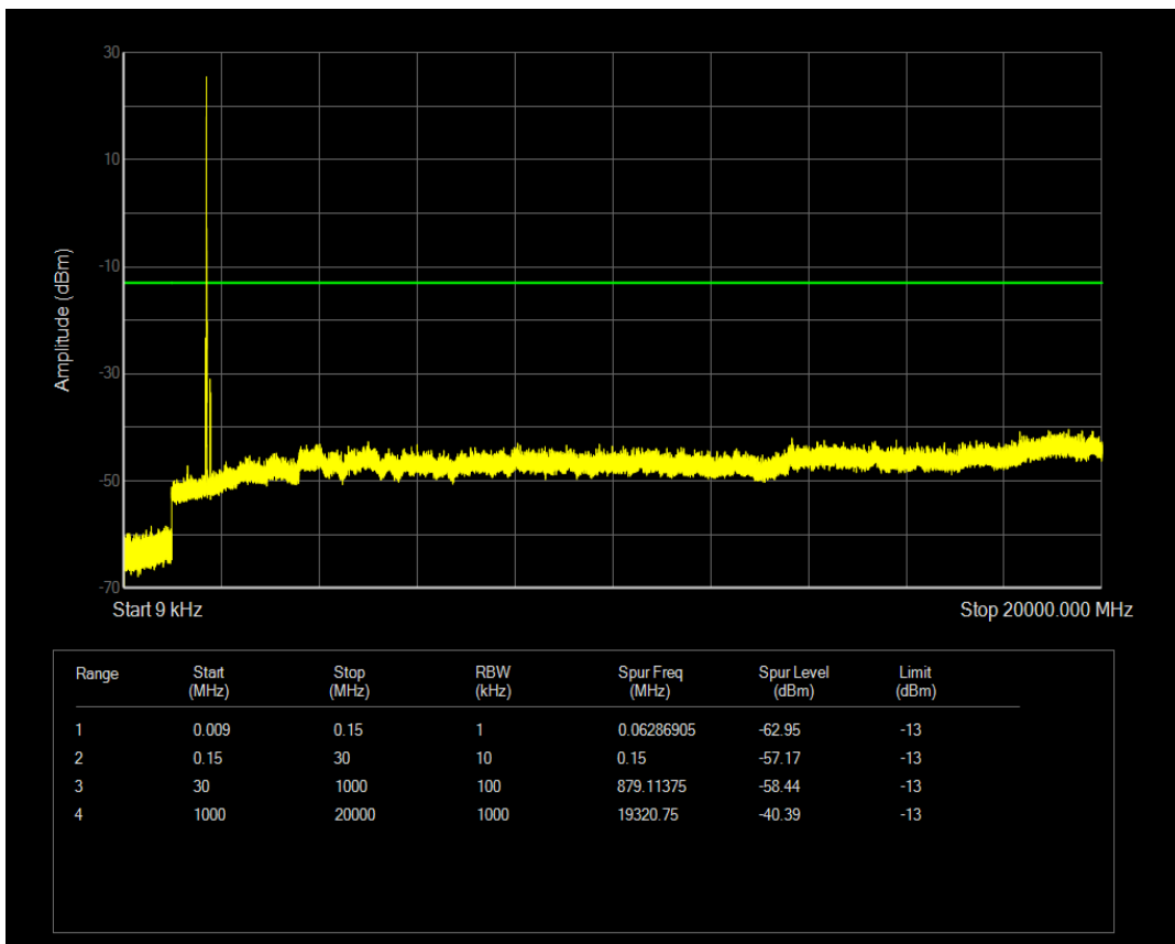
n66 SCS=15kHz DFT_QPSK BW=5MHz Channel=342500 RB=1@24
