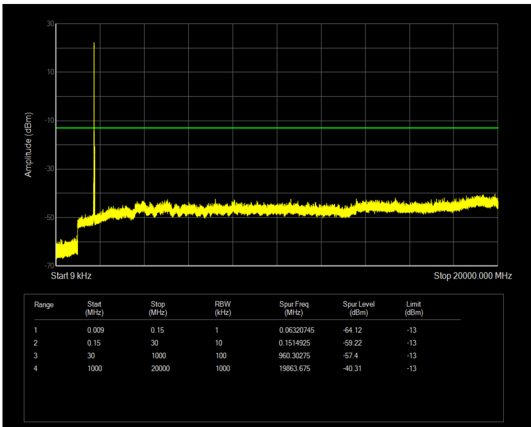
n66 SCS=15kHz DFT_QPSK BW=5MHz Channel=349000 RB=1@24
