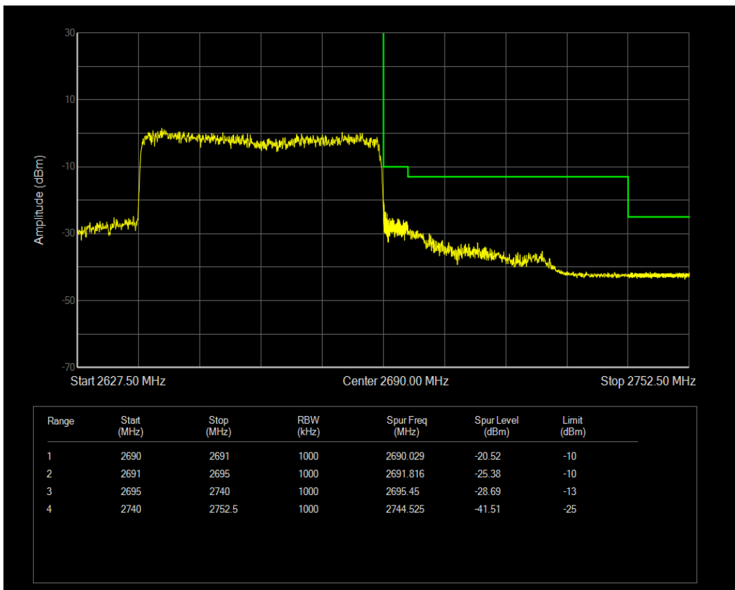
n41 SCS=15kHz DFT_QPSK BW=50MHz Channel=532998 RB=1@269
