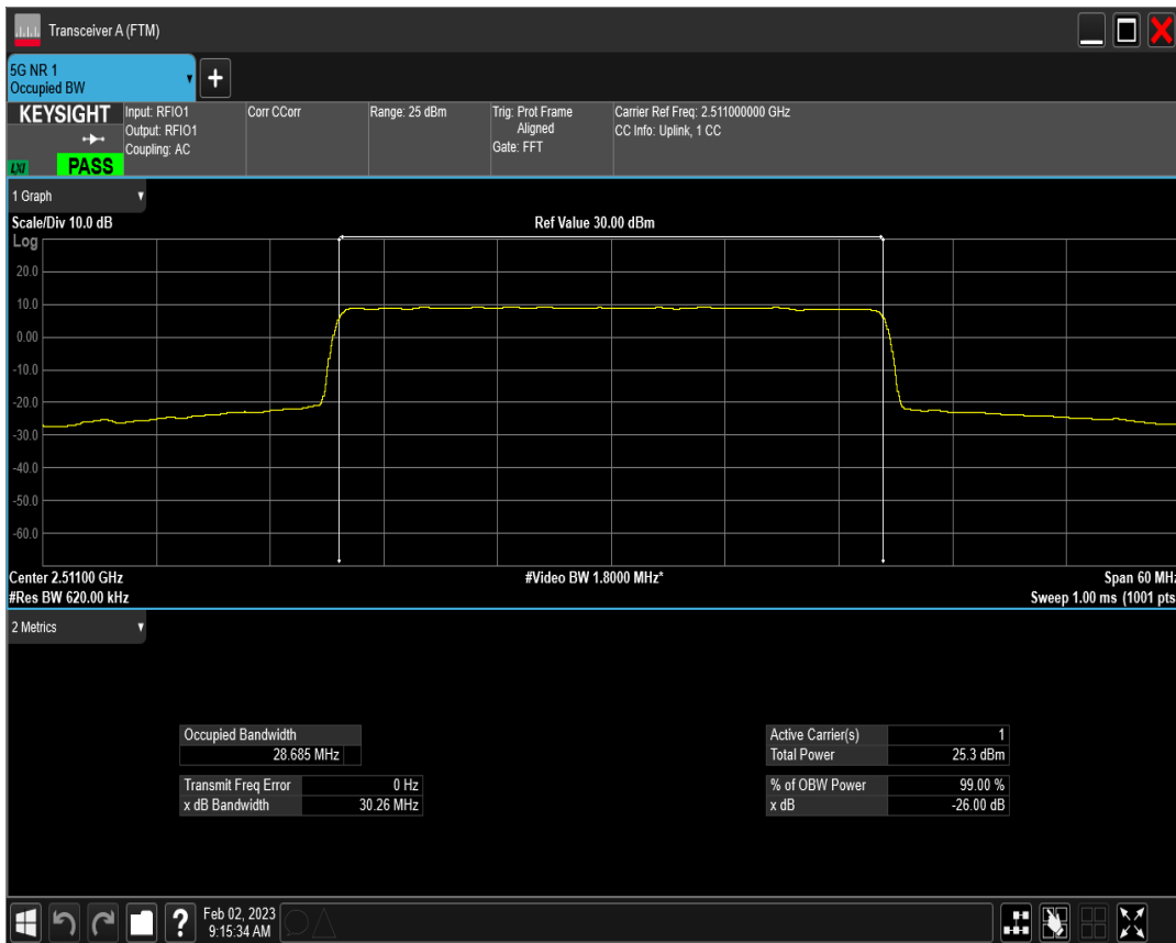
n41 SCS=15kHz DFT_QAM16 BW=30MHz Channel=502200 RB=160@0
