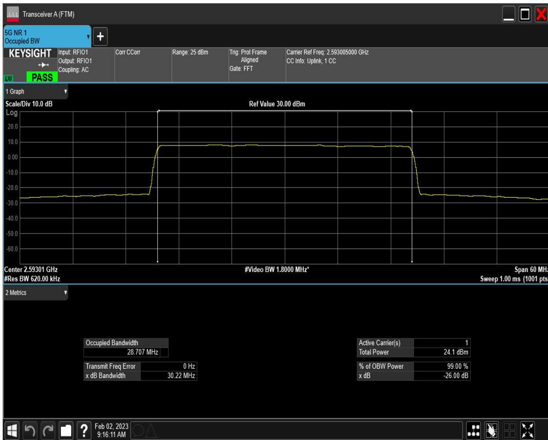
n41 SCS=15kHz DFT_QAM64 BW=30MHz Channel=518601 RB=160@0
