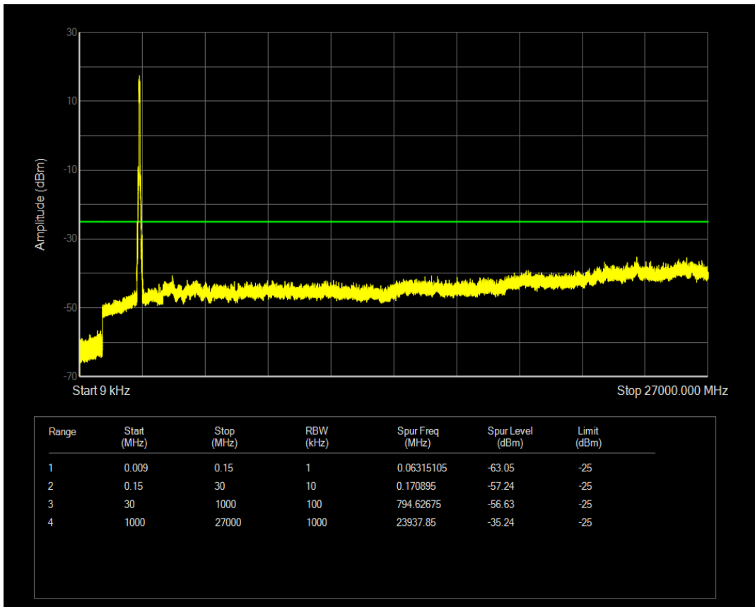
n41 SCS=15kHz DFT_QPSK BW=50MHz Channel=518601 RB=1@269
