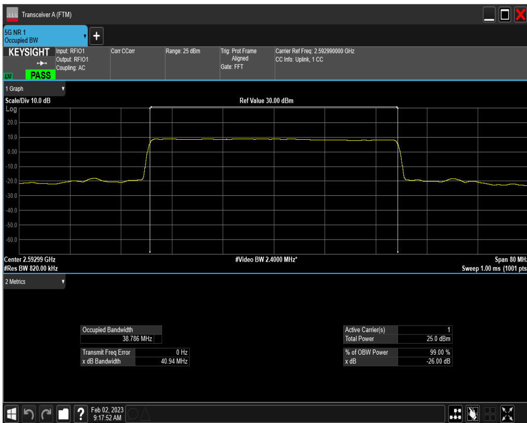
n41 SCS=15kHz DFT_QAM16 BW=40MHz Channel=518598 RB=216@0
