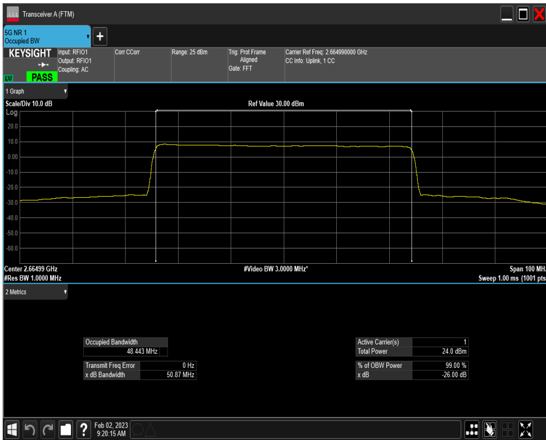
n41 SCS=15kHz DFT_QAM64 BW=50MHz Channel=532998 RB=270@0
