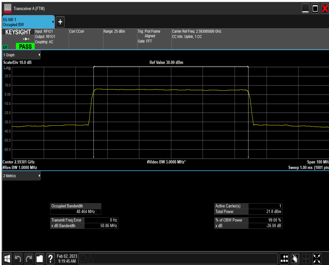
n41 SCS=15kHz CP_QPSK BW=50MHz Channel=518601 RB=270@0
