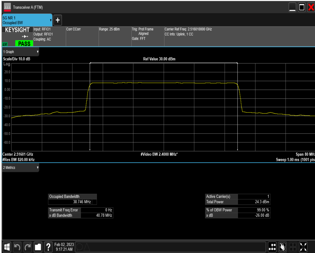
n41 SCS=15kHz DFT_QAM64 BW=40MHz Channel=503202 RB=216@0
