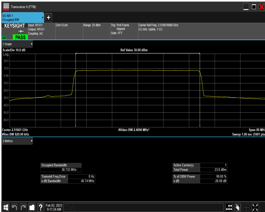
n41 SCS=15kHz DFT_QAM256 BW=40MHz Channel=503202 RB=216@0
