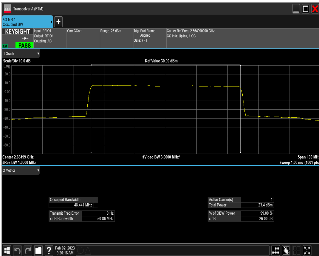
n41 SCS=15kHz DFT_QAM256 BW=50MHz Channel=532998 RB=270@0
