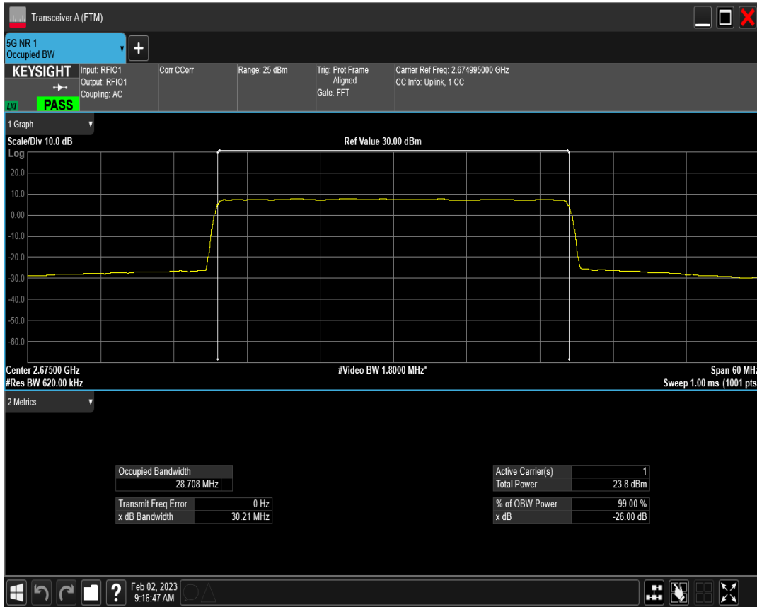
n41 SCS=15kHz DFT_QAM64 BW=30MHz Channel=534999 RB=160@0
