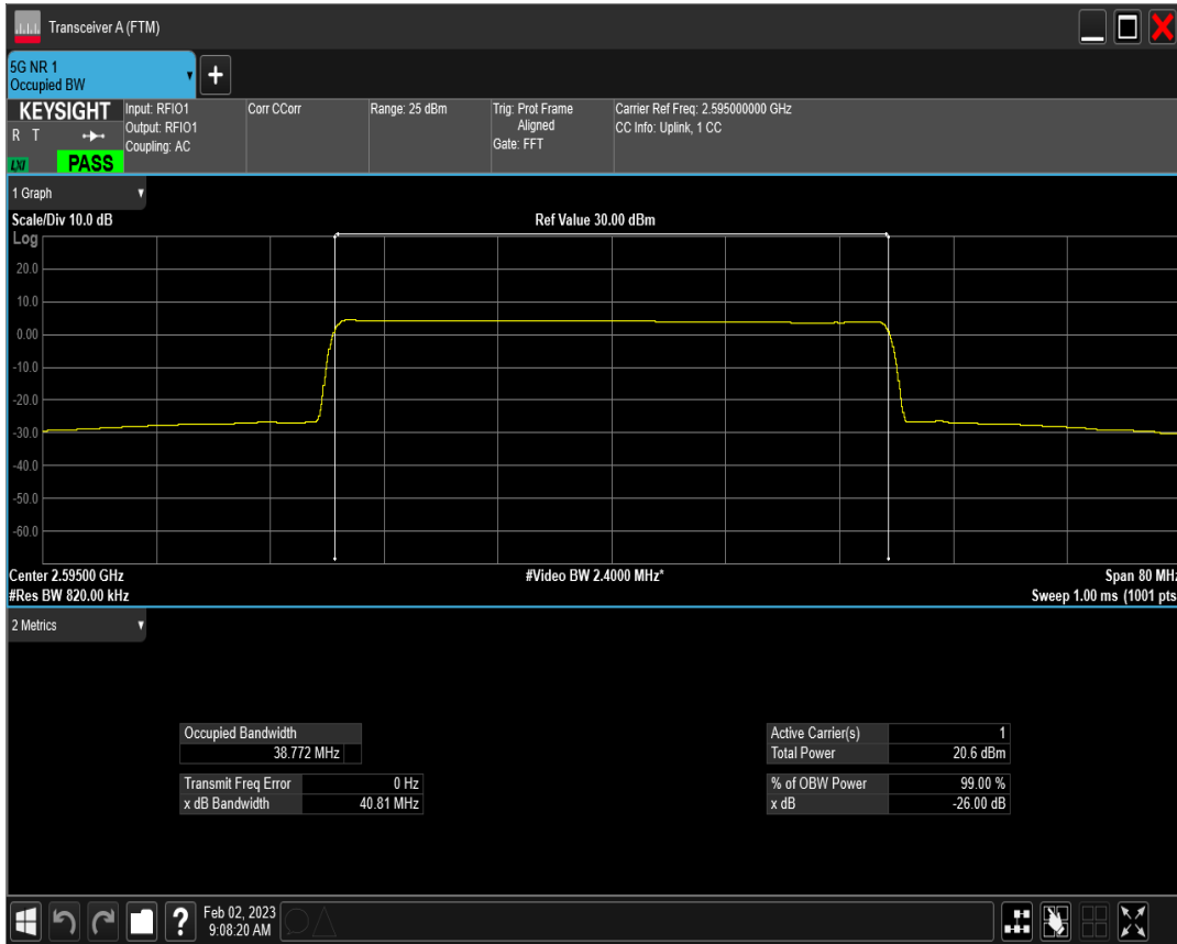
n38 SCS=15kHz DFT_BPSK BW=40MHz Channel=520000 RB=216@0
