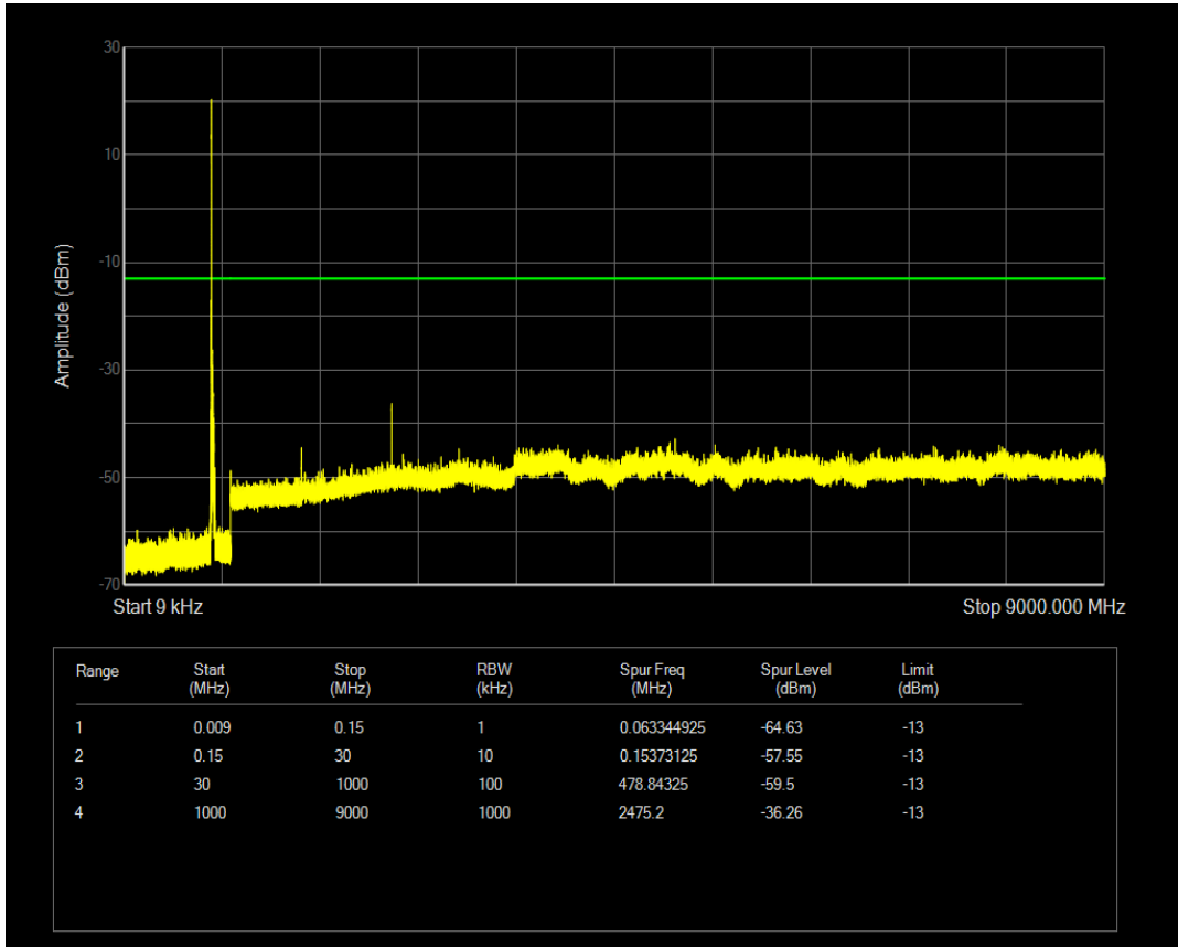
n5 SCS=30kHz DFT_QPSK BW=20MHz Channel=166800 RB=1@50
