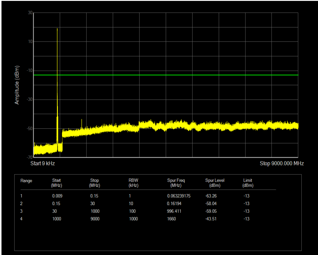
n5 SCS=30kHz DFT_QPSK BW=20MHz Channel=167800 RB=1@50
