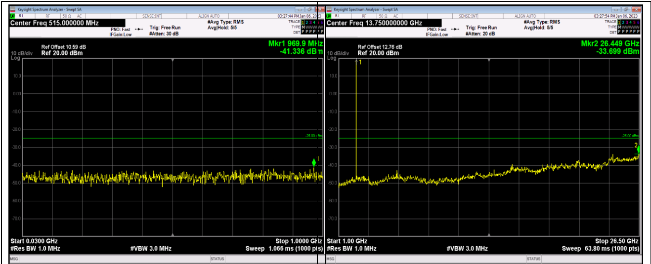
Band7-5MHz-64QAM-21100-1RB#0-Range1:30~1000MHz
