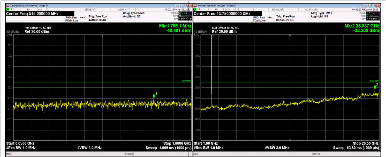
Band7-20MHz-64QAM-21350-1RB#0-Range1:30~1000MHz
