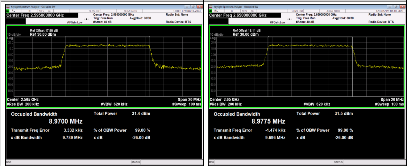
Band41-10MHz-16QAM-40090-50RB#0
