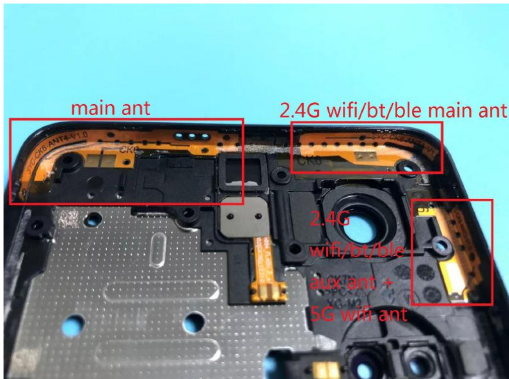
main + 2.4G wifi+bt+ble+5G wifi Antenna
