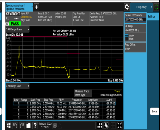
Band7-20MHz-QPSK-21350-100RB#0
