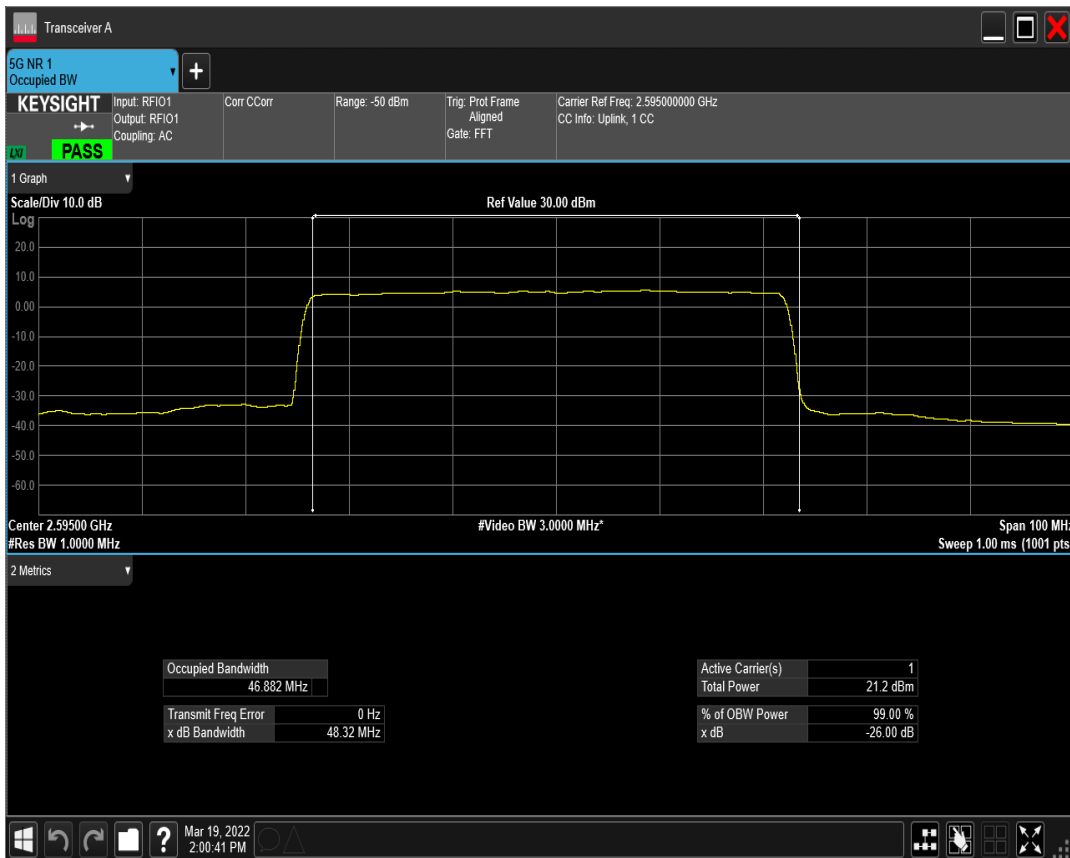
n41(2535-2655) SCS=30kHz CP_QPSK BW=50MHz Channel=519000 RB=133@0
