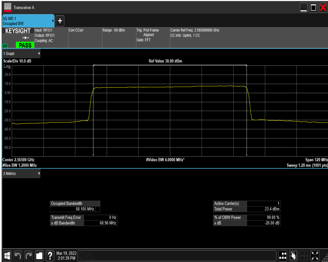
n41(2535-2655) SCS=30kHz DFT_QAM256 BW=60MHz Channel=513000 RB=162@0
