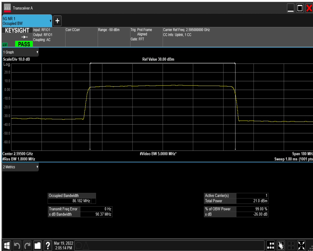
n41(2535-2655) SCS=30kHz CP_QPSK BW=90MHz Channel=519000 RB=245@0
