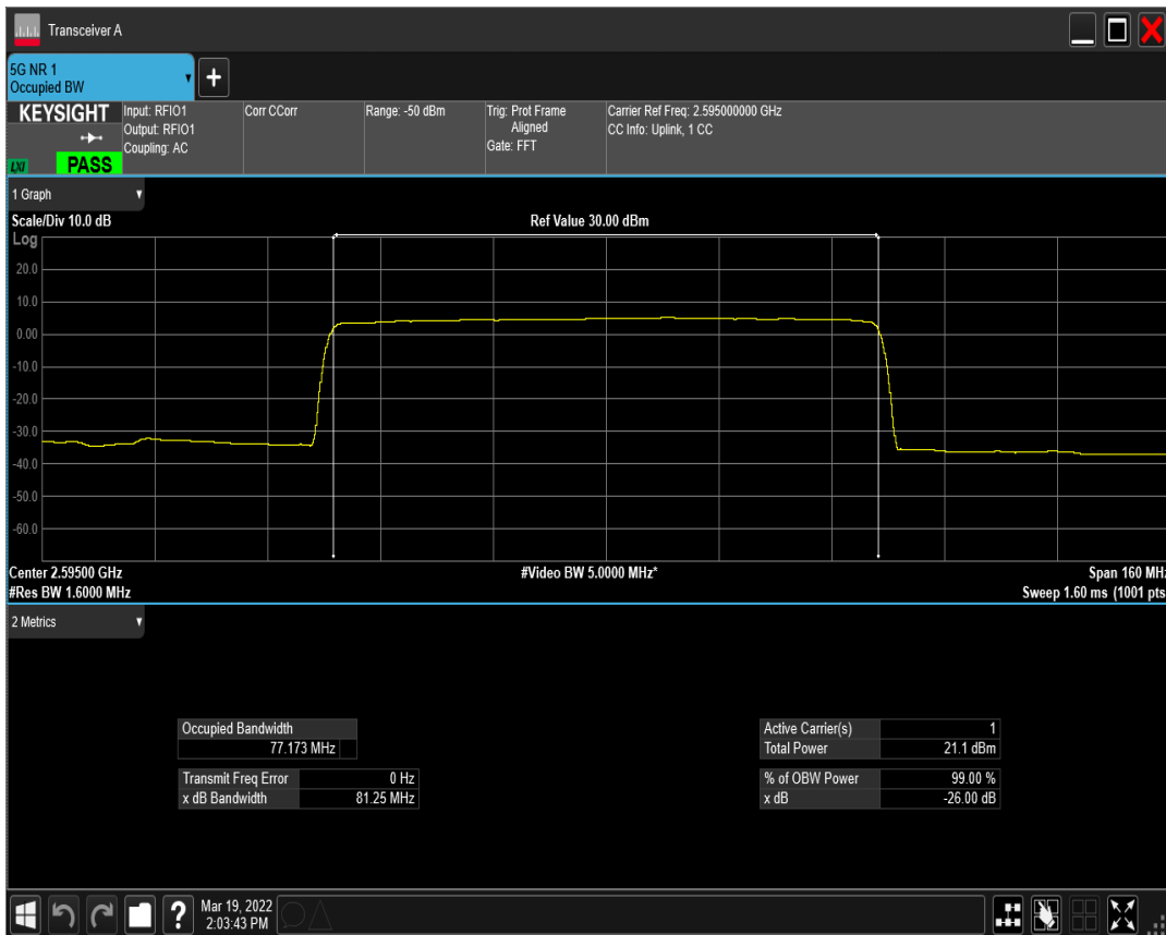
n41(2535-2655) SCS=30kHz CP_QPSK BW=80MHz Channel=519000 RB=217@0
