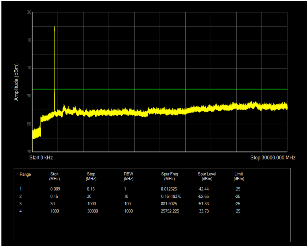
n41(2535-2655) SCS=30kHz DFT_QPSK BW=10MHz Channel=529998 RB=1 @0
