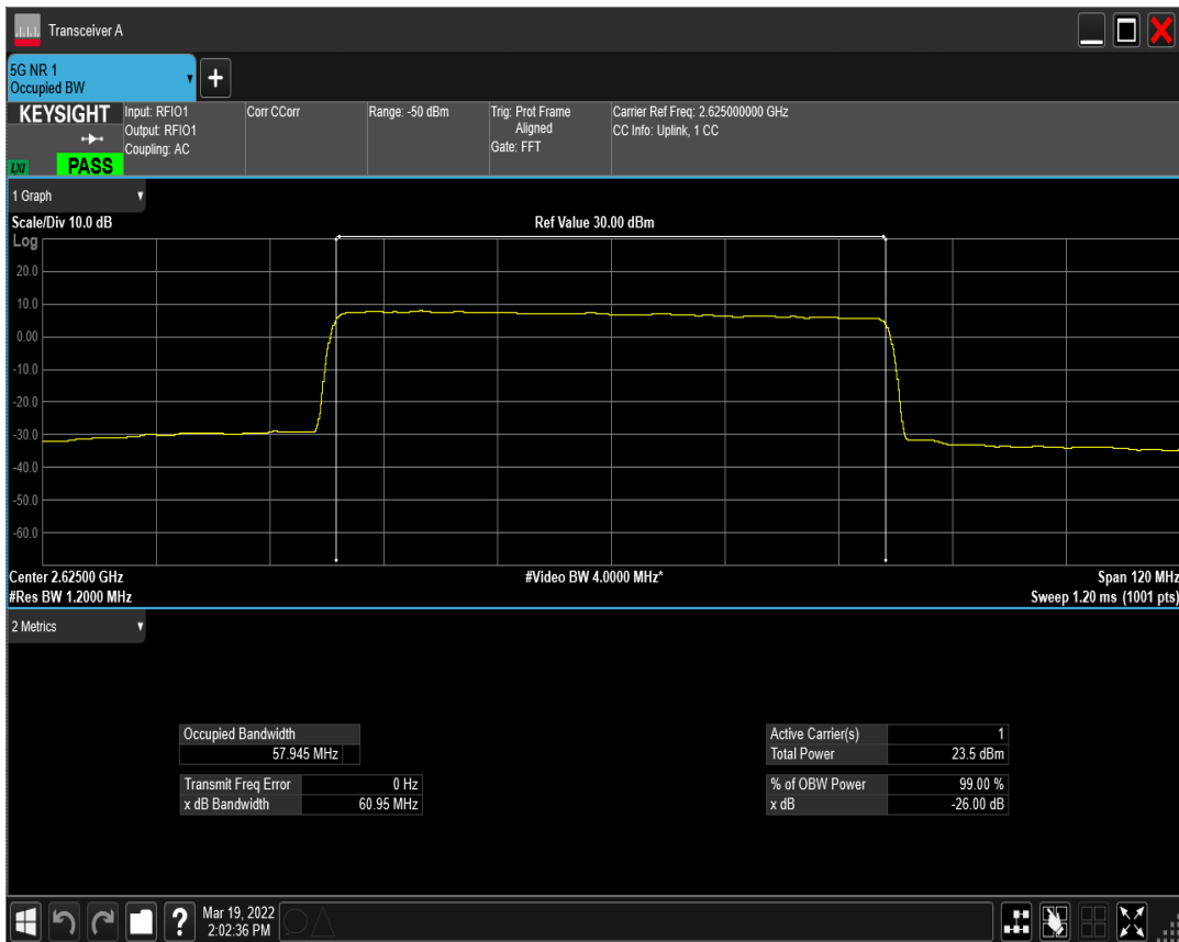
n41(2535-2655) SCS=30kHz DFT_QAM64 BW=60MHz Channel=525000 RB=162@0
