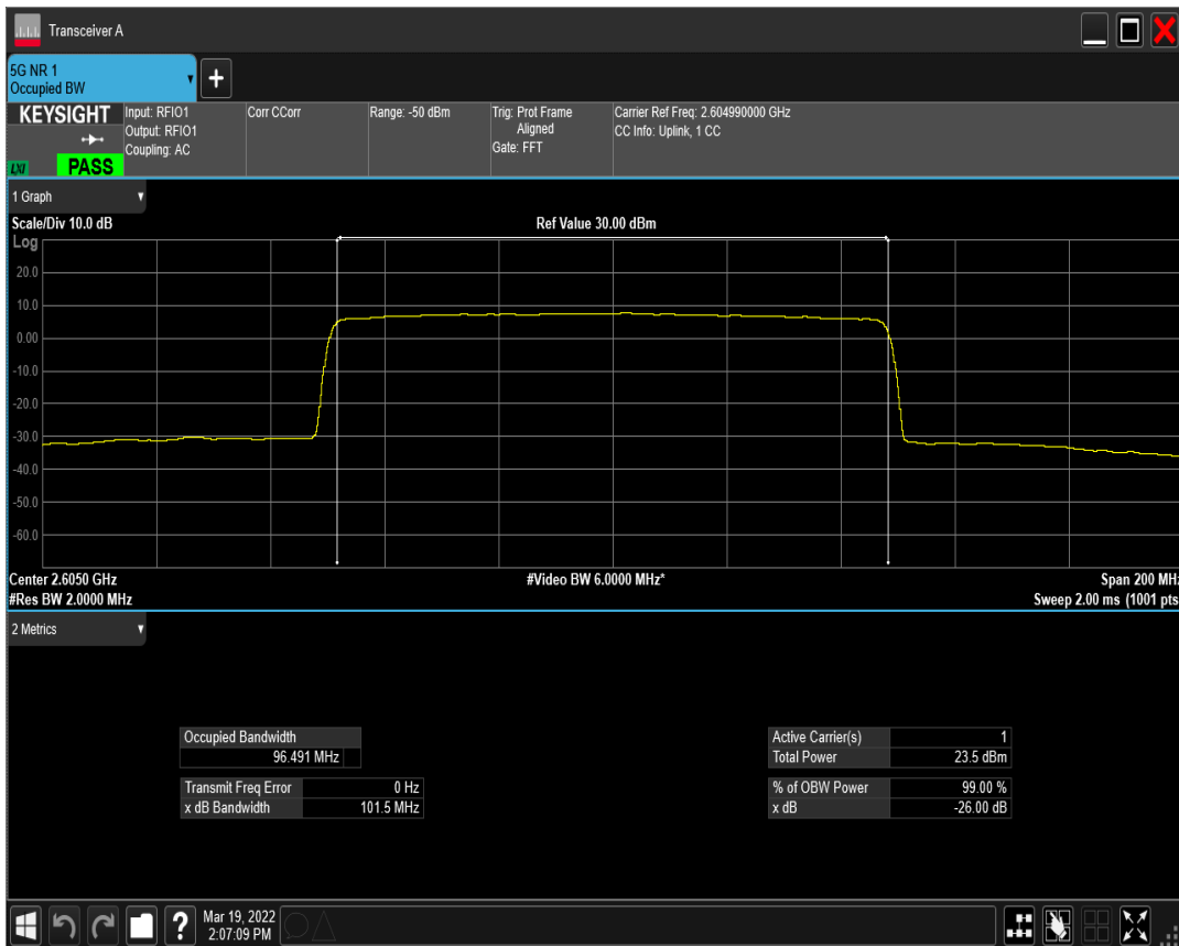
n41(2535-2655) SCS=30kHz DFT_QAM64 BW=100MHz Channel=520998 RB=270@0
