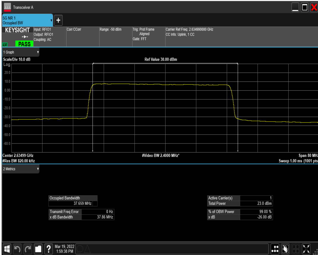
n41(2535-2655) SCS=30kHz DFT_QAM256 BW=40MHz Channel=526998 RB=100@0
