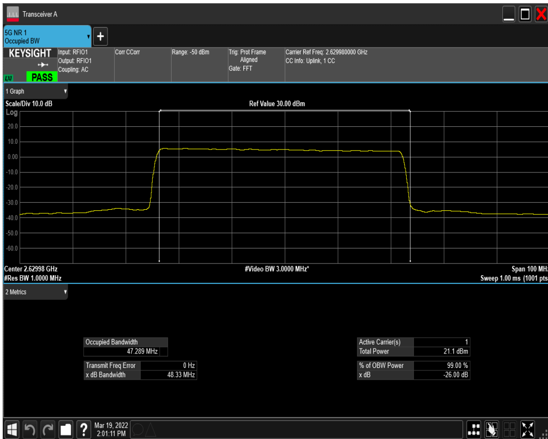
n41(2535-2655) SCS=30kHz CP_QPSK BW=50MHz Channel=525996 RB=133@0
