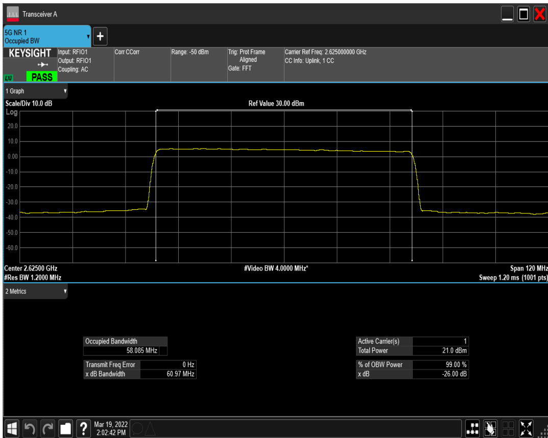
n41(2535-2655) SCS=30kHz CP_QPSK BW=60MHz Channel=525000 RB=162@0
