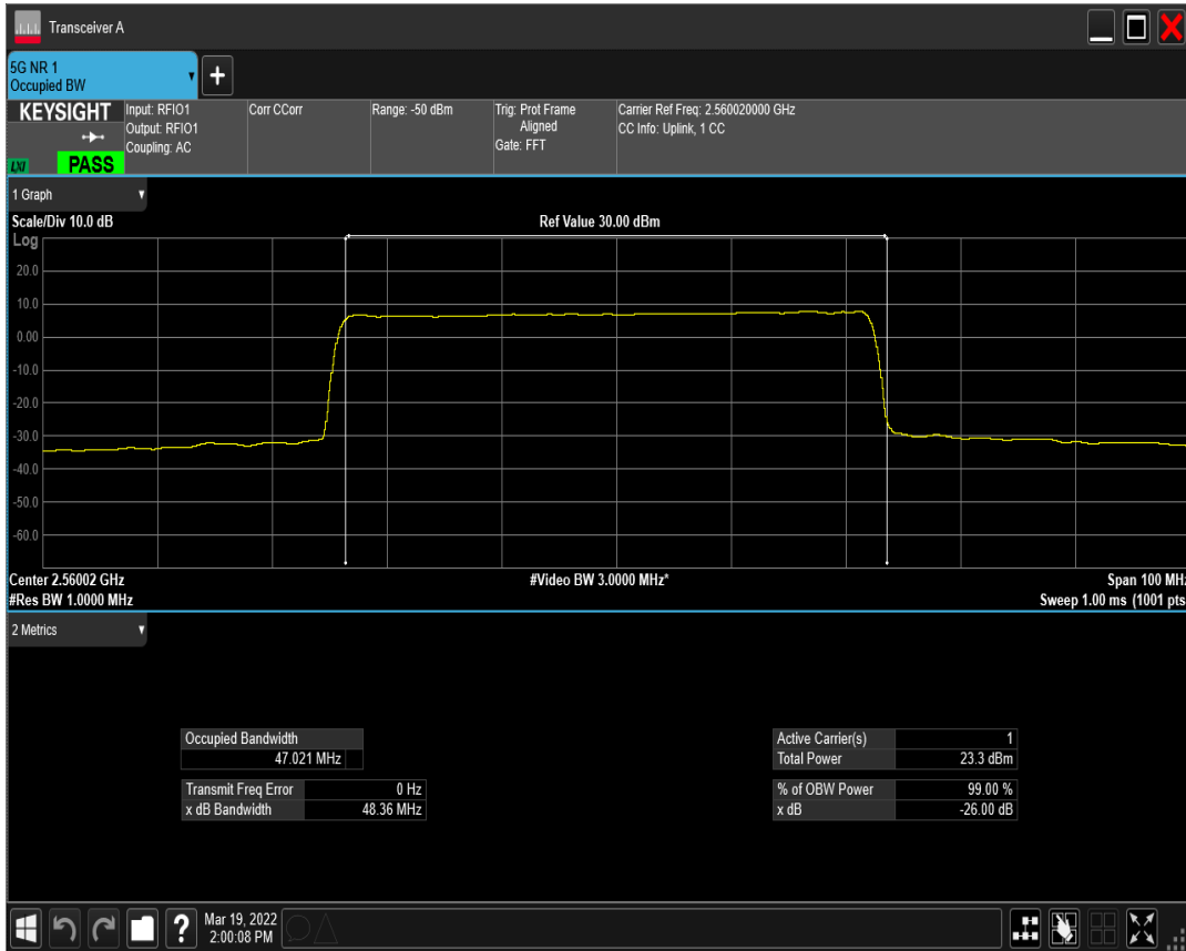
n41(2535-2655) SCS=30kHz DFT_QAM256 BW=50MHz Channel=512004 RB=128@0
