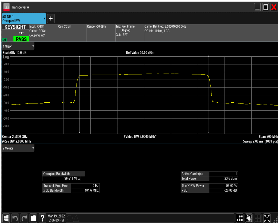
n41(2535-2655) SCS=30kHz DFT_QAM64 BW=100MHz Channel=517002 RB=270@0
