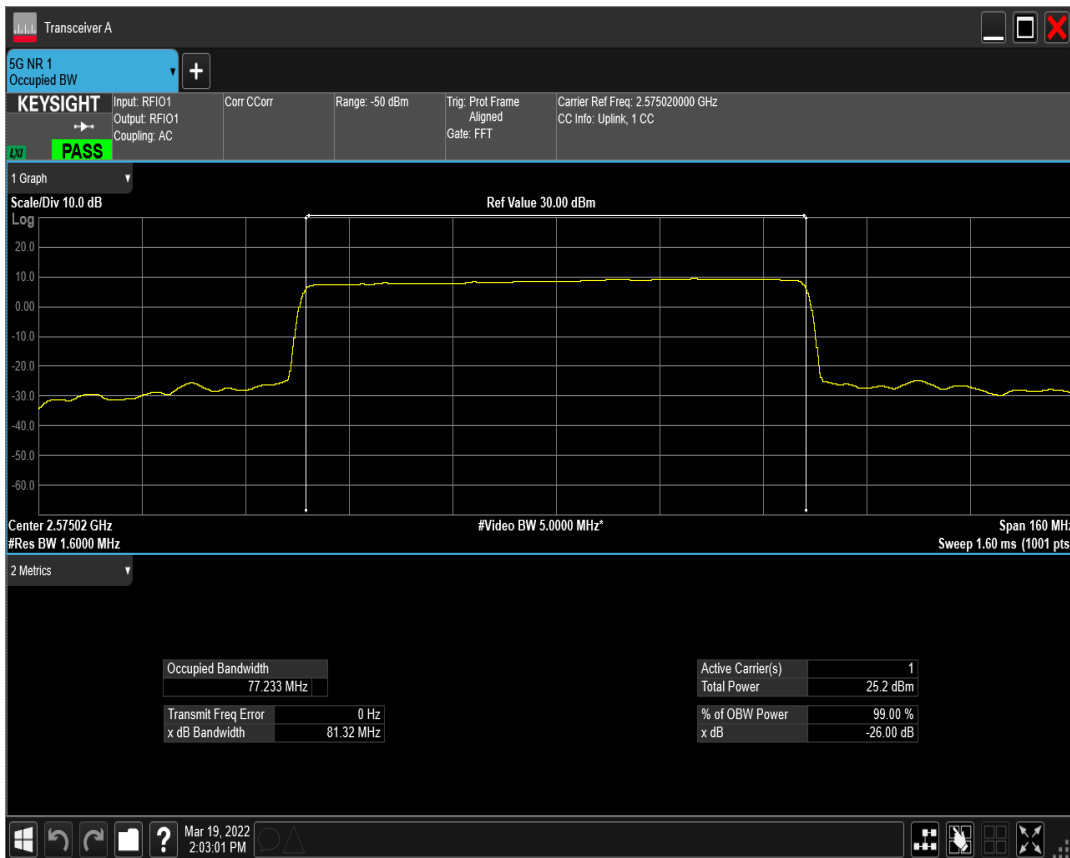
n41(2535-2655) SCS=30kHz DFT_QPSK BW=80MHz Channel=515004 RB=216@0
