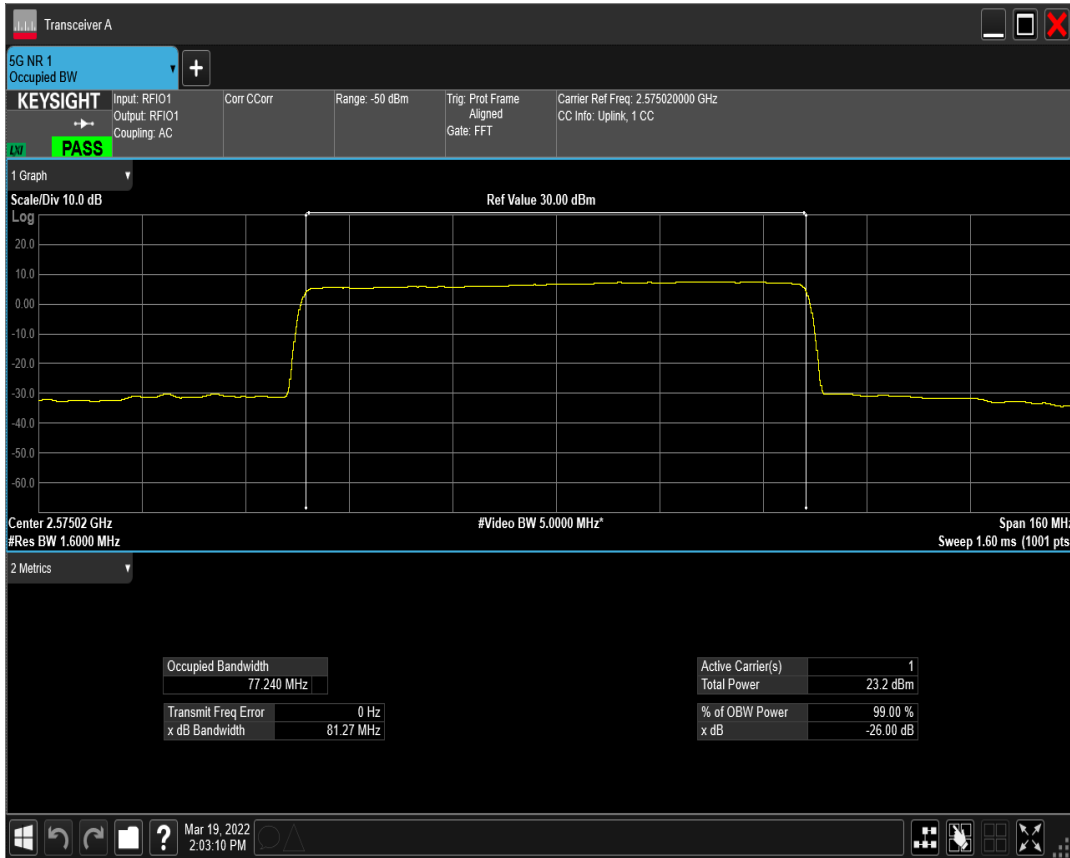
n41(2535-2655) SCS=30kHz DFT_QAM256 BW=80MHz Channel=515004 RB=216@0
