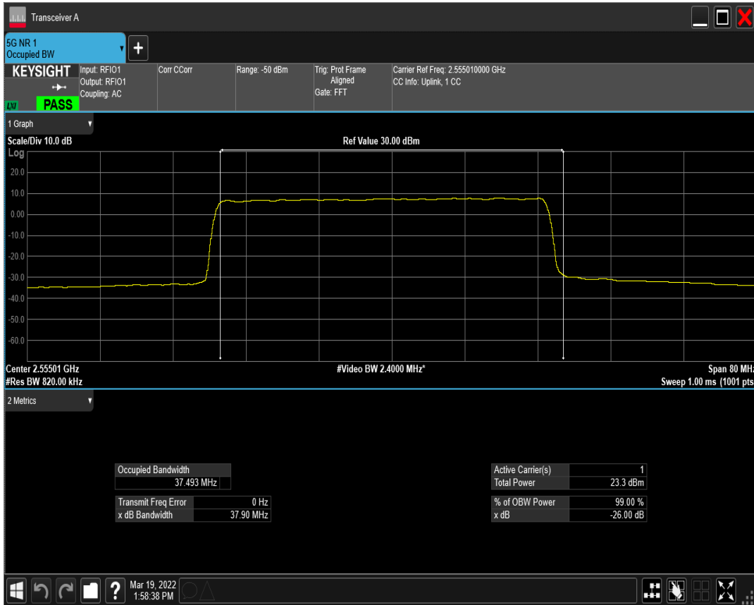
n41(2535-2655) SCS=30kHz DFT_QAM256 BW=40MHz Channel=511002 RB=100@0
