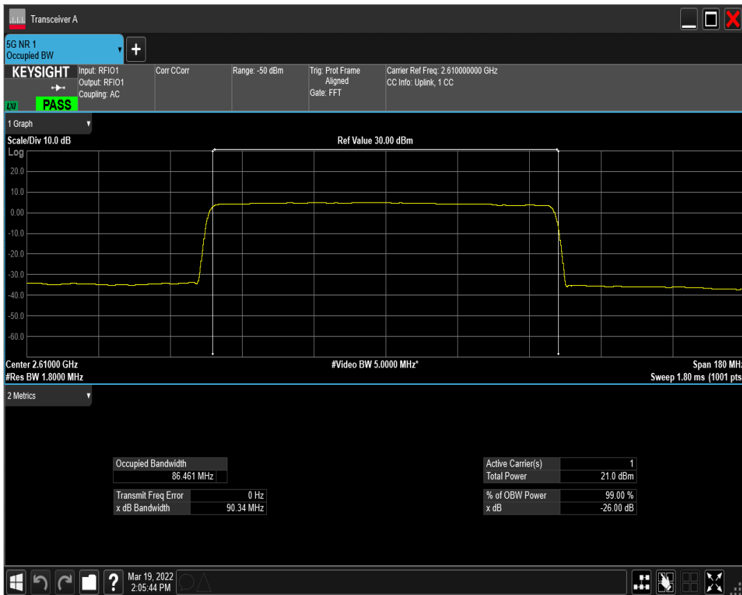
n41(2535-2655) SCS=30kHz CP_QPSK BW=90MHz Channel=522000 RB=245@0
