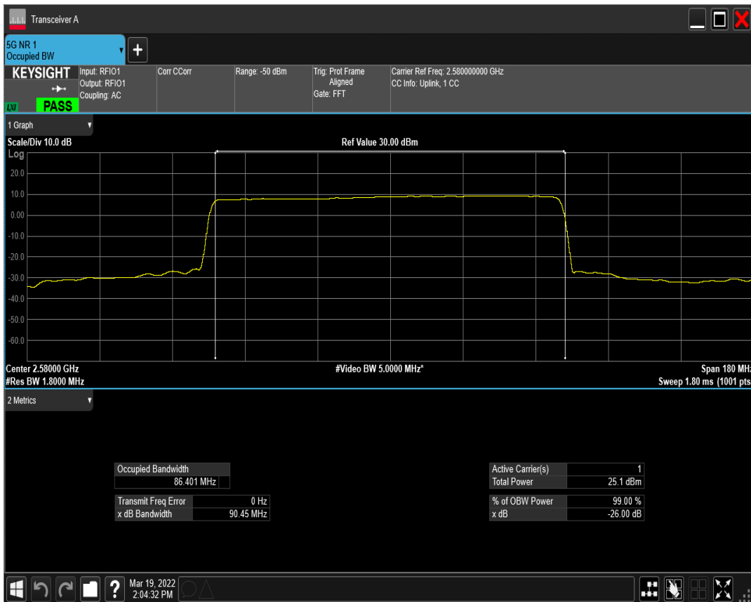
n41(2535-2655) SCS=30kHz DFT_QPSK BW=90MHz Channel=516000 RB=240@0
