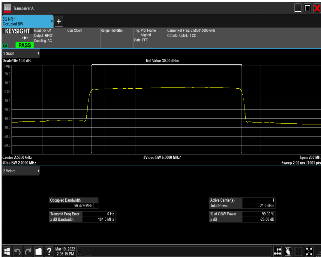
n41(2535-2655) SCS=30kHz CP_QPSK BW=100MHz Channel=517002 RB=273@0
