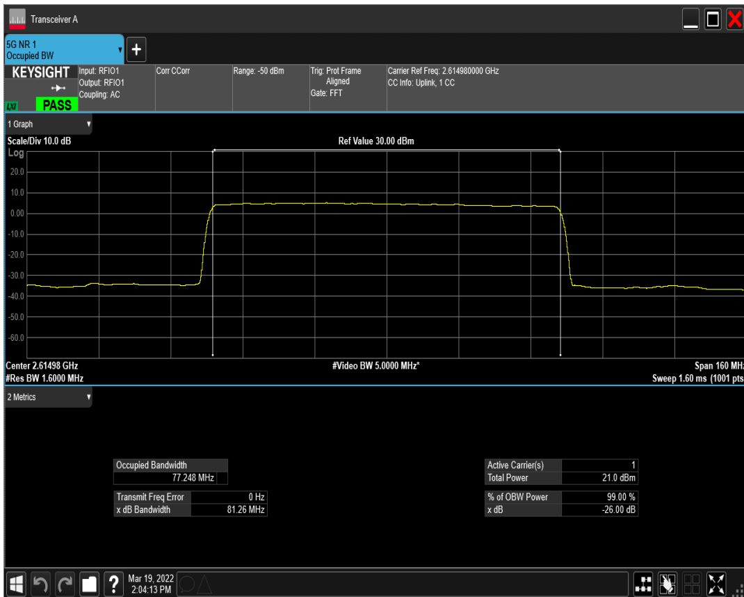
n41(2535-2655) SCS=30kHz CP_QPSK BW=80MHz Channel=522996 RB=217@0
