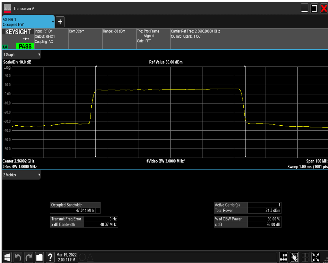
n41(2535-2655) SCS=30kHz CP_QPSK BW=50MHz Channel=512004 RB=133@0
