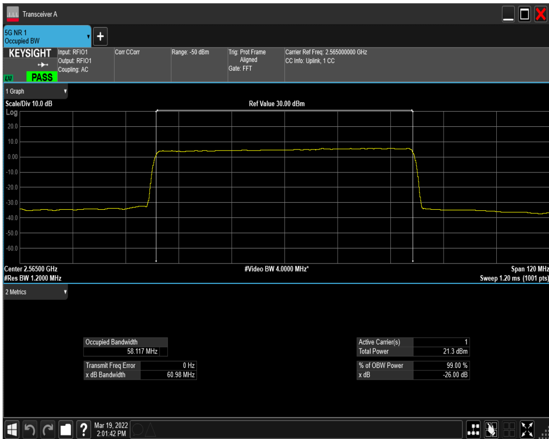
n41(2535-2655) SCS=30kHz CP_QPSK BW=60MHz Channel=513000 RB=162@0
