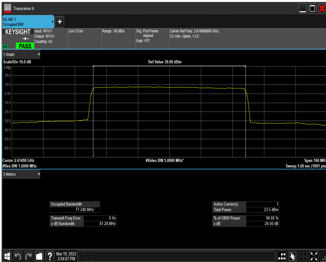
n41(2535-2655) SCS=30kHz DFT_QAM64 BW=80MHz Channel=522996 RB=216@0
