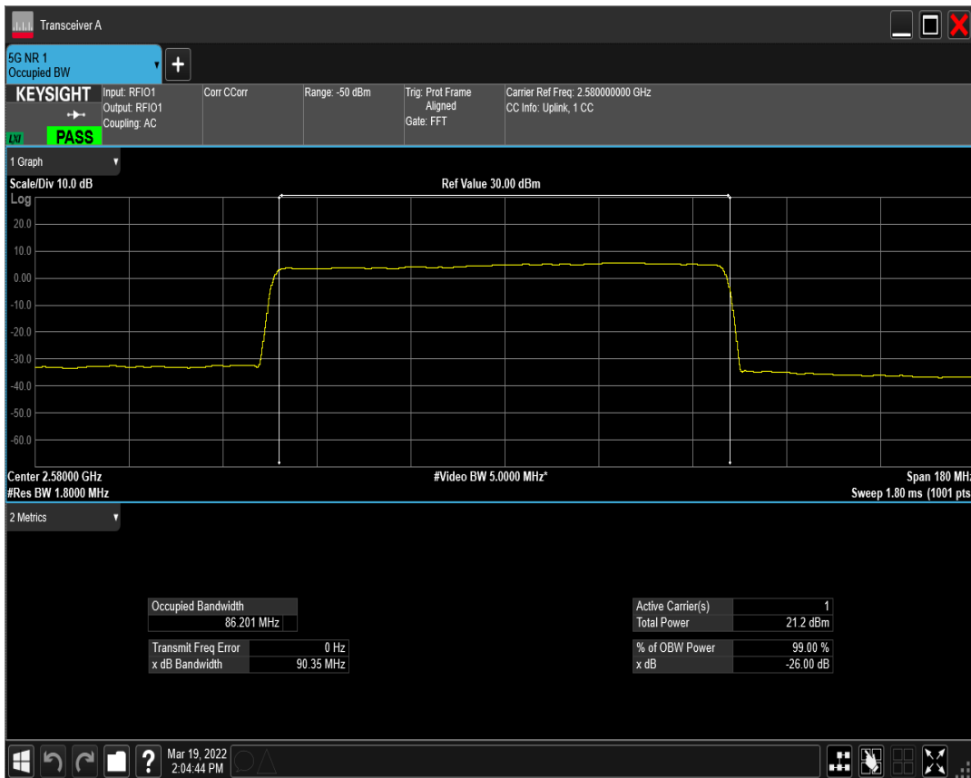
n41(2535-2655) SCS=30kHz CP_QPSK BW=90MHz Channel=516000 RB=245@0
