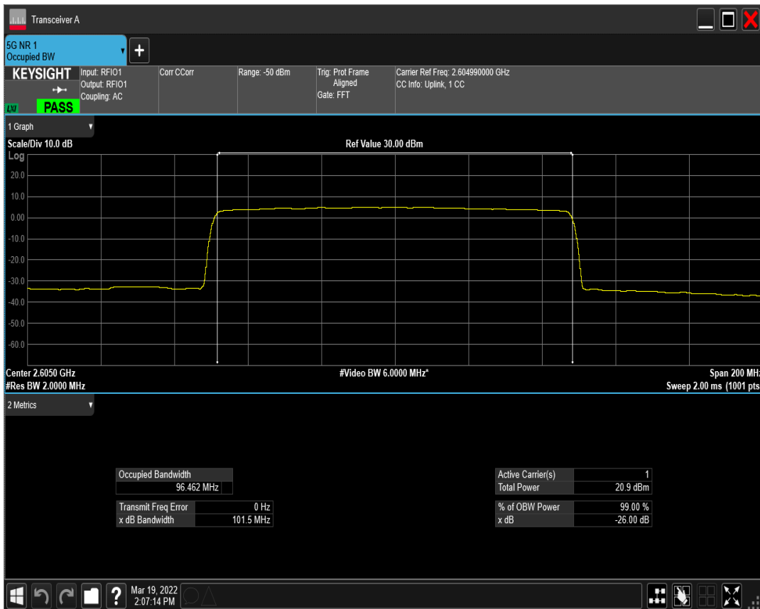
n41(2535-2655) SCS=30kHz CP_QPSK BW=100MHz Channel=520998 RB=273 @0
