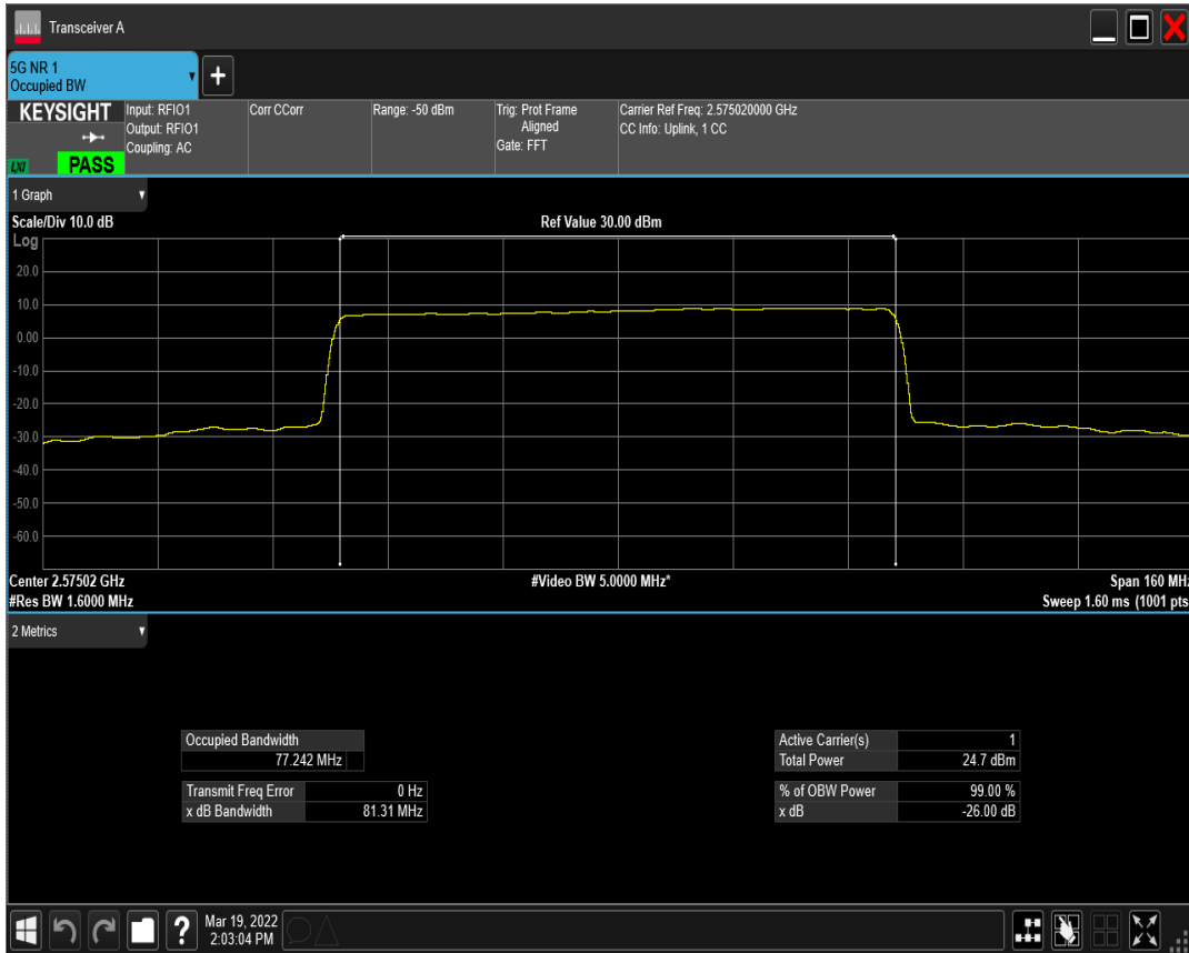
n41(2535-2655) SCS=30kHz DFT_QAM16 BW=80MHz Channel=515004 RB=216@0
