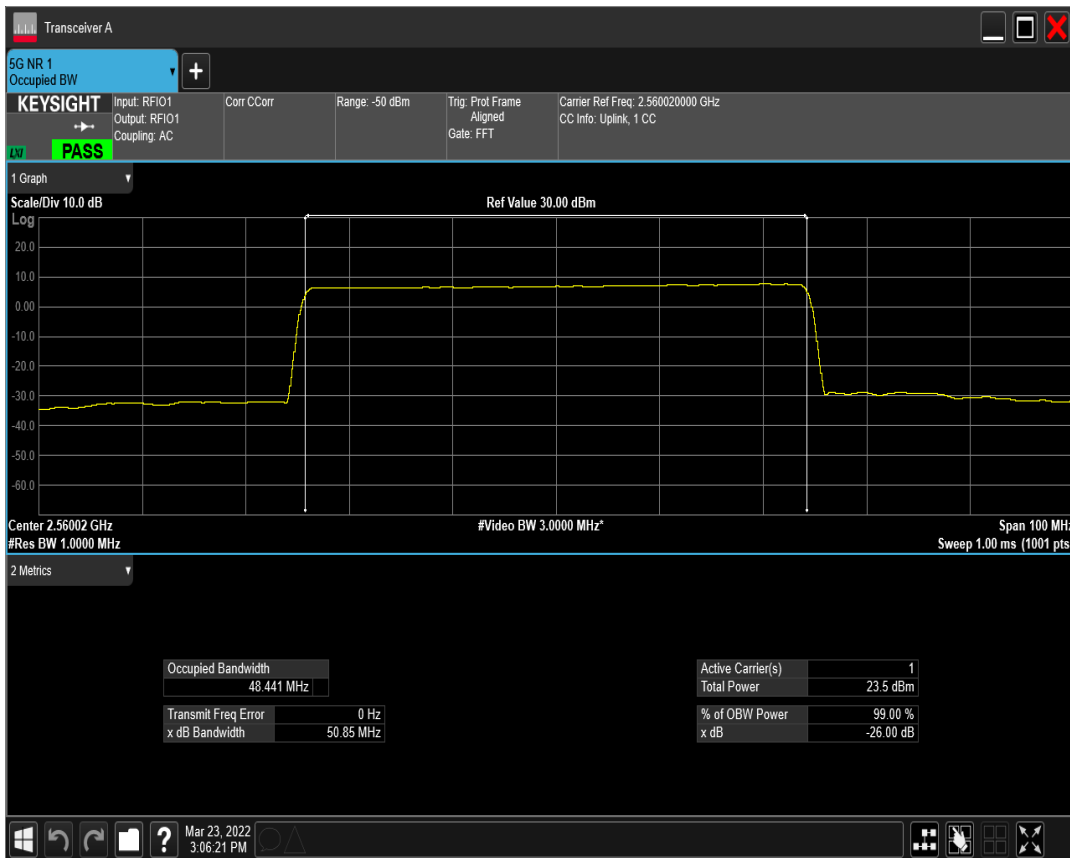
n41(2535-2655) SCS=15kHz DFT_QAM256 BW=50MHz Channel=512004 RB=270@0
