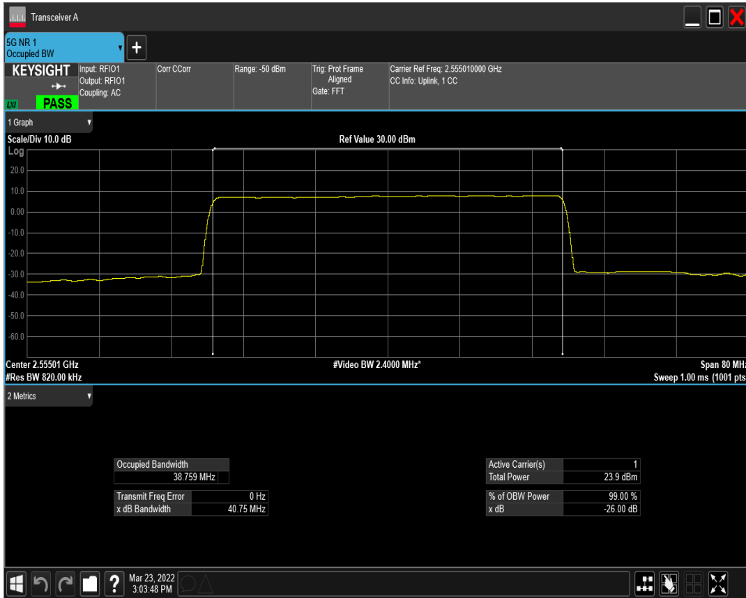
n41(2535-2655) SCS=15kHz DFT_QAM64 BW=40MHz Channel=511002 RB=216@0
