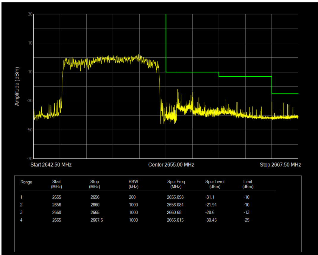
n41(2535-2655) SCS=15kHz DFT_QPSK BW=10MHz Channel=529998 RB=1@51
