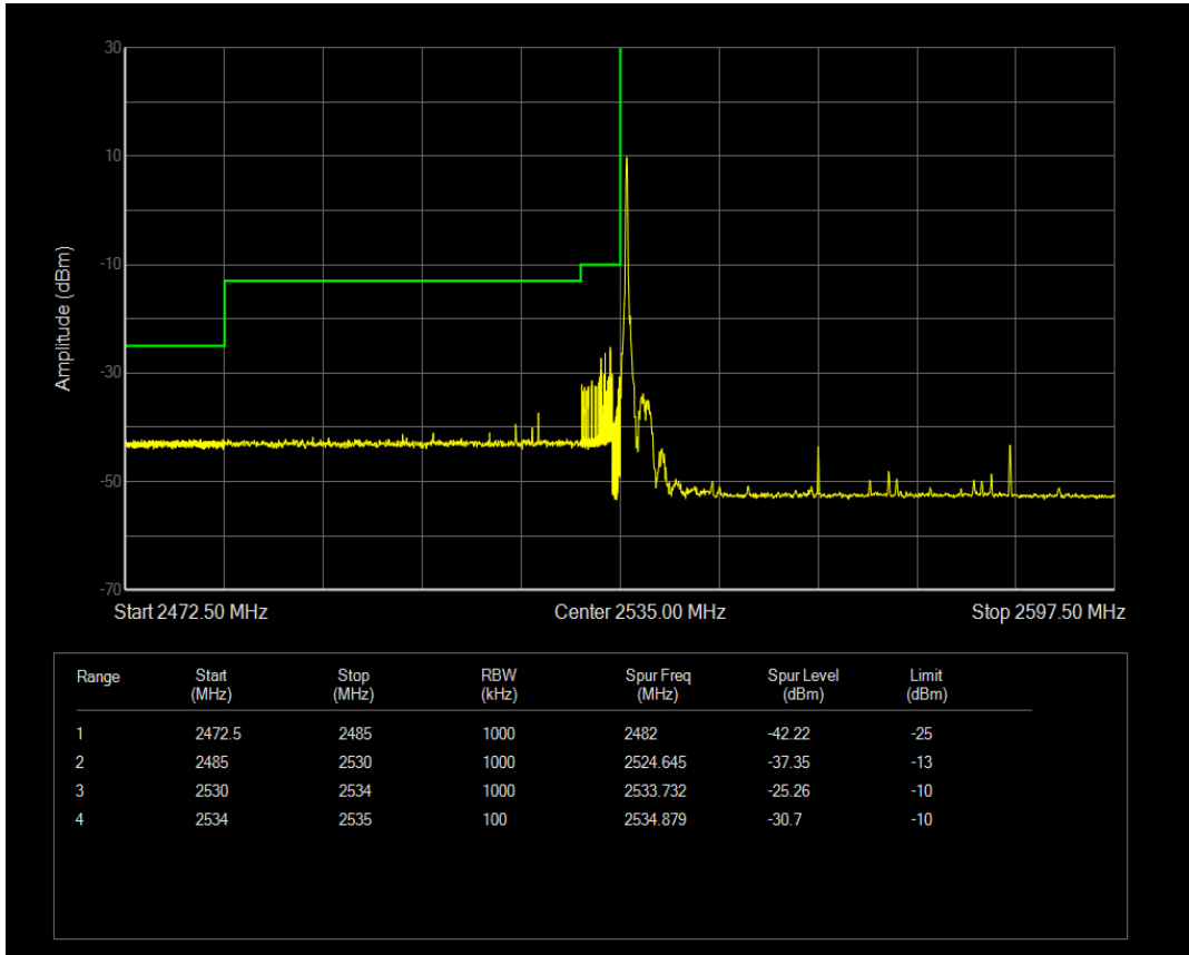
n41(2535-2655) SCS=15kHz DFT_QPSK BW=50MHz Channel=525996 RB=270@0
