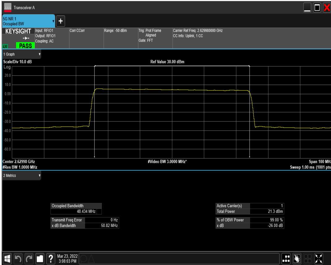
n41(2535-2655) SCS=15kHz CP_QPSK BW=50MHz Channel=525996 RB=270@0
