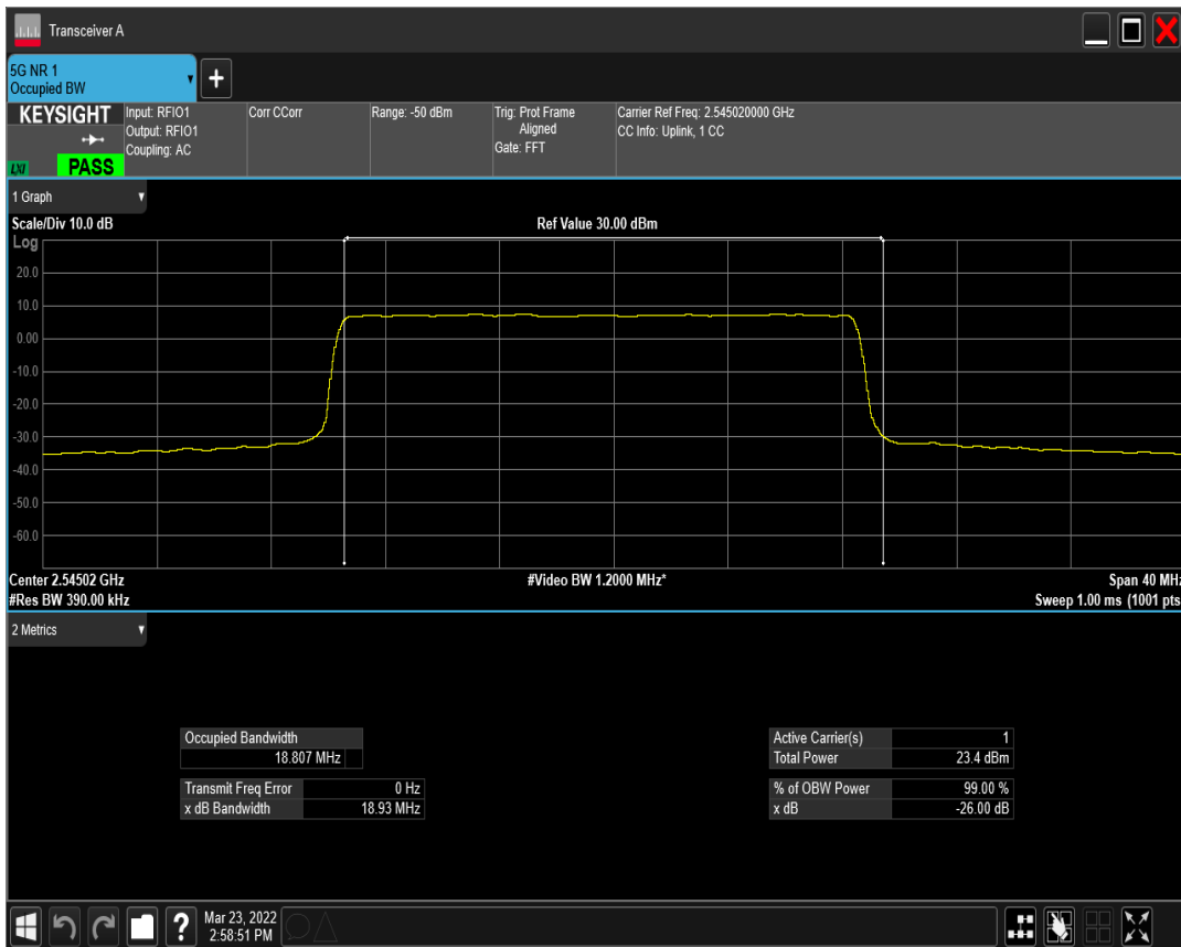
n41(2535-2655) SCS=15kHz DFT_QAM256 BW=20MHz Channel=509004 RB=100@0
