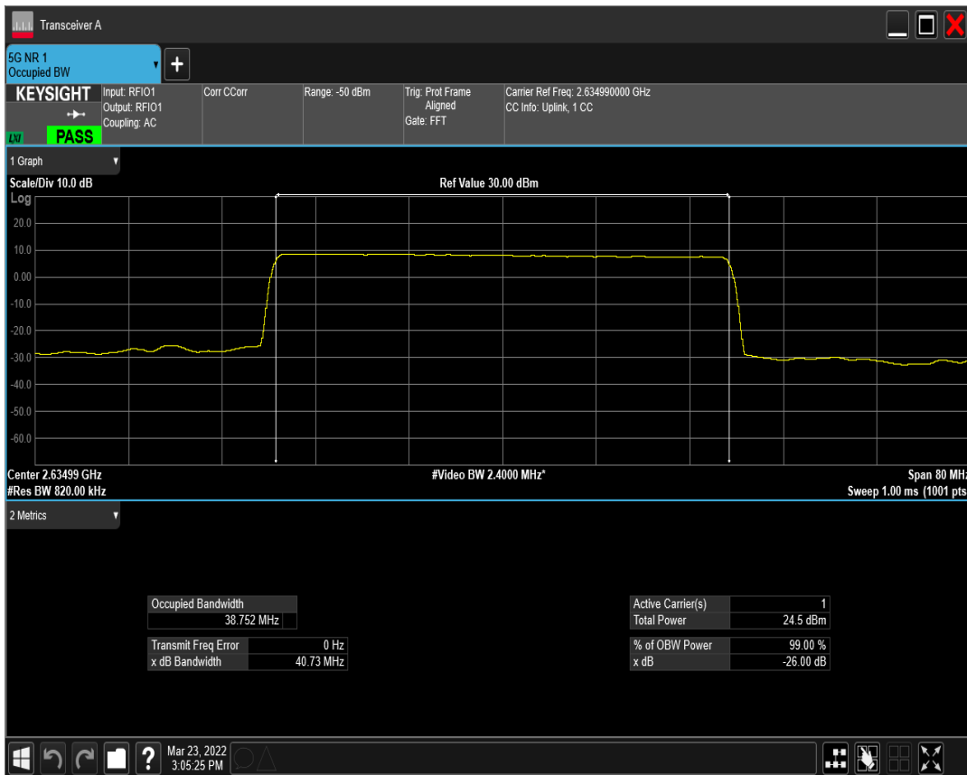
n41(2535-2655) SCS=15kHz DFT_QAM16 BW=40MHz Channel=526998 RB=216@0
