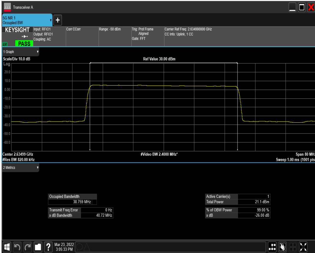
n41(2535-2655) SCS=15kHz CP_QPSK BW=40MHz Channel=526998 RB=216@0
