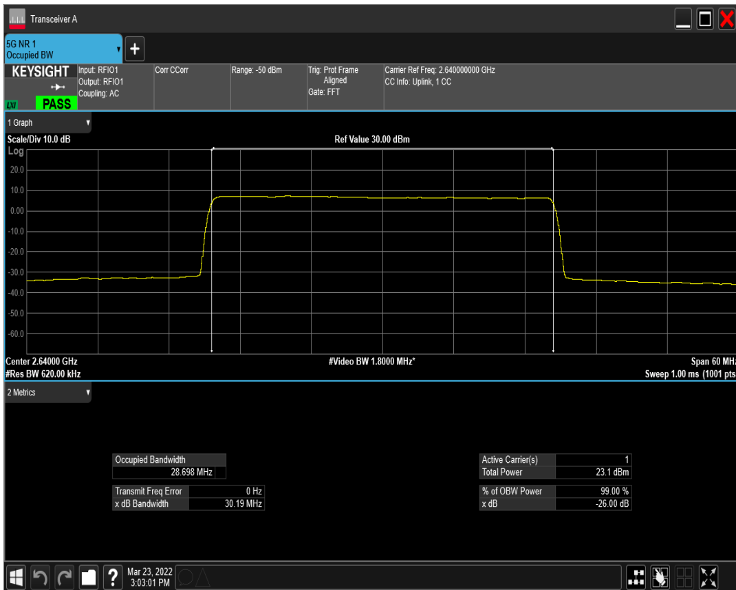
n41(2535-2655) SCS=15kHz DFT_QAM256 BW=30MHz Channel=528000 RB=160@0
