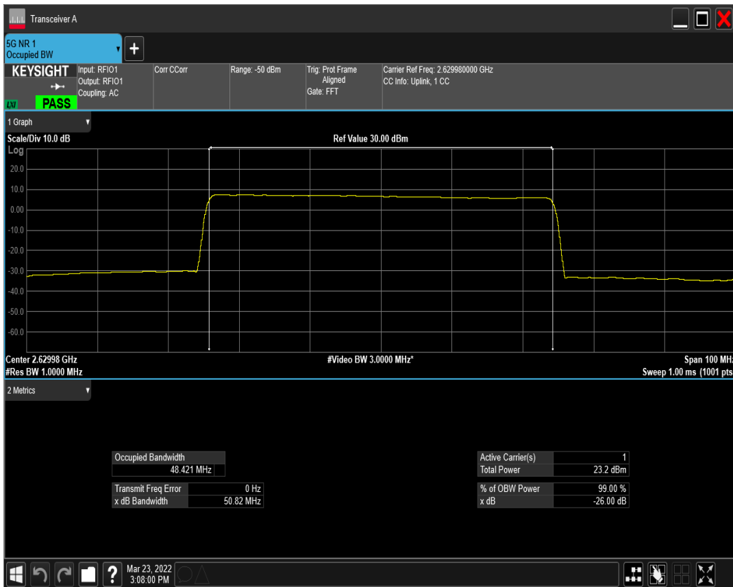
n41(2535-2655) SCS=15kHz DFT_QAM256 BW=50MHz Channel=525996 RB=270@0
