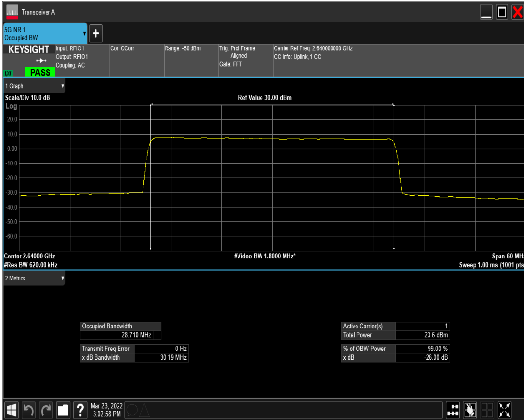
n41(2535-2655) SCS=15kHz DFT_QAM64 BW=30MHz Channel=528000 RB=160@0
