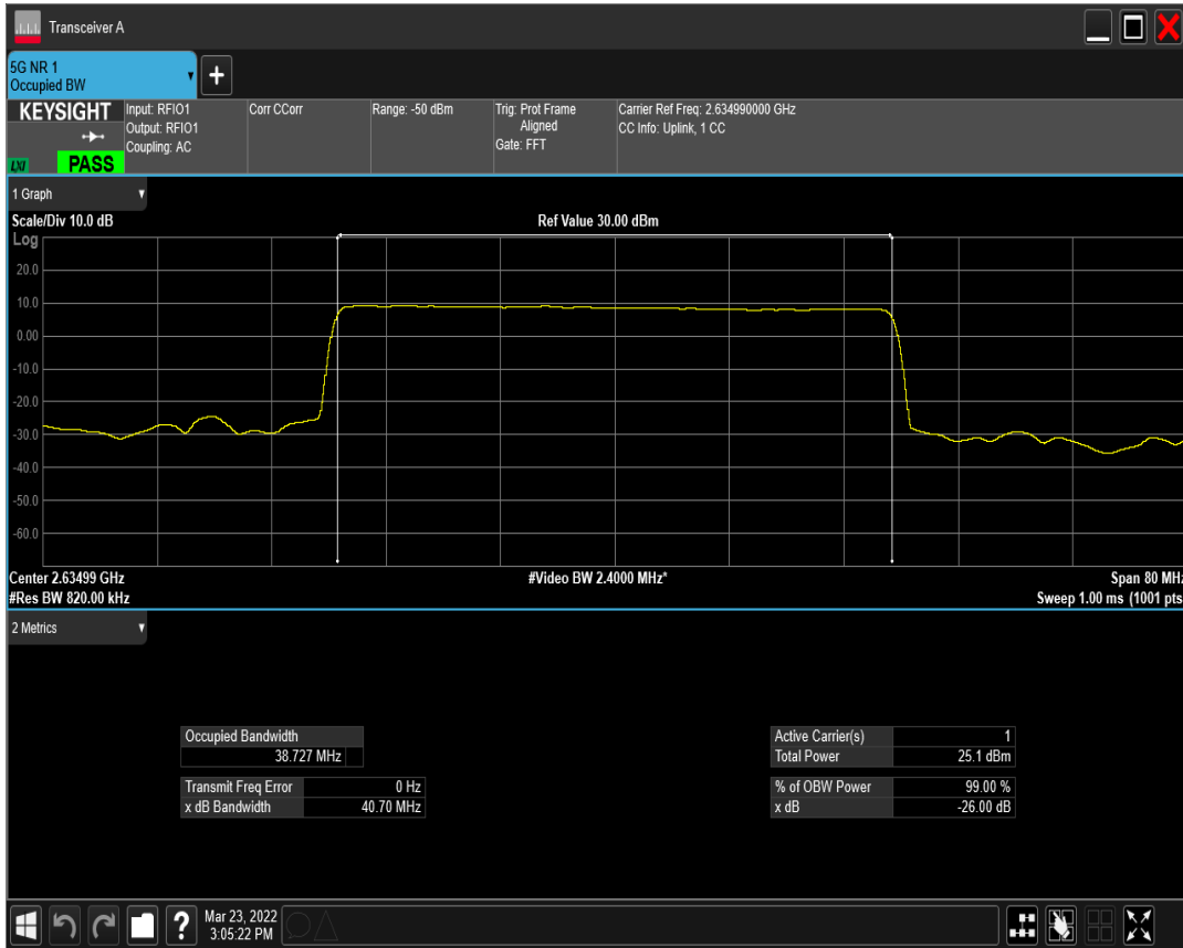
n41(2535-2655) SCS=15kHz DFT_QPSK BW=40MHz Channel=526998 RB=216@0
