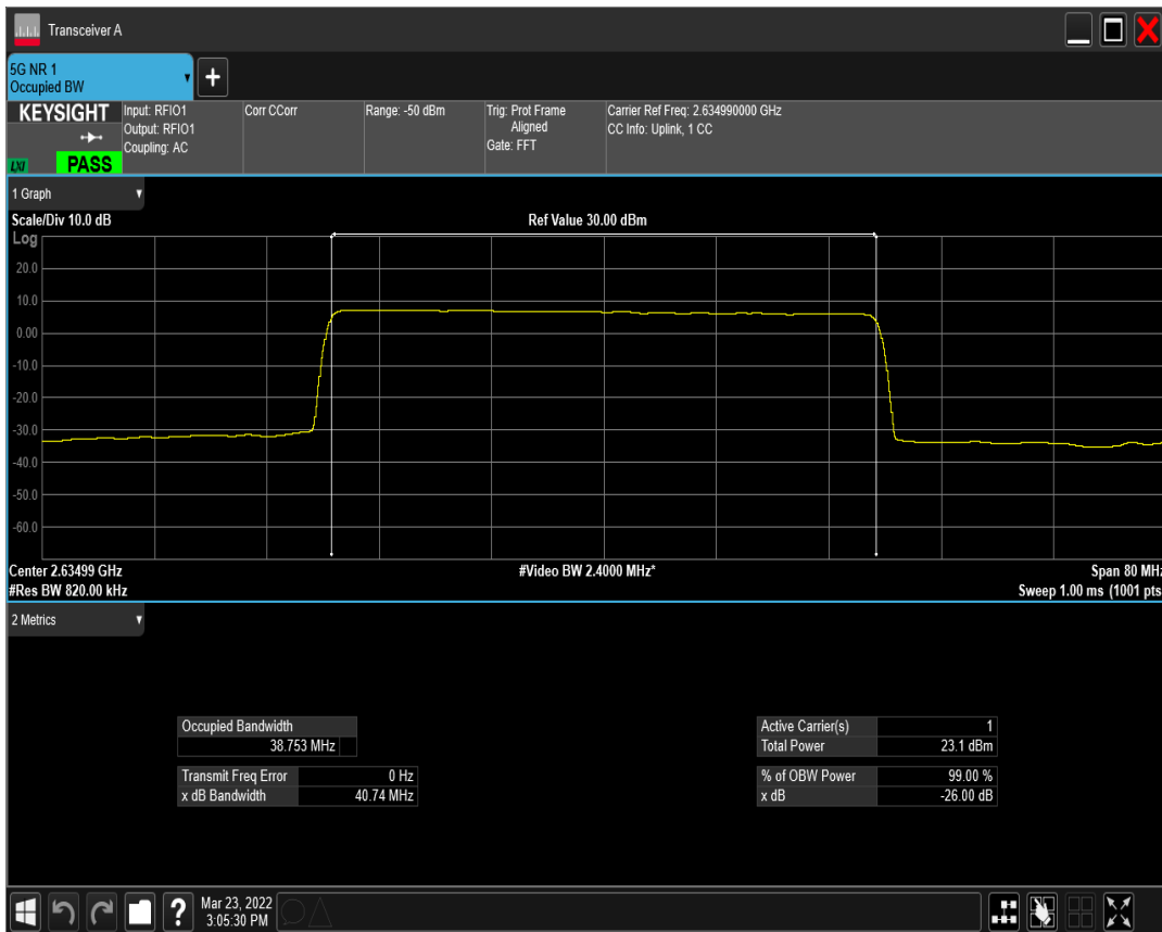
n41(2535-2655) SCS=15kHz DFT_QAM256 BW=40MHz Channel=526998 RB=216@0
