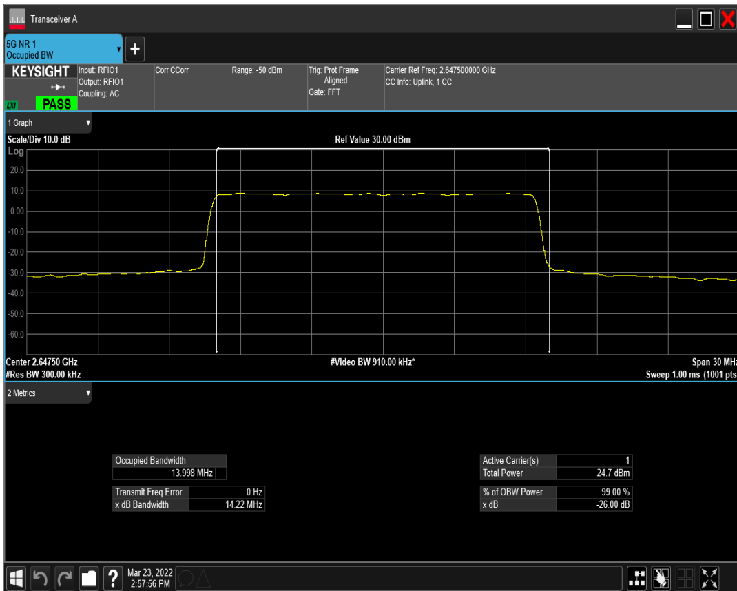
n41(2535-2655) SCS=15kHz DFT_QAM16 BW=15MHz Channel=529500 RB=75@0
