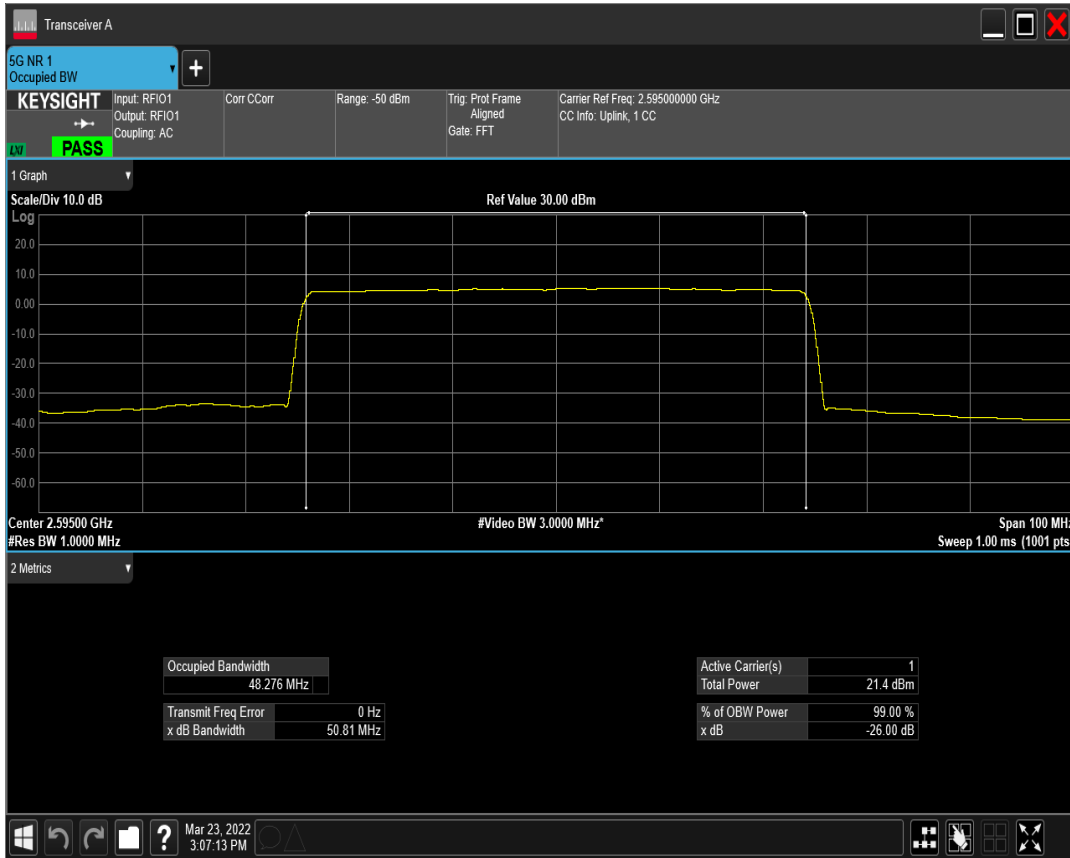
n41(2535-2655) SCS=15kHz CP_QPSK BW=50MHz Channel=519000 RB=270@0
