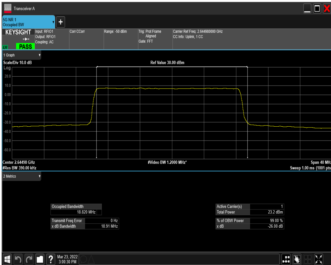
n41(2535-2655) SCS=15kHz DFT_QAM256 BW=20MHz Channel=528996 RB=100@0
