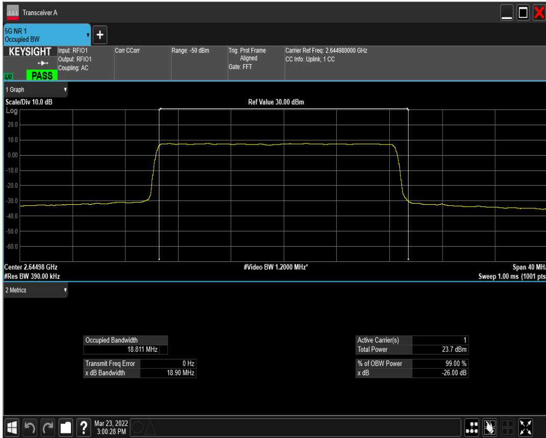
n41(2535-2655) SCS=15kHz DFT_QAM64 BW=20MHz Channel=528996 RB=100@0
