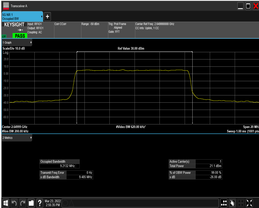
n41(2535-2655) SCS=15kHz CP_QPSK BW=10MHz Channel=529998 RB=52@0
