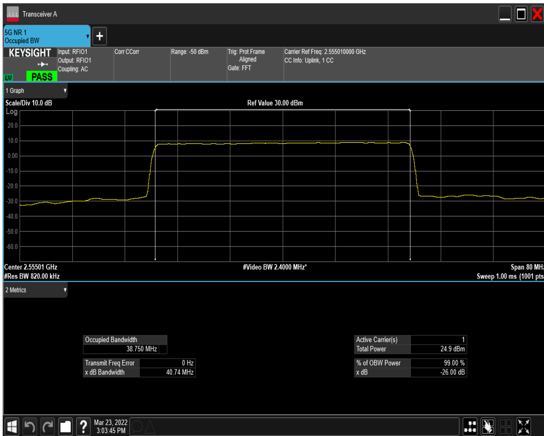
n41(2535-2655) SCS=15kHz DFT_QAM16 BW=40MHz Channel=511002 RB=216@0
