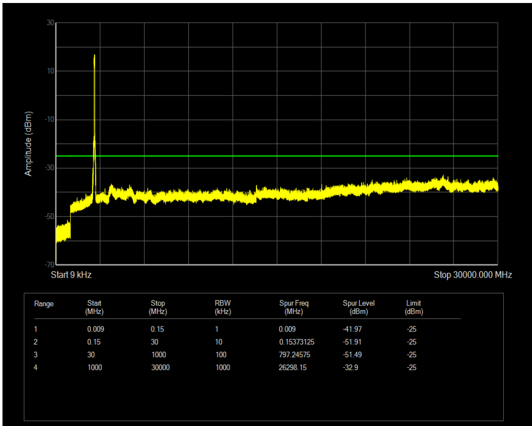
n41(2535-2655) SCS=15kHz DFT_QPSK BW=50MHz Channel=525996 RB=1@0
