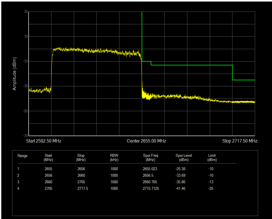
n41(2535-2655) SCS=15kHz DFT_QPSK BW=50MHz Channel=525996 RB=1@269
