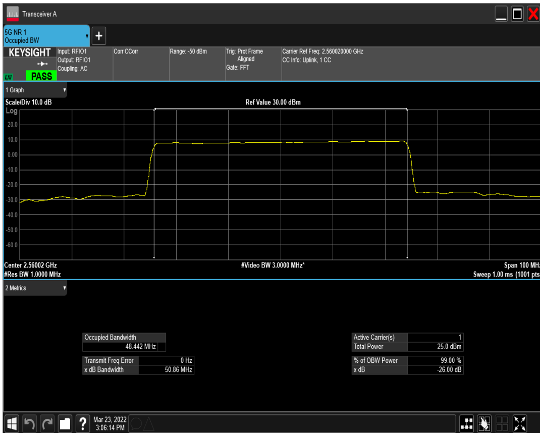
n41(2535-2655) SCS=15kHz DFT_QAM16 BW=50MHz Channel=512004 RB=270@0
