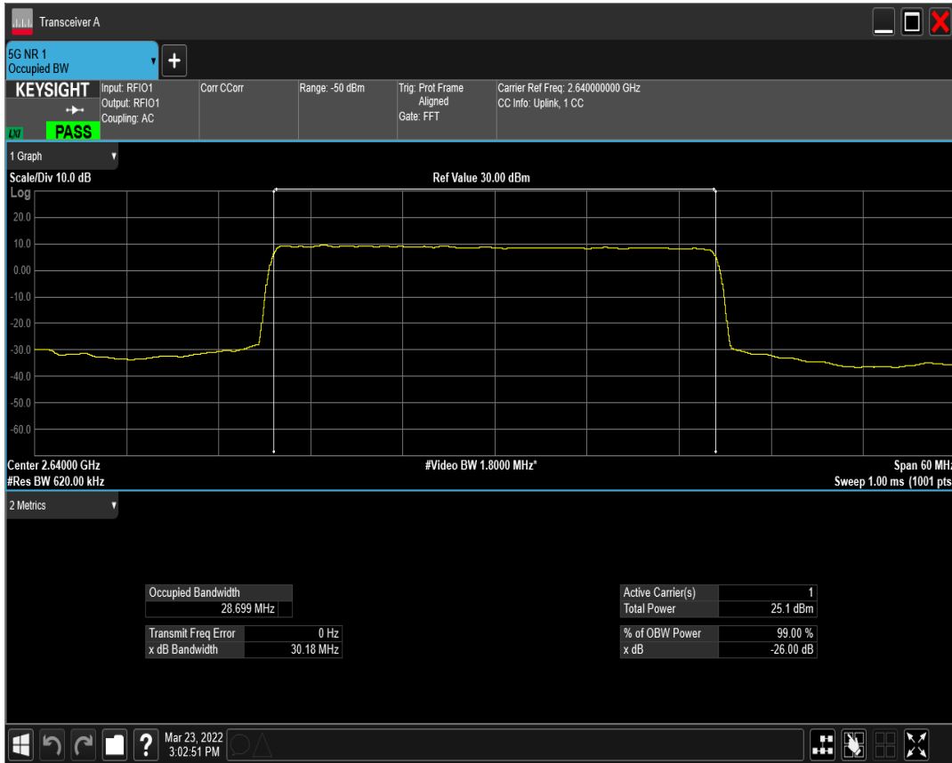
n41(2535-2655) SCS=15kHz DFT_QPSK BW=30MHz Channel=528000 RB=160@0
