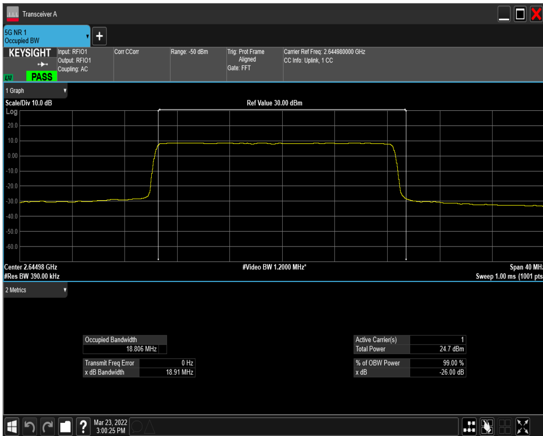
n41(2535-2655) SCS=15kHz DFT_QAM16 BW=20MHz Channel=528996 RB=100@0
