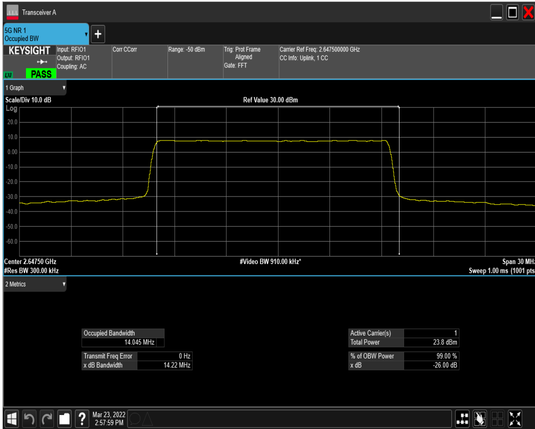
n41(2535-2655) SCS=15kHz DFT_QAM64 BW=15MHz Channel=529500 RB=75@0
