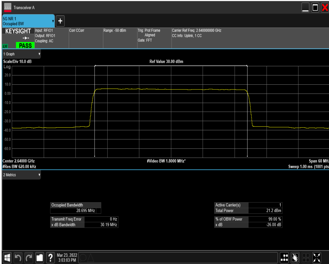
n41(2535-2655) SCS=15kHz CP_QPSK BW=30MHz Channel=528000 RB=160@0
