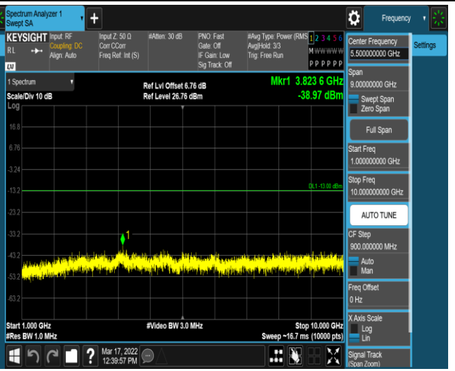
Band5-10MHz-QPSK-20600-1RB#0-Range2:1000~10000MHz
