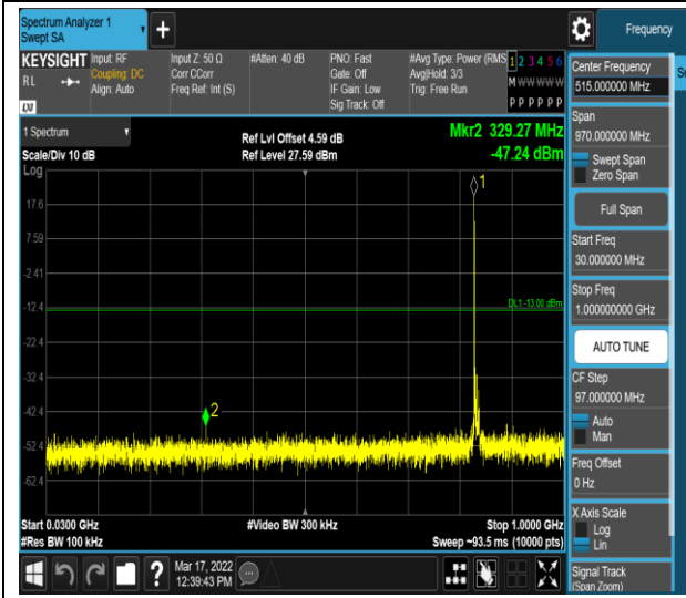
Band5-10MHz-QPSK-20600-1RB#0-Range1:30~1000MHz
