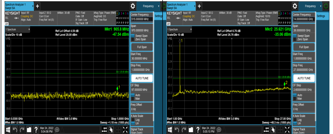
Band41-20MHz-16QAM-41140-1RB#0-Range1:30 ~1000MHz Band41-20MHz-16QAM-41140-1RB#0-Range2:1000~ 27000MHz
