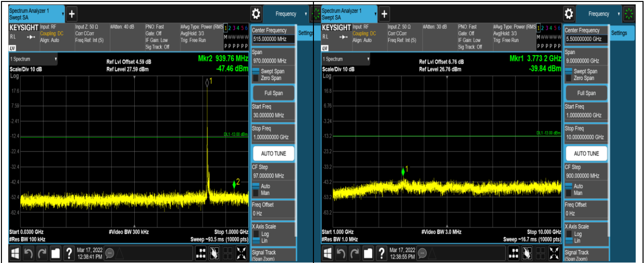
Band5-10MHz-QPSK-20525-1RB#0-Range1:30~1000MHz
