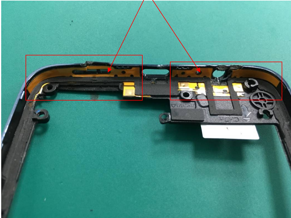
Aux Antenna
