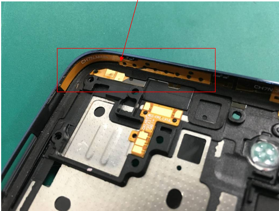
Main Antenna
