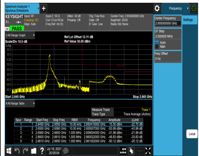
Band41-5MHz-QPSK-41215-25RB#0
