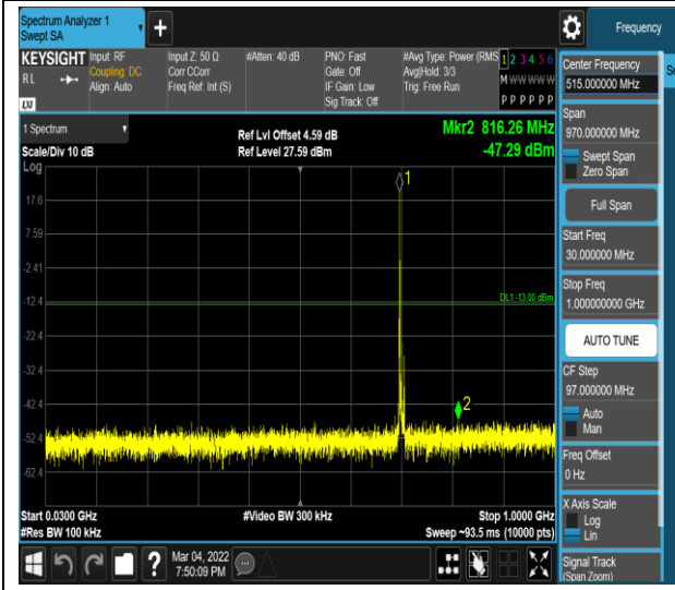
Band17-5MHz-16QAM-23755-1RB#0-Range1:30~1000MHz
