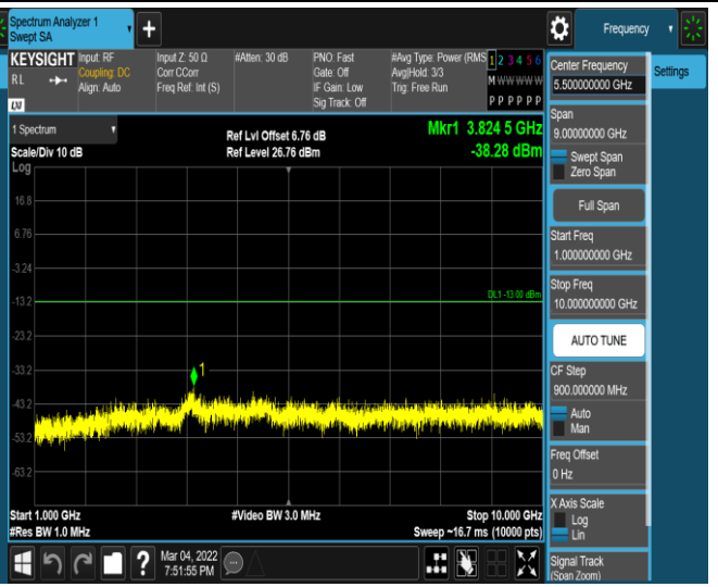
Band17-5MHz-16QAM-23755-1RB#0-Range2:1000~10000MHz
