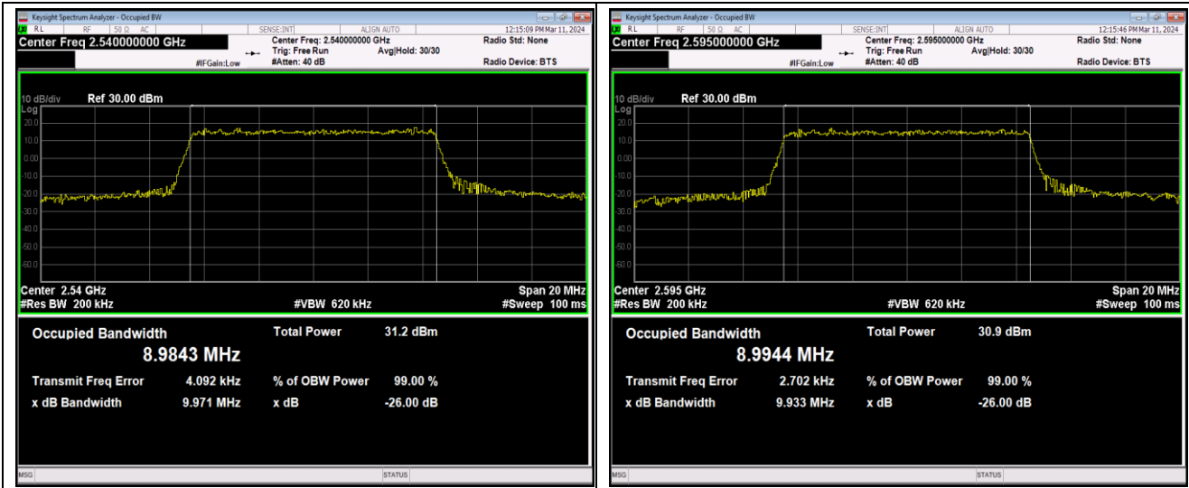
Band41-10MHz-16QAM-41190-50RB#0
