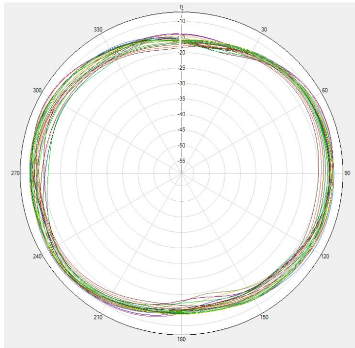
DCS1800/PCS1900/WCDMA B1/B2/B4/ LTE B1/B2/B3/B4 Theta=90deg
