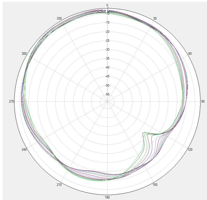
LTE B7/B38/41 Phi=90deg
