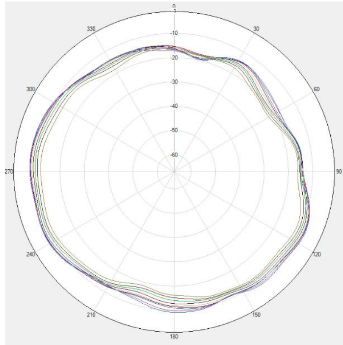
GSM900 / WCDMA B8 / LTE B8 Phi=90deg
