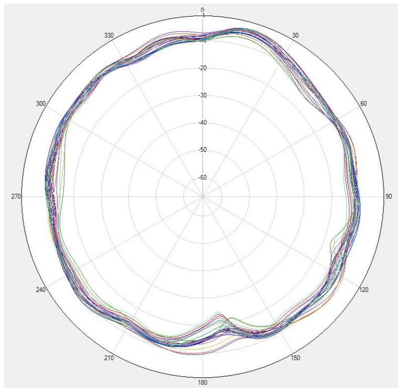
DCS1800/PCS1900/WCDMA B1/B2/B4/ LTE B1/B2/B3/B4 Phi=0deg
