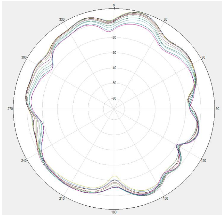
LTE B7/B38/41 Phi=90deg
