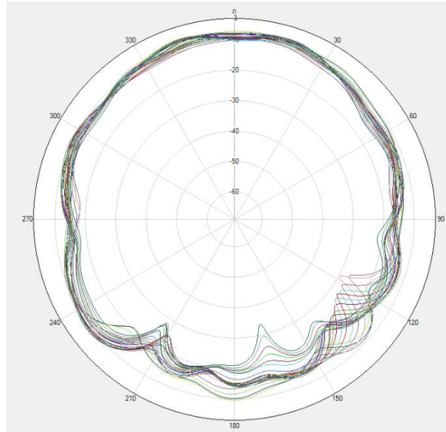
DCS1800/PCS1900/WCDMA B1/B2/B4/ LTE B1/B2/B3/B4 Phi=0deg
