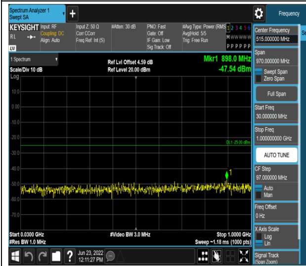
Band7-5MHz-16QAM-21425-1RB#0-Range1:30~1000MHz
