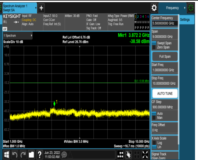
Band5-10MHz-QPSK-20525-1RB#0-Range2:1000~10000MHz
