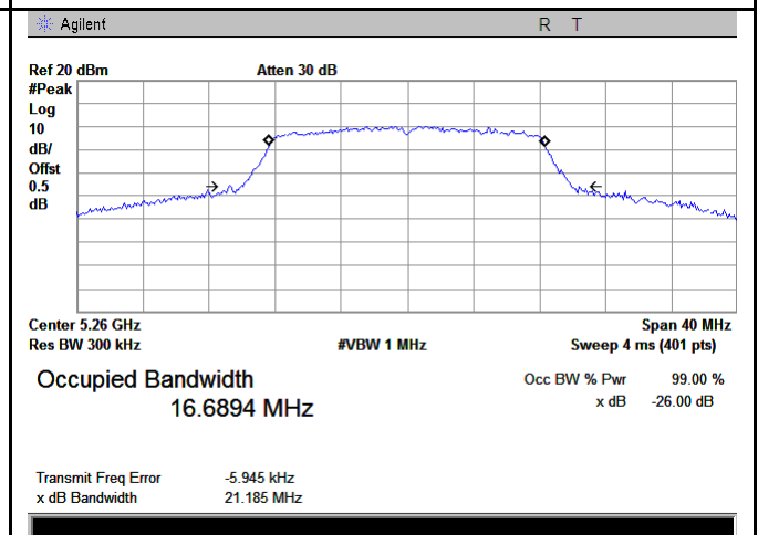
5250-5350MHz Bandwidth - Low CH 5260
