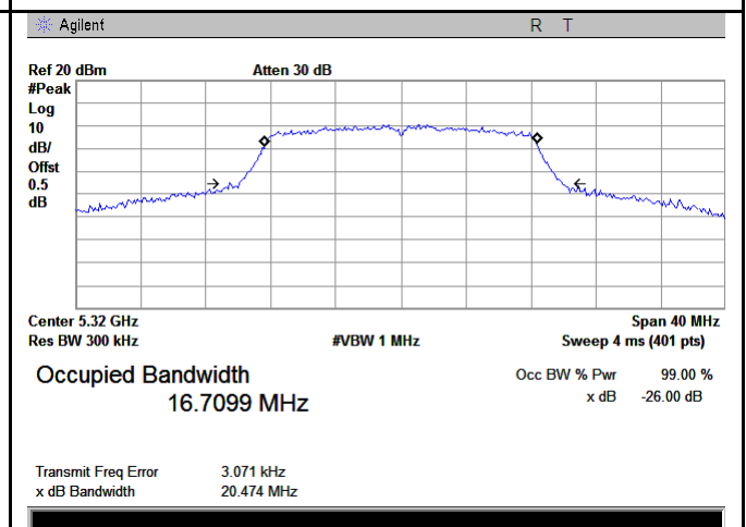
5250-5350MHz Bandwidth - High CH 5320
