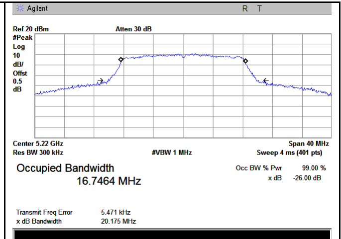
5150-5250MHz Bandwidth - Middle CH 5220
