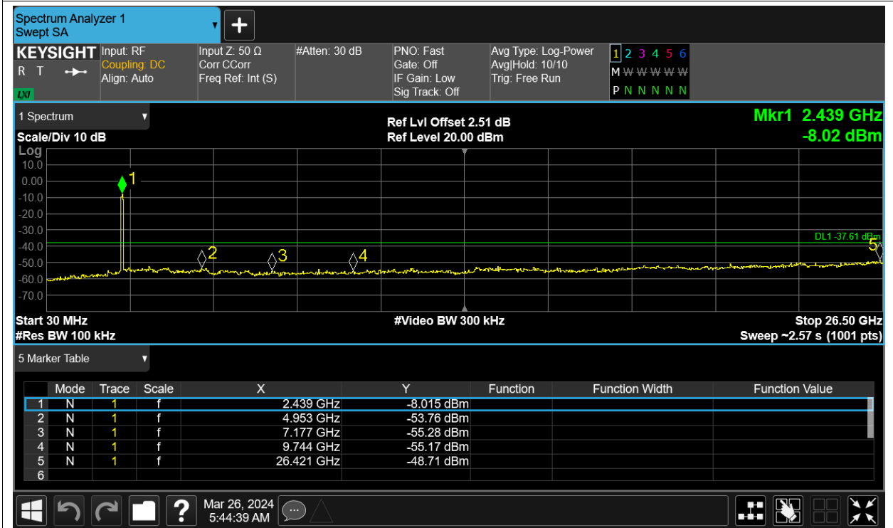
Tx. Spurious NVNT ax40 2452MHz Ant12 Ref
