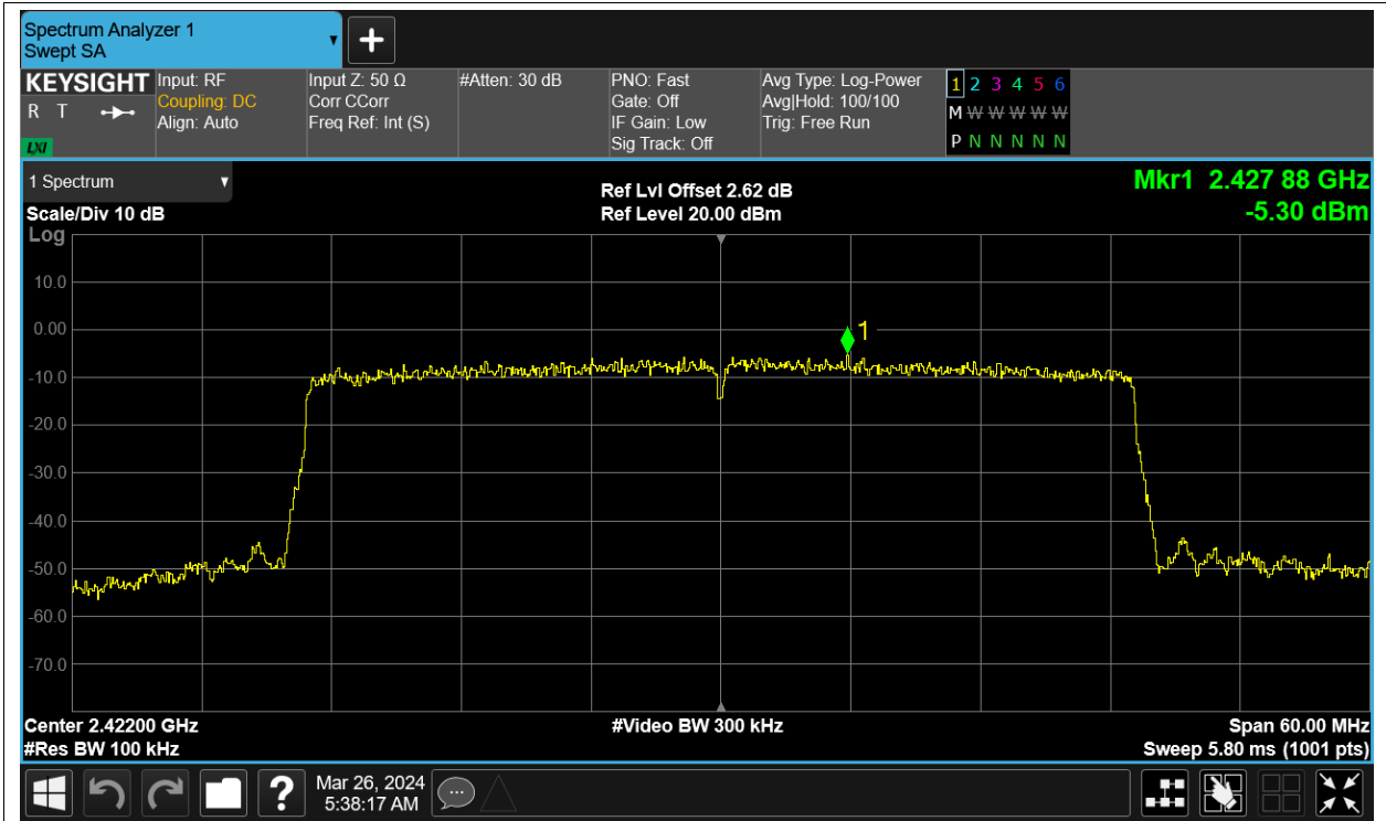
Tx. Spurious NVNT ax40 2422MHz Ant12 Emission
