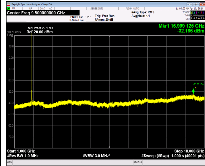
Band7_20MHz_QPSK_21350_1RB#0_1000~18000_1000~18000
