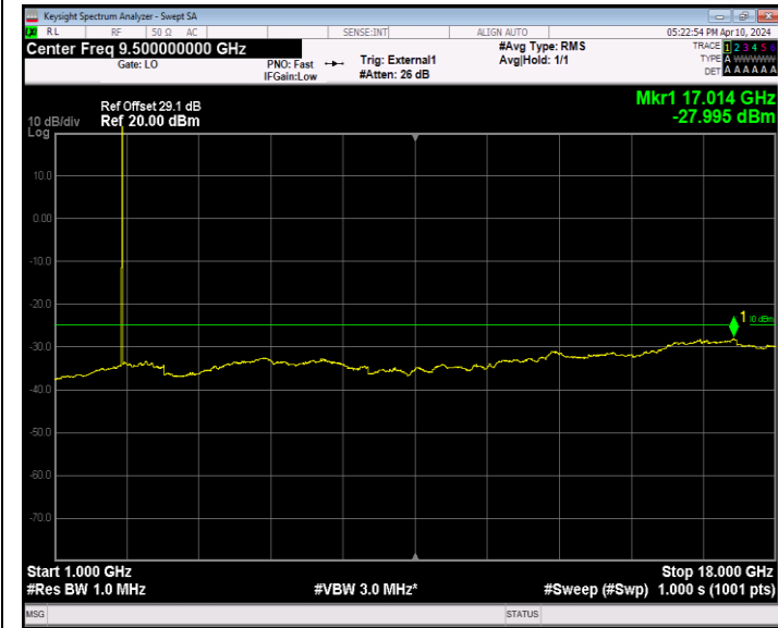
Band41_5MHz_QPSK_40620_1RB#0_1000~18000_1000~18000
