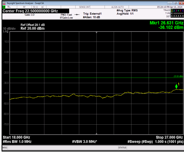
Band41_5MHz_16QAM_40620_1RB#0_18000~27000_18000~27000
