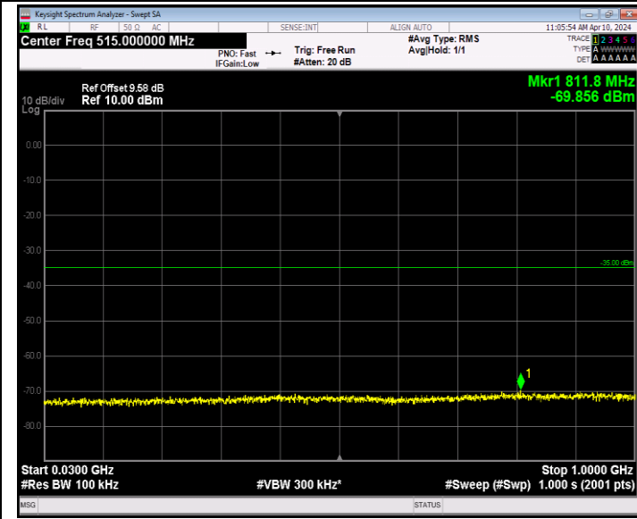
Band7_20MHz_16QAM_20850_1RB#0_30~1000_30~1000
