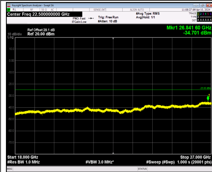
Band7_20MHz_64QAM_21100_1RB#0_18000~27000_18000~27000 000
