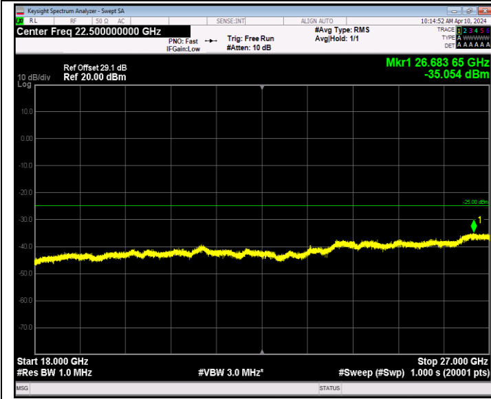
Band7_5MHz_64QAM_20775_1RB#0_18000~27000_18000~27000 00
