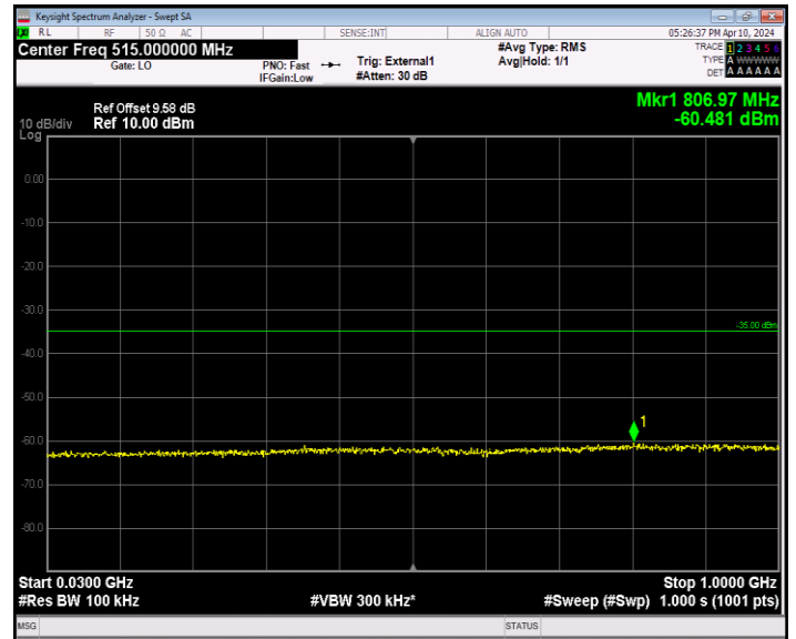
Band41_5MHz_16QAM_41565_1RB#0_30~1000_30~1000
