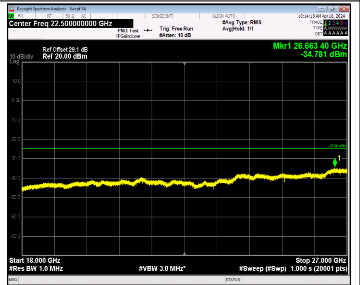
Band7_5MHz_16QAM_20775_1RB#0_18000~27000_18000~2700 00
