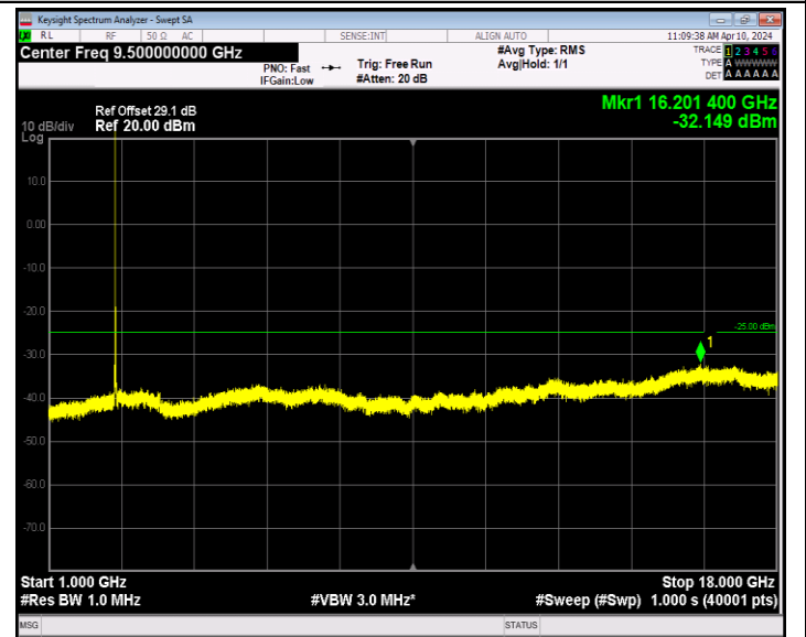
Band7_20MHz_16QAM_21350_1RB#0_1000~18000_1000~1800 0
