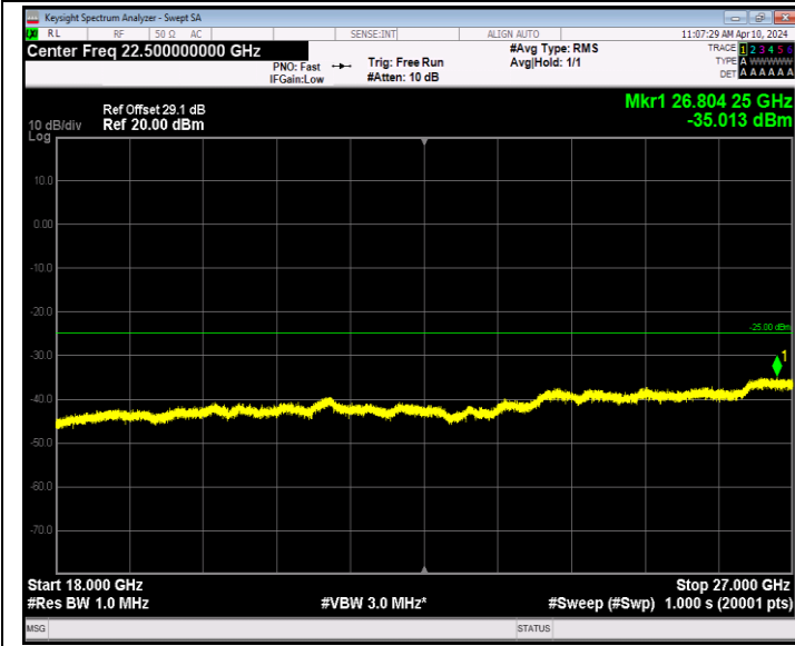
Band7_20MHz_QPSK_21100_1RB#0_18000~27000_18000~27000 00
