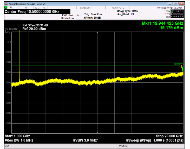
Band2_20MHz_64QAM_19100_1RB#0_1000~20000_1000~2000 0
