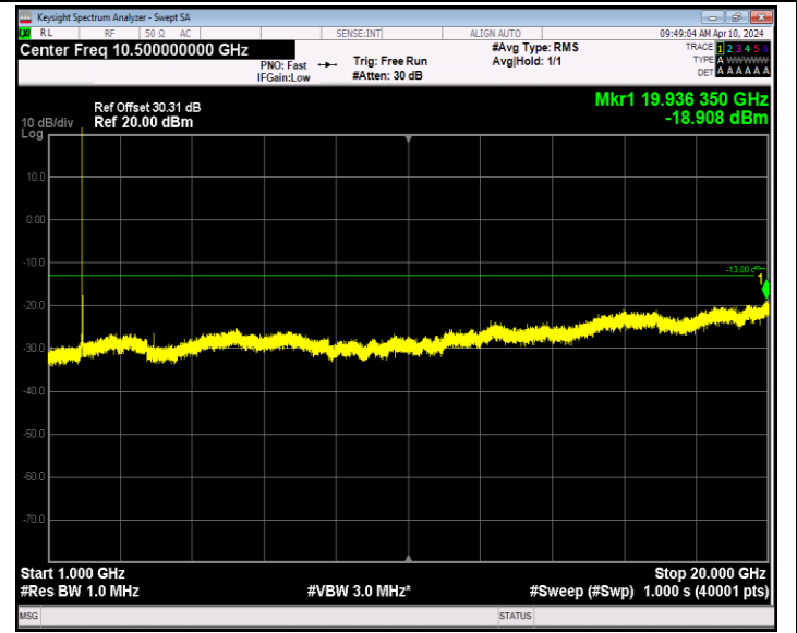
Band2_20MHz_16QAM_19100_1RB#0_1000~20000_1000~2000
