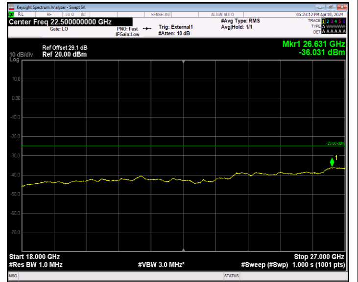
Band41_5MHz_QPSK_40620_1RB#0_18000~27000_18000~27000 00
