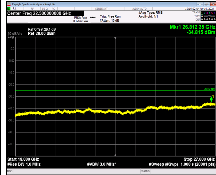
Band7_5MHz_16QAM_21100_1RB#0_18000~27000_18000~270
