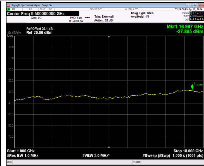
Band41_5MHz_64QAM_40620_1RB#0_1000~18000_1000~1800 0
