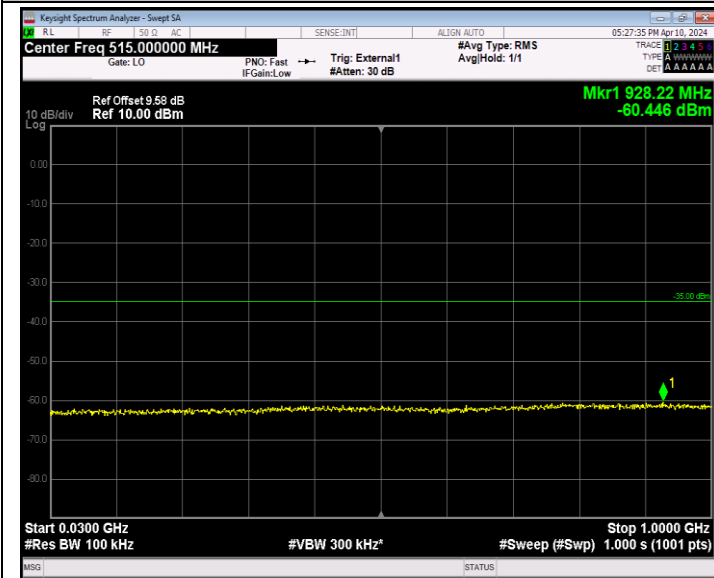
Band41_5MHz_64QAM_41565_1RB#0_30~1000_30~1000 0
