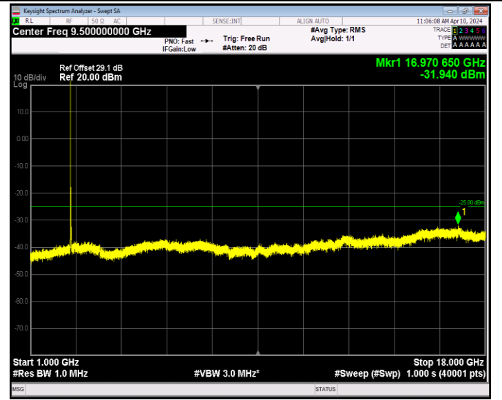
Band7_20MHz_16QAM_20850_1RB#0_1000~18000_1000~1800 0
