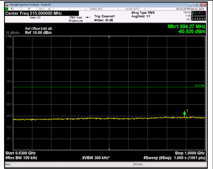
Band41_5MHz_QPSK_40620_1RB#0_30~1000_30~1000
