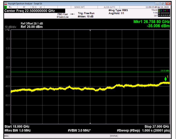
Band7_20MHz_QPSK_21350_1RB#0_18000~27000_18000~27000 00
