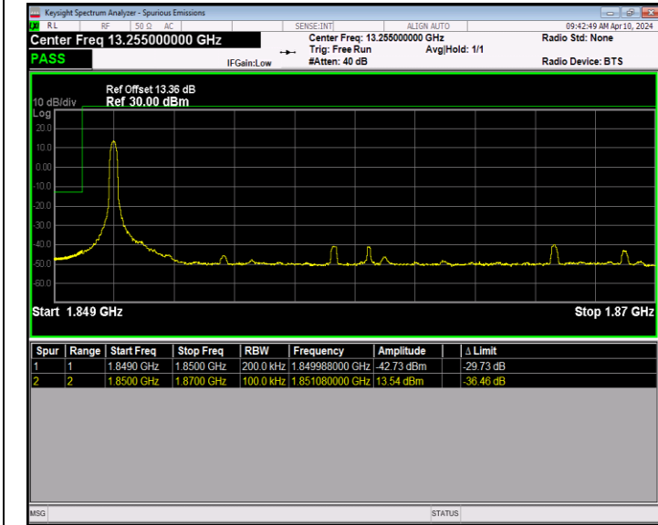
Band2_20MHz_64QAM_18700_1RB#0
