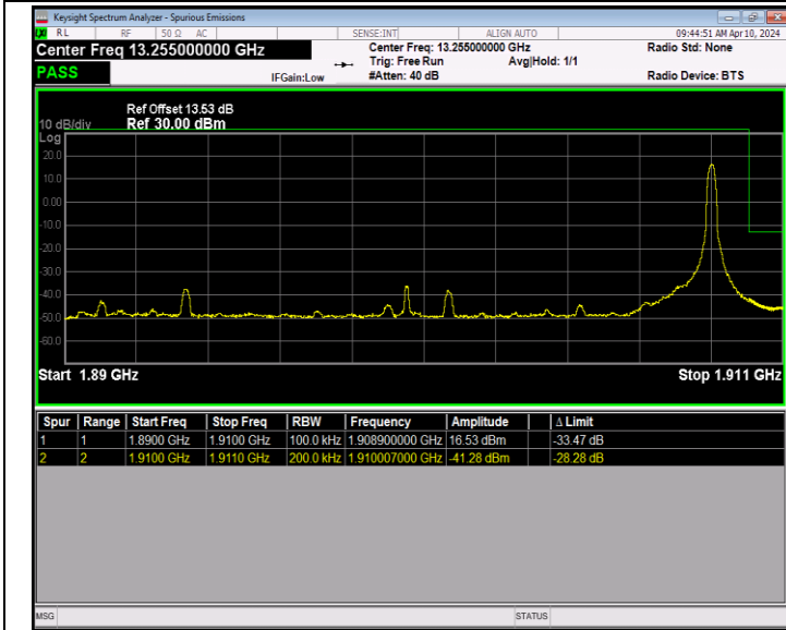
Band2_20MHz_QPSK_19100_1RB#99
