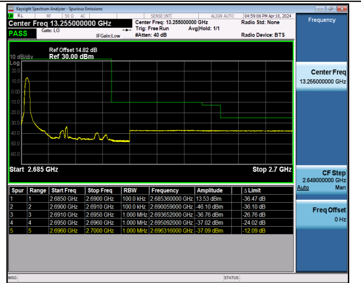
Band41_5MHz_64QAM_41565_1RB#0
