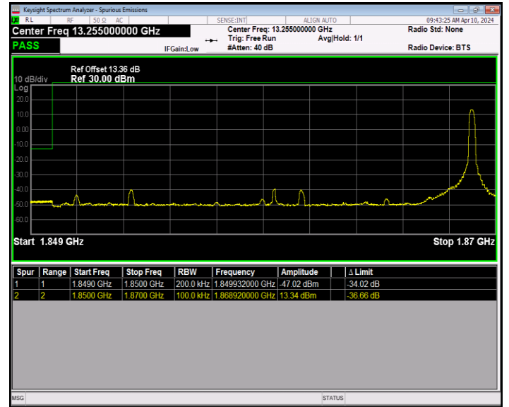
Band2_20MHz_64QAM_18700_1RB#99
