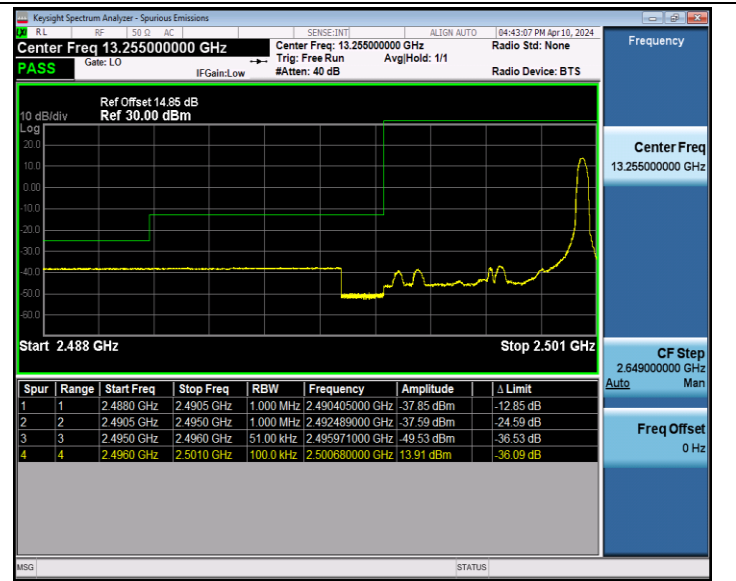
Band41_5MHz_64QAM_39675_1RB#24
