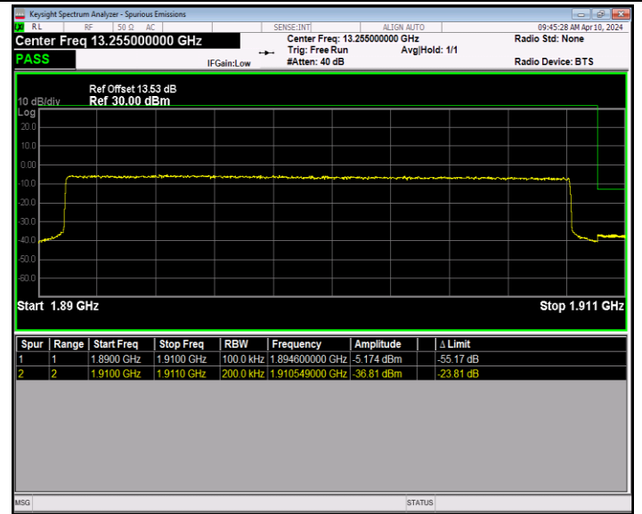
Band2_20MHz_QPSK_19100_100RB#0
