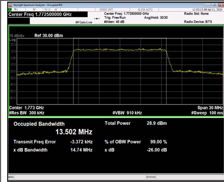
Band66-15MHz-QPSK-132597-75RB#0-PASS
