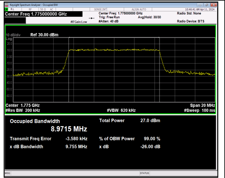
Band66-10MHz-64QAM-132622-50RB#0-PASS
