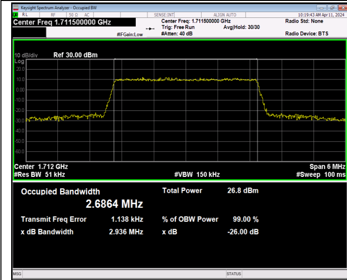
Band66-3MHz-16QAM-131987-15RB#0-PASS
