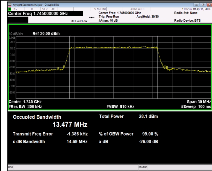
Band66-15MHz-16QAM-132322-75RB#0-PASS
