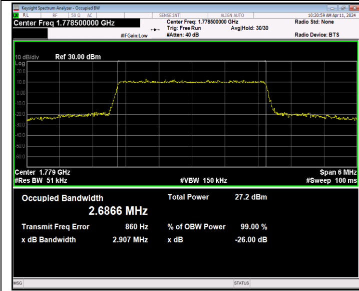
Band66-3MHz-16QAM-132657-15RB#0-PASS
