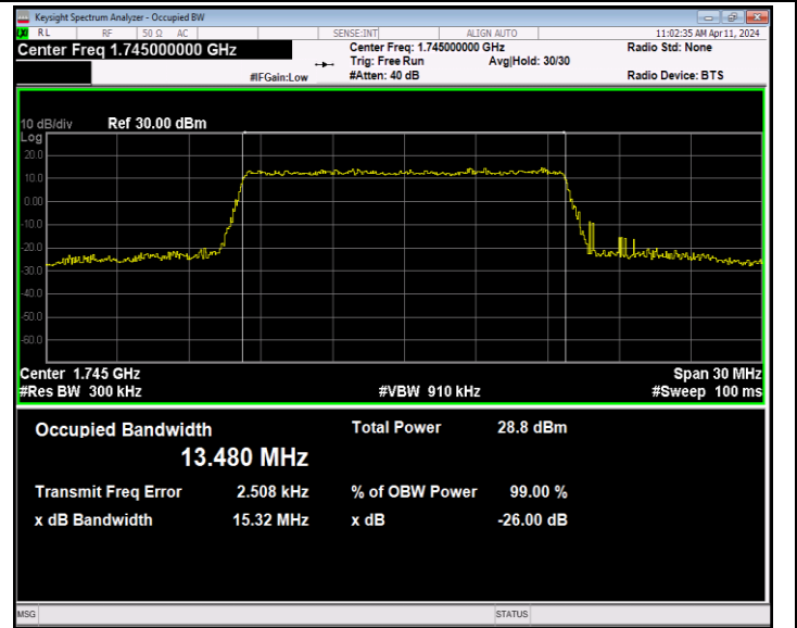
Band66-15MHz-QPSK-132322-75RB#0-PASS
