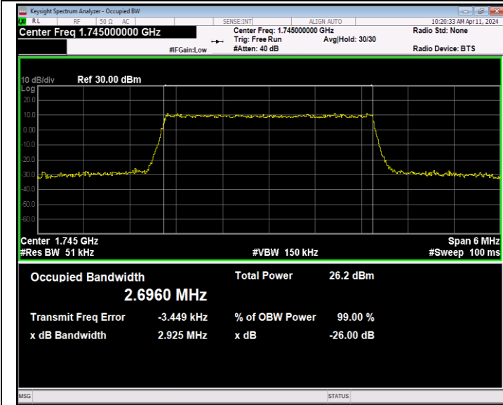
Band66-3MHz-64QAM-132322-15RB#0-PASS
